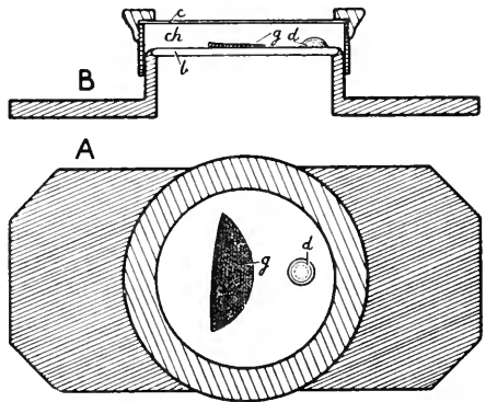
FIG. 14.—A compressor cell used for observing the development and discharge of spores on the hymenium of Hymenomyces. A, viewed from above; g, a gill of an Agaric; d, a water-drop. B, vertical section; b, the glass base of the cell; c, the cover-glass; ch, the moist chamber; g, a gill; d, a water-drop. The frame-work of the cell was made of brass. The chamber, ch, can be made larger or smaller by raising or lowering the cap of the cell. Actual size.
