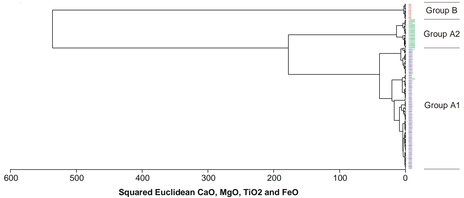
Figure 5.21: Dendrogram using minimum variance to group the EPMA analyses of the SILK layers. The marks on the right hand side identify the analyses: red = Group B; green = Group A2; blue = Group A1.
