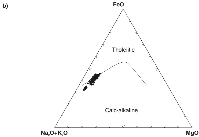
Figure 5.16: Graphs to show that: a) all of the analysed SILK layers are silicic, based on recommendations of Le Maitre (1989). b) The SILK layers can clearly be split into two groups with the smaller group being wholly calc-alkaline and the larger group straddling the tholeiitic/calc-alkaline boundary, based on Irvine and Baragar (1971).
