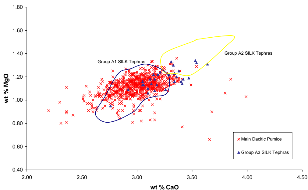
Figure 5.34: Graph to show the differences between the SILK Group A1, A2 and A3 tephra layers and the correlation of the A1 SILK layers with the main ocean-rafted pumice. The blue field is defined by 153 analyses of the Group A1 tephra (3 extreme analyses are excluded) and the yellow field is defined by 40 analyses of the Group A2 tephra.
