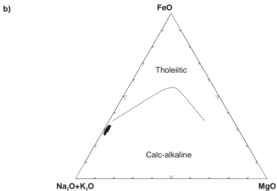
Figure 5.29: Graphs to show that: a) all of the analysed Katla pumice are silicic, based on recommendations of Le Maitre (1989). b) the silicic pumice is calc-alkaline, based on Irvine and Baragar (1971).
