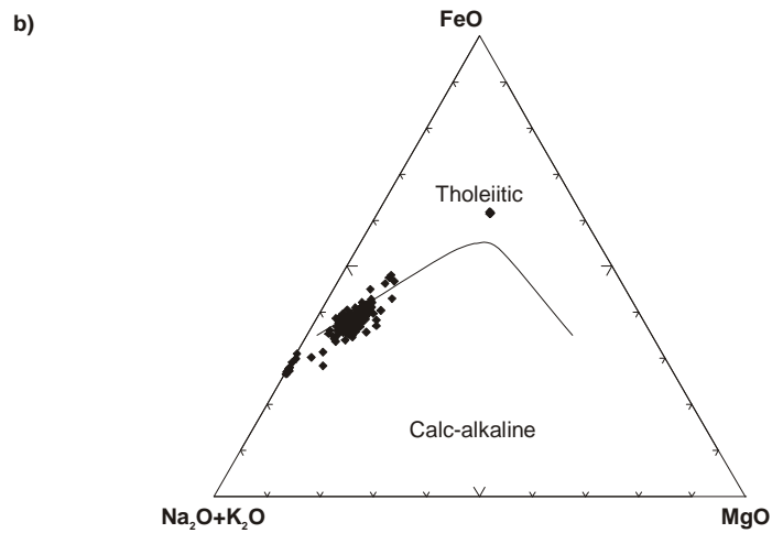
Figure 3.18: Graphs to show that: a) most of the pumice pieces analysed are silicic, with some basic analyses and can be split into at least three distinct groups (based on recommendations of Le Maitre, 1989). b) The majority of the pumice is calc-alkaline, with some tholeiitic analyses. At least three major groups can be identified (based on Irvine and Baragar, 1971). The term acidic has been replaced by silicic in this thesis, as recommended by Dugmore et al. (1995), in order to avoid confusion with volcanic aerosols.
