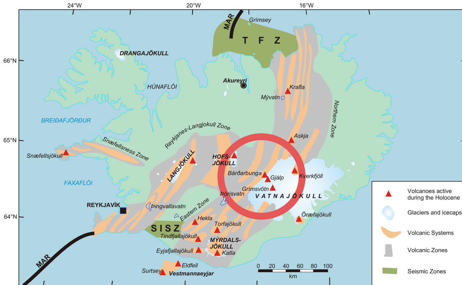
Figure 5.1: Map to show the location of Icelandic volcanic zones, volcanic systems, recently active volcanoes, fracture zones and mantle plume. The position of the mantle plume is indicated by the red circle. MAR = Mid-Atlantic Ridge, SISZ = South Iceland Seismic Zone, TFZ = Tjörnes Fracture Zone. Based on information in Jakobsson (1979), Wolfe (1997), Larsen et al. (1998).
