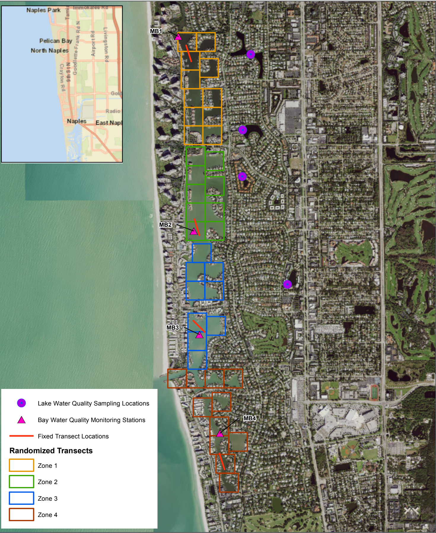
Figure 2-1. Water Quality and Biological Monitoring Locations in Moorings Bay City of Naples, Natural Resources Division Collier County, Florida
