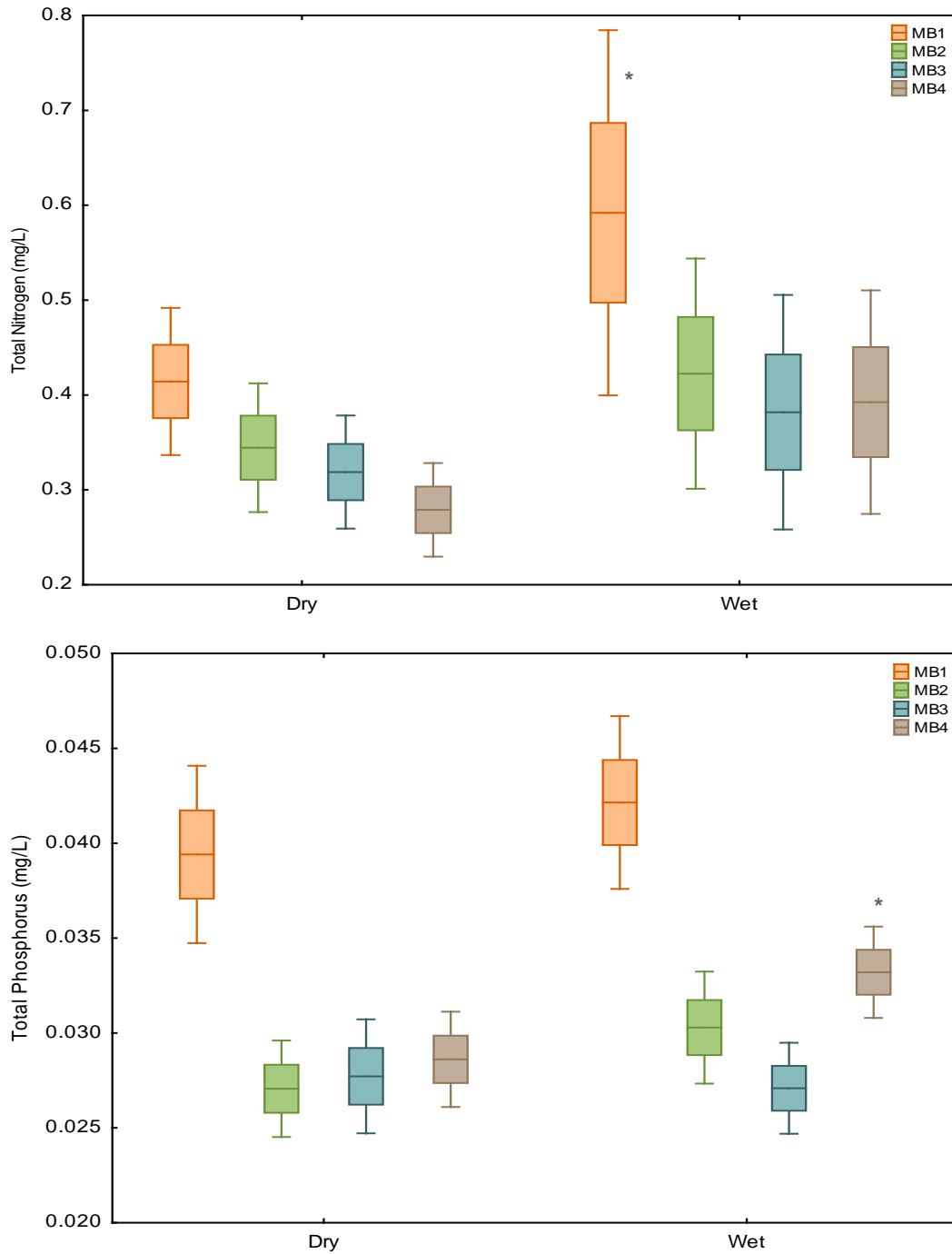
Figure 4-12. Seasonal total nitrogen and total phosphorus by station in Moorings Bay, October 2008–December 2015 (mean, \pm 1 SE, and \pm 0.95 confidence interval). Within each plot, asterisks indicate stations with a significant difference between seasons (two-tailed t-test).
