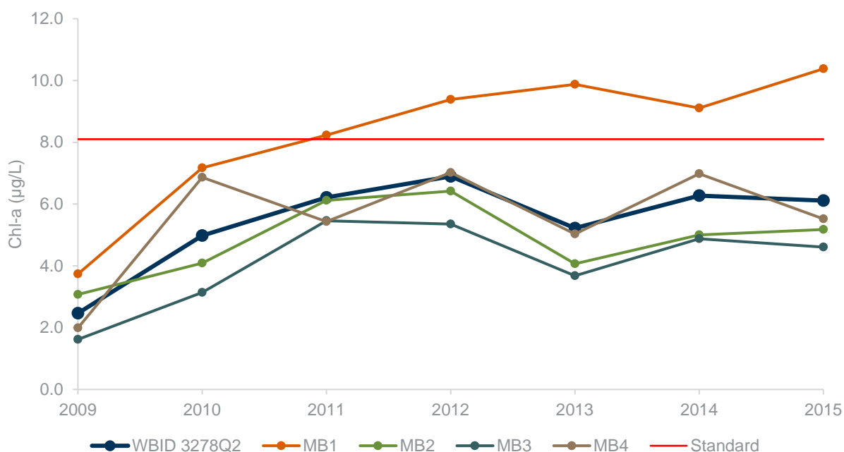
Figure 4-15. Chlorophyll-a concentrations in Moorings Bay and by sampling station with the NNC threshold, October 2008–December 2015.
