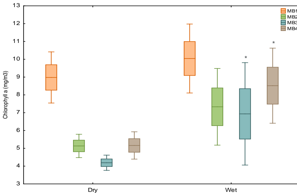
Figure 4-18. Seasonal chlorophyll- a concentrations by station in Moorings Bay, October 2008–December 2015 (mean, \pm 1\text{SE} , and \pm 0.95 confidence interval). Within each plot, asterisks indicate stations with a significant difference between seasons (two-tailed t-test).
