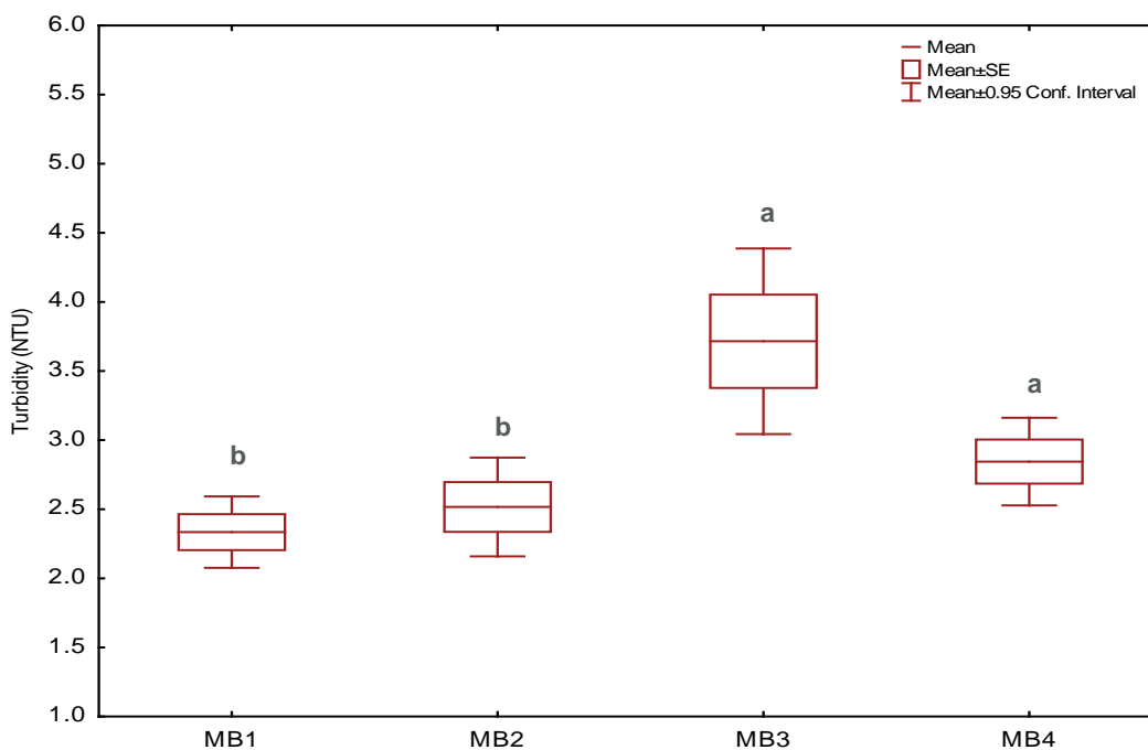
Figure 5-2. Turbidity concentrations by station in Moorings Bay, October 2008–December 2015. Within each plot, letters next to the boxes designate statistically significant different groups (paired t-test, two-tailed, p < 0.05 ).
