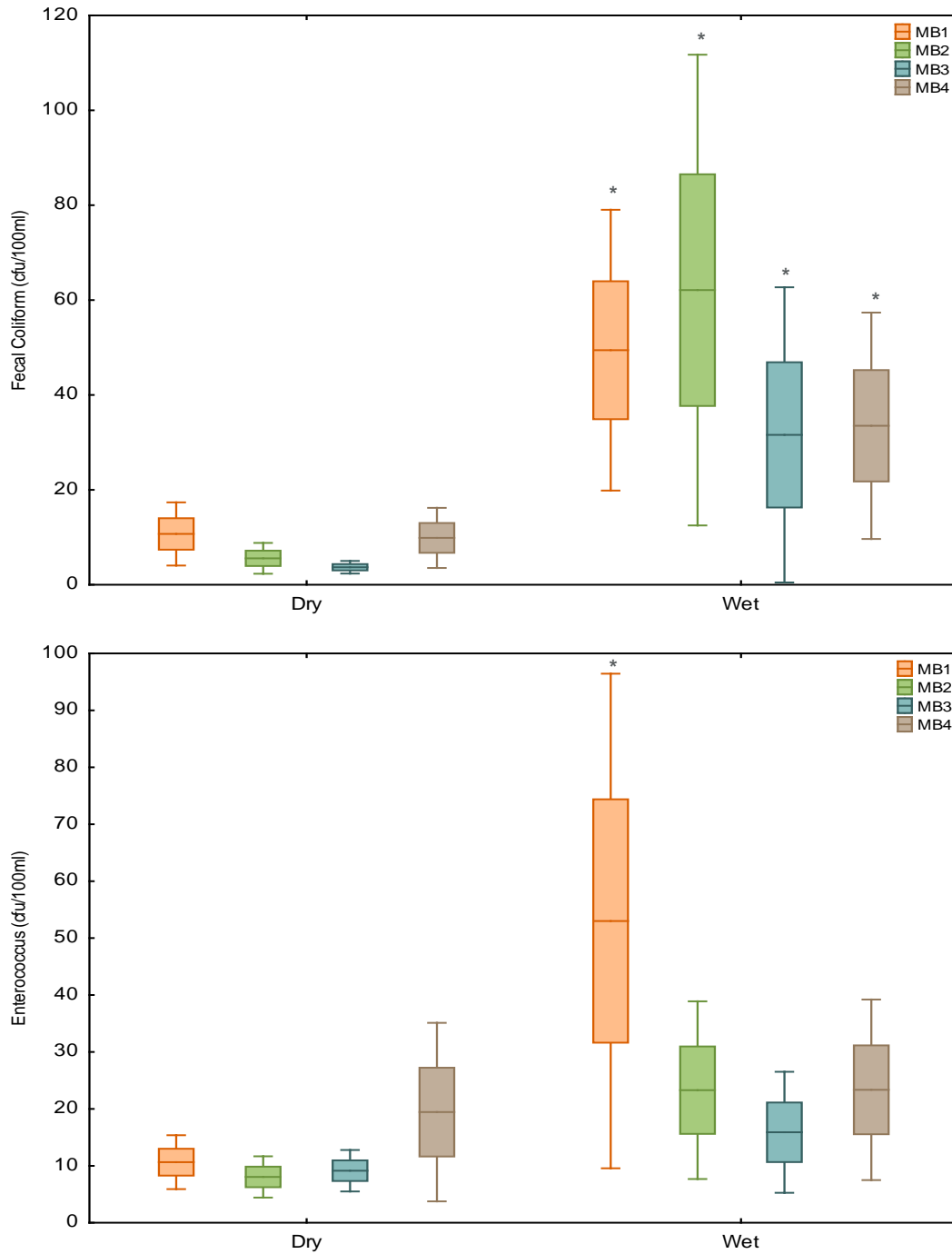
Figure 4-27. Fecal coliform and Enterococci concentrations by station in Moorings Bay, October 2008–December 2015 (mean, \pm 1 SE, and \pm 0.95 confidence interval). Within each plot, asterisks indicate stations with a significant difference between seasons (paired t-test).
