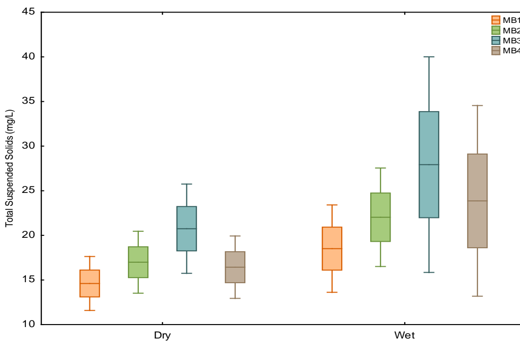
Figure 5-7. Seasonal total suspended solids concentrations by station in Moorings Bay, October 2008–December 2015 (mean, \pm 1 SE, and \pm 0.95 confidence interval). Within each plot, asterisks indicate stations with a significant difference between seasons (two-tailed t-test).
