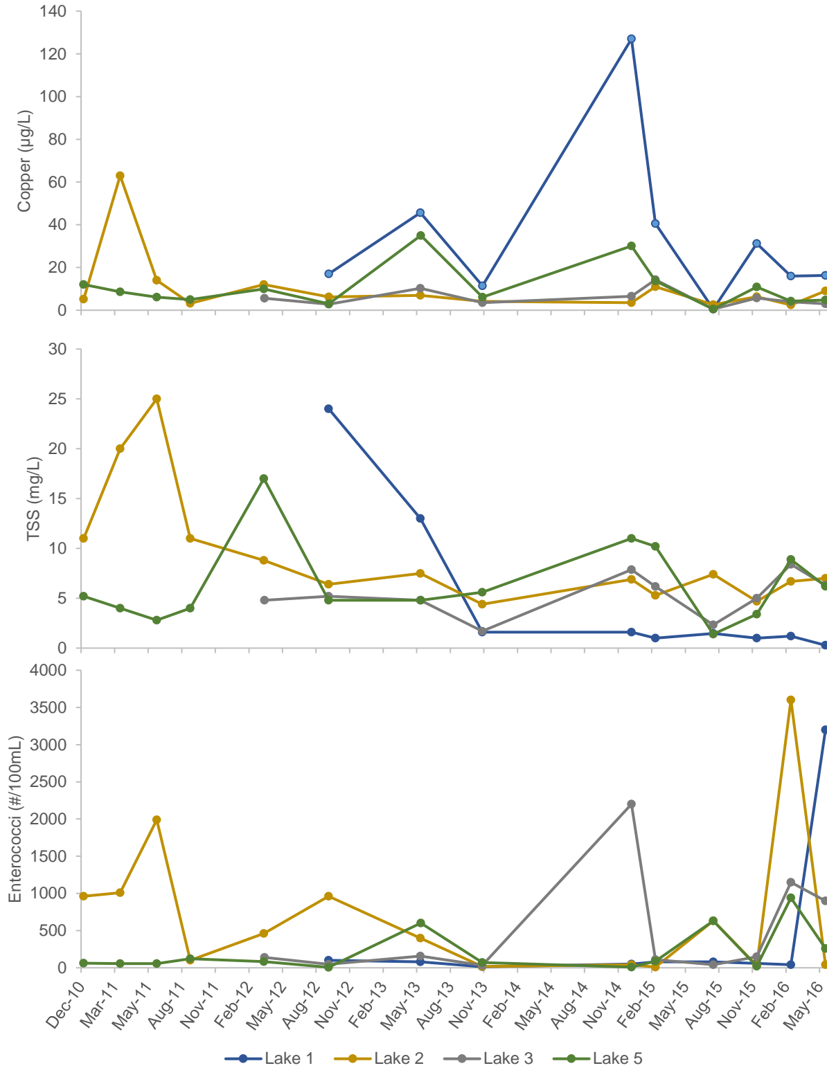
Figure 3-4. Copper, TSS, and Enterococci concentrations in stormwater lakes that discharge to Moorings Bay, December 2010–May 2016.
