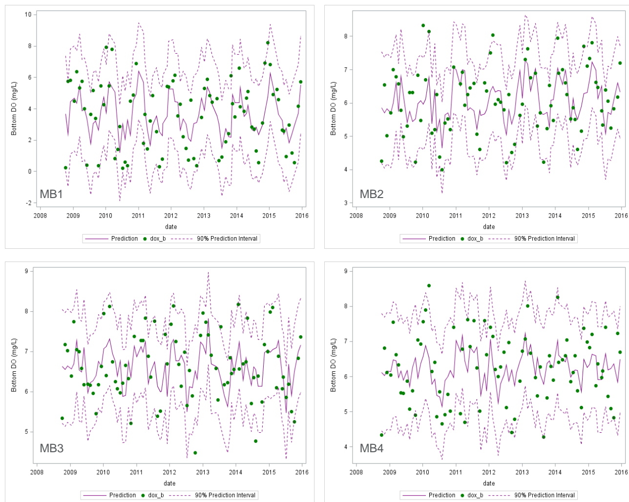
Figure 4-24. Results of AEM time series models of monthly bottom dissolved oxygen in Moorings Bay, 2008–2015, including observed, predicted, and 90 percent prediction intervals.
