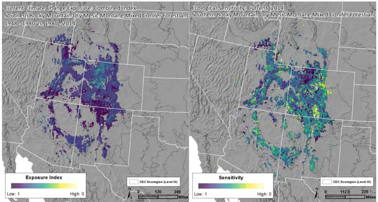
Figure 26. Climate exposure as of 2014 (left) and overall sensitivity (right) for Southern Rocky Mountain Dry-Mesic Montane Mixed Conifer Forest and Woodland. The results have been summarized and are displayed in 100km 2 hexagons. In both maps, the dark purple indicates low exposure or low sensitivity, with progressively higher exposure or sensitivity (and hence higher vulnerability) indicated by the bright green to yellow.
