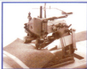
SISAL/BERBER BINDER 81200-S The heavy duty binder that binds top and bottom in one operation. Independent heavy duty front & back pullers.
