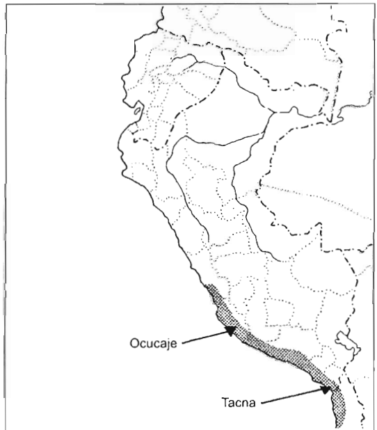
Map. Distribution of Slender-billed Finch Xenospingus concolor (from Ridgely & Tudor 5 ), identifying the study areas.
