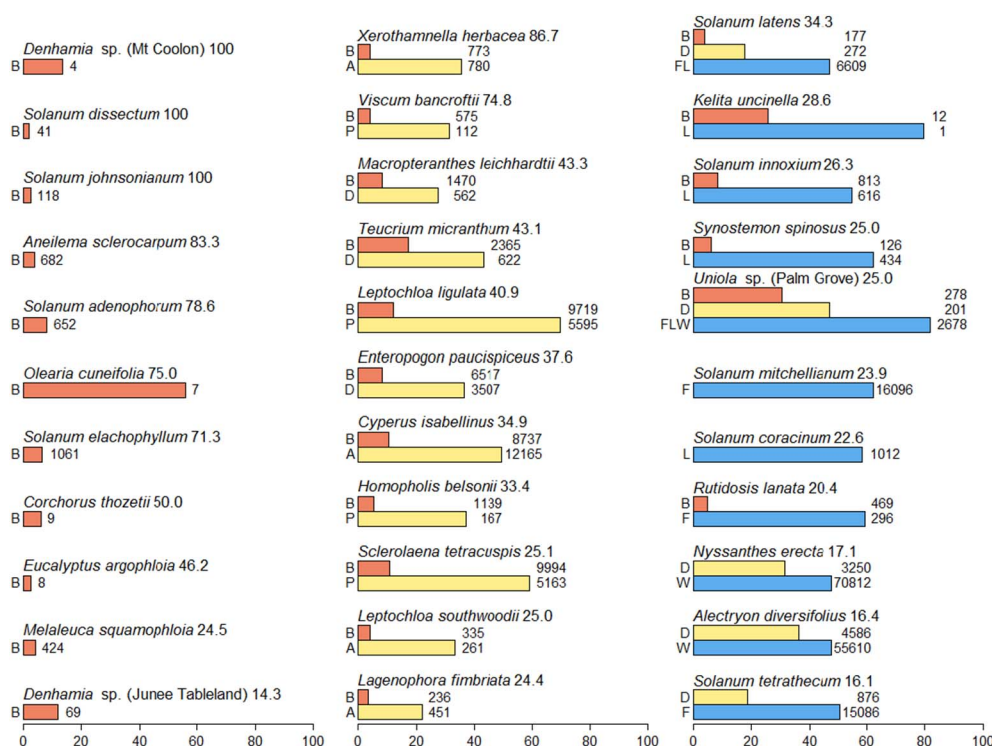
Fig. 2. The percentage habitat remaining for ten species with the highest threat exposure score (Appendix 4) in three groups: species confined to brigalow habitat (left-hand column), species also associated with other heavily cleared habitats (middle column); species also associated with less heavily cleared habitats (right-hand column). These three categories are indicated by the colours: brigalow (brown); other heavily cleared habitats (mustard); less heavily cleared habitats (blue), and the letter codes: B, brigalow; A, alluvial woodland; P, poplar box woodland; D, dry rainforest; F, eucalypt forest; W, eucalypt woodland; L, lancewood forest. The threat exposure score is indicated next to the name of the species. (For interpretation of the references to colour in this figure legend, the reader is referred to the web version of this article.)
