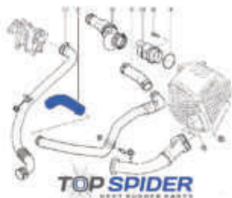
Renault Laguna II 1.9 DCI 2001-2005 intercooler turbo hose
