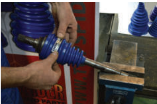
7. USE THE GREASE AND PUT THE CLAMPS ON / Staviti grafitnu mast i montirati šelne
