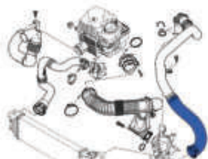
Renault Master II 2.3 DCI intercooler turbo hose
