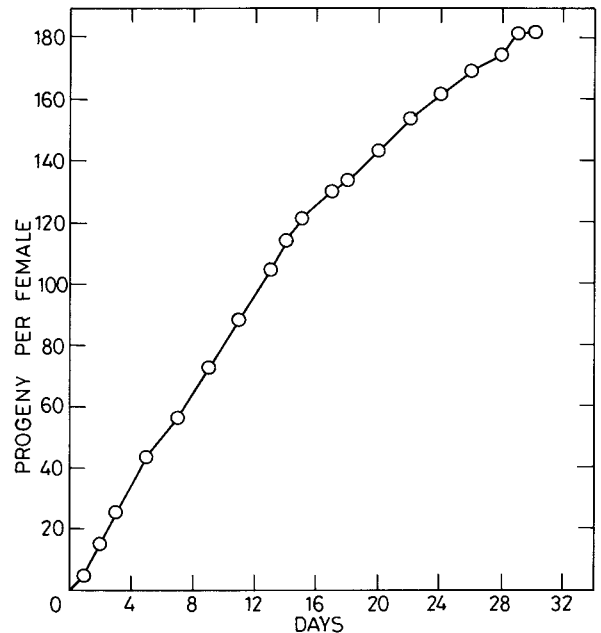
Fig. 30. Chartocerus subaeneus , cumulative progeny production at 28°C, >50% RH (initial n = 6).
