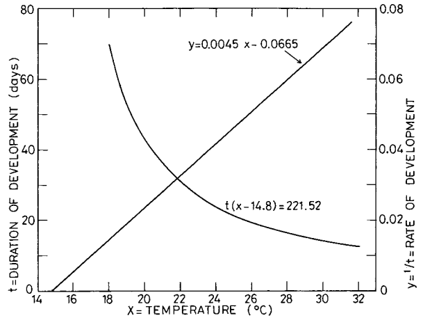
Fig. 33. Chartocerus subaeneus , effect of temperature on rate and duration of development.
