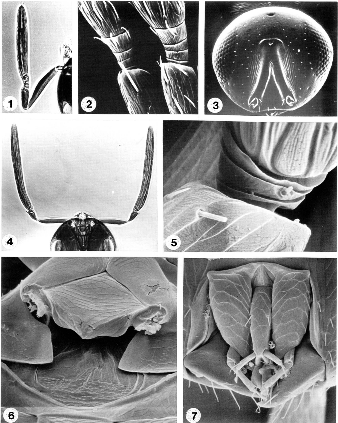
Figs. 1-7. Chartocerus subaeneus . 1, Female antenna. 2, Female antennae: pedicel, funicle and base of club (SEM). 3, Head, frontal view; antennae removed to show toruli and scrobes (SEM). 4, Male head and antennae. 5, Male antennal funicle (SEM). 6, Female prosternum, ventral pronotum, prepectus, and mesepisternum in ventral view; fore coxae removed (SEM). 7, Female mouthparts, ventral aspect, showing maxillae and labium (SEM).
