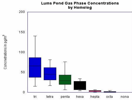
Figure 4.1-3 PCB Air Data for the 3 DRBC Monitoring Sites
