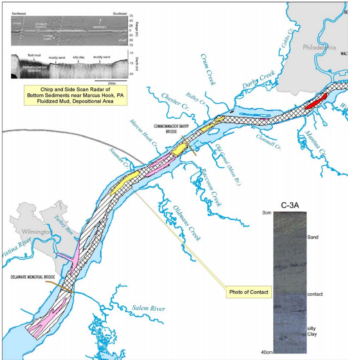
Figure 2.4-2 Sedimentation Rates in the Tidal Delaware River
