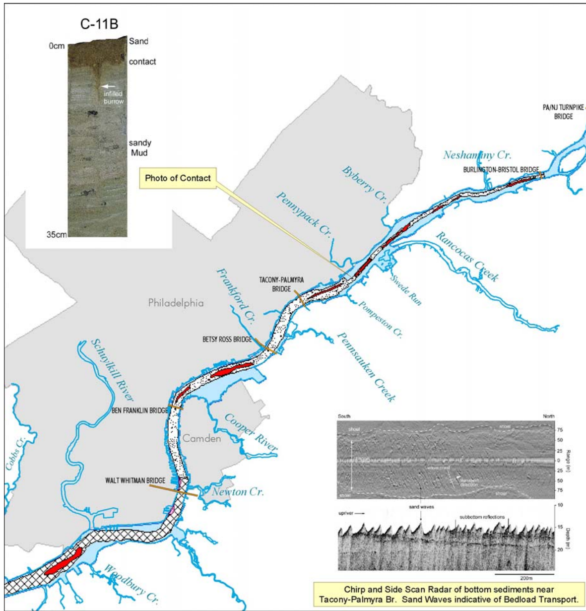
Figure 2.4-1 Spatial Distribution of Sediment Types in the Tidal Delaware River
