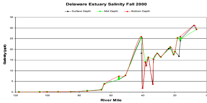
Figure 3.4-8 a-c Depth Related Data for Salinity, Dissolved Oxygen and pH from the Delaware Estuary
