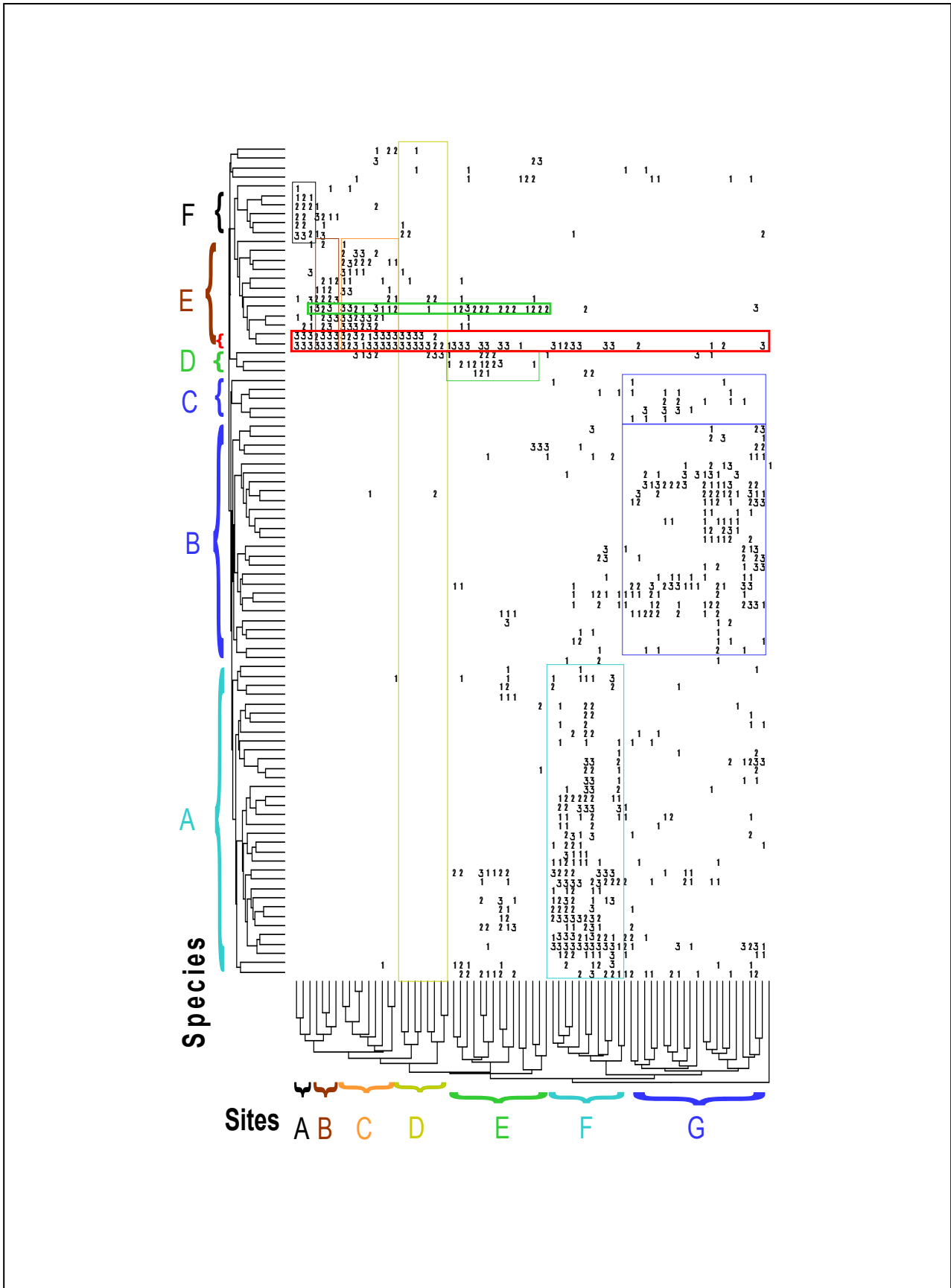
Figure 2.3-2 Nodal Analysis of Delaware Bay Benthic Communities
