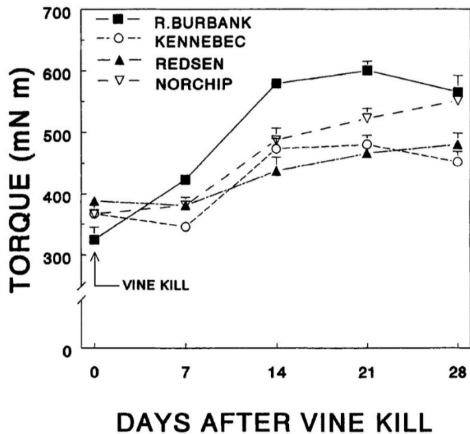
Figure 2. Differences in skin strength of four potato cultivars in 1991 non-irrigated research (Lulai and Orr, 1993).
