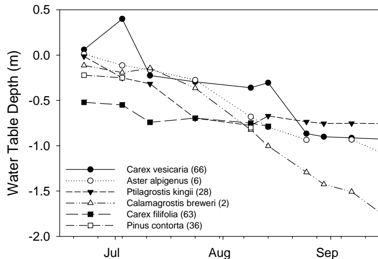
Figure 3-14. Depth to the water table below the ground surface (0.0) for one representative well in each of the six community types.
