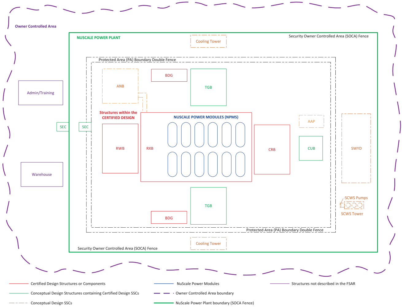
Figure 1.2-2: NuScale Functional Boundaries
