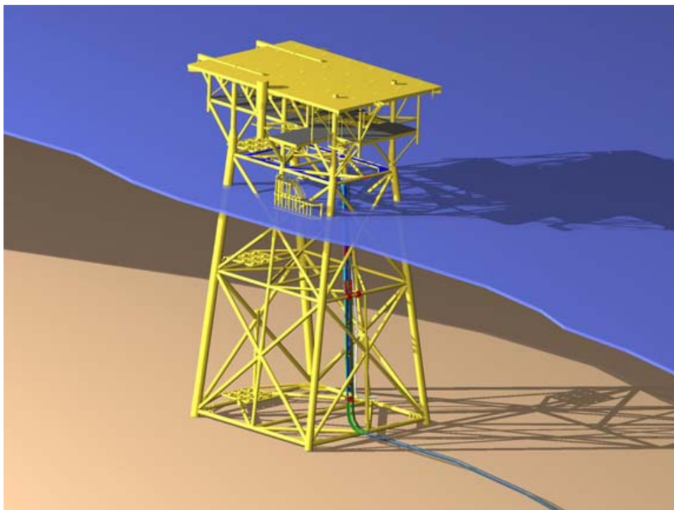
Figure 4.2. Schematic illustrating the configuration of the pipeline riser bend as the pipeline transitions from the seafloor to the vertical platform (source: Antares Offshore, http://www.antaressoffshore.com/images/close up of pltfrm with risers 1.JPG , accessed January 28, 2010).
