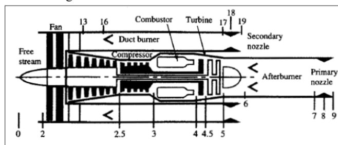
Figure 5: A gas turbine engine with station numbering used to analyze the turbofan engine flows
