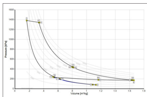
Figure 7: The Pressure-Volume Diagram (P-V diagram)
