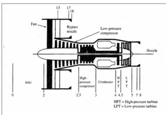
Figure 1: Schematic of a turbofan engine
