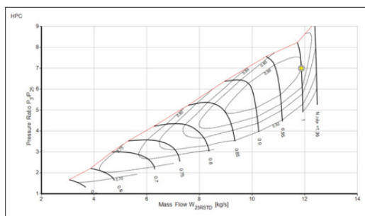
Figure 9: The High-Pressure Compressor Graph
