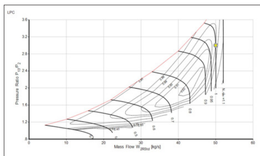
Figure 8: The Low-Pressure Compressor Graph
