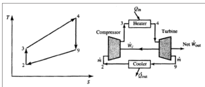
Figure 3: The Brayton cycle which includes a TS-diagram
