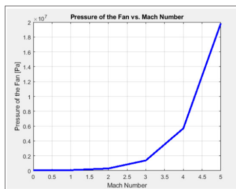
Figure 11: Pressure of the Fan vs Mach Number
