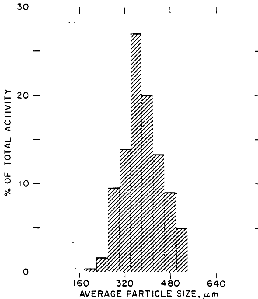
Figure 4. Activity vs granule size for Bikini ash.
