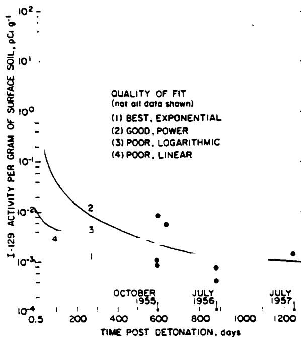
Figure 3. Curve fit of archival soil results.
