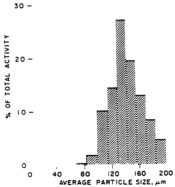
Figure 6. Activity vs granule size for Rongelap Island fallout.
