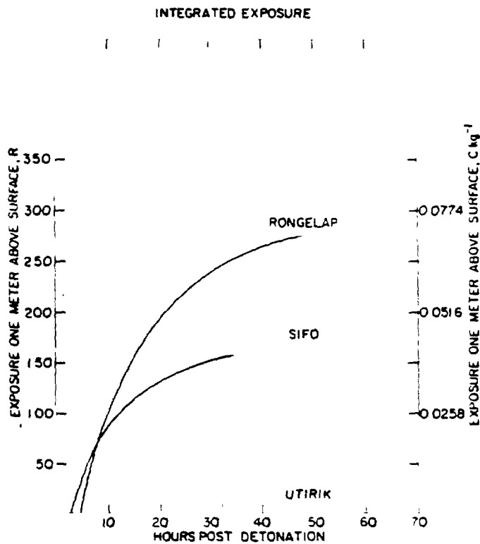
Figure 11. Integrated exposure vs time.
