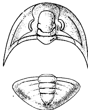
Text-figure 2. Pseudosaukia suni KOBAYASHI
