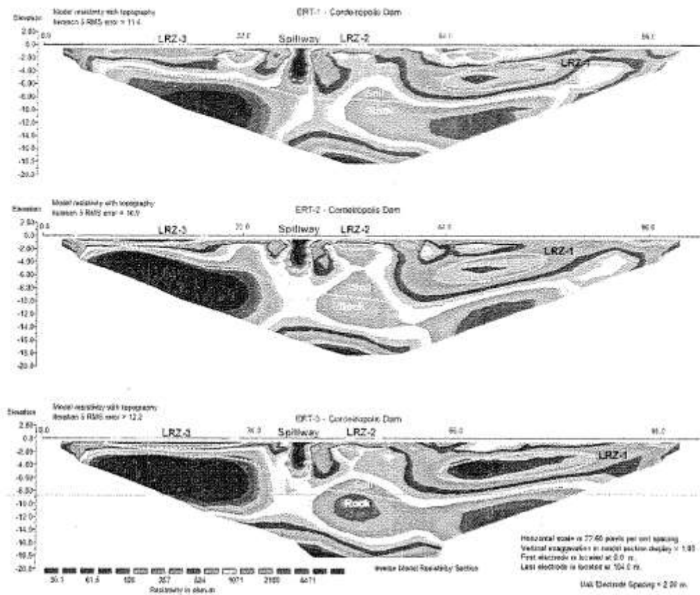
Figure 20 Geoelectric Resistivity Tomography Example
