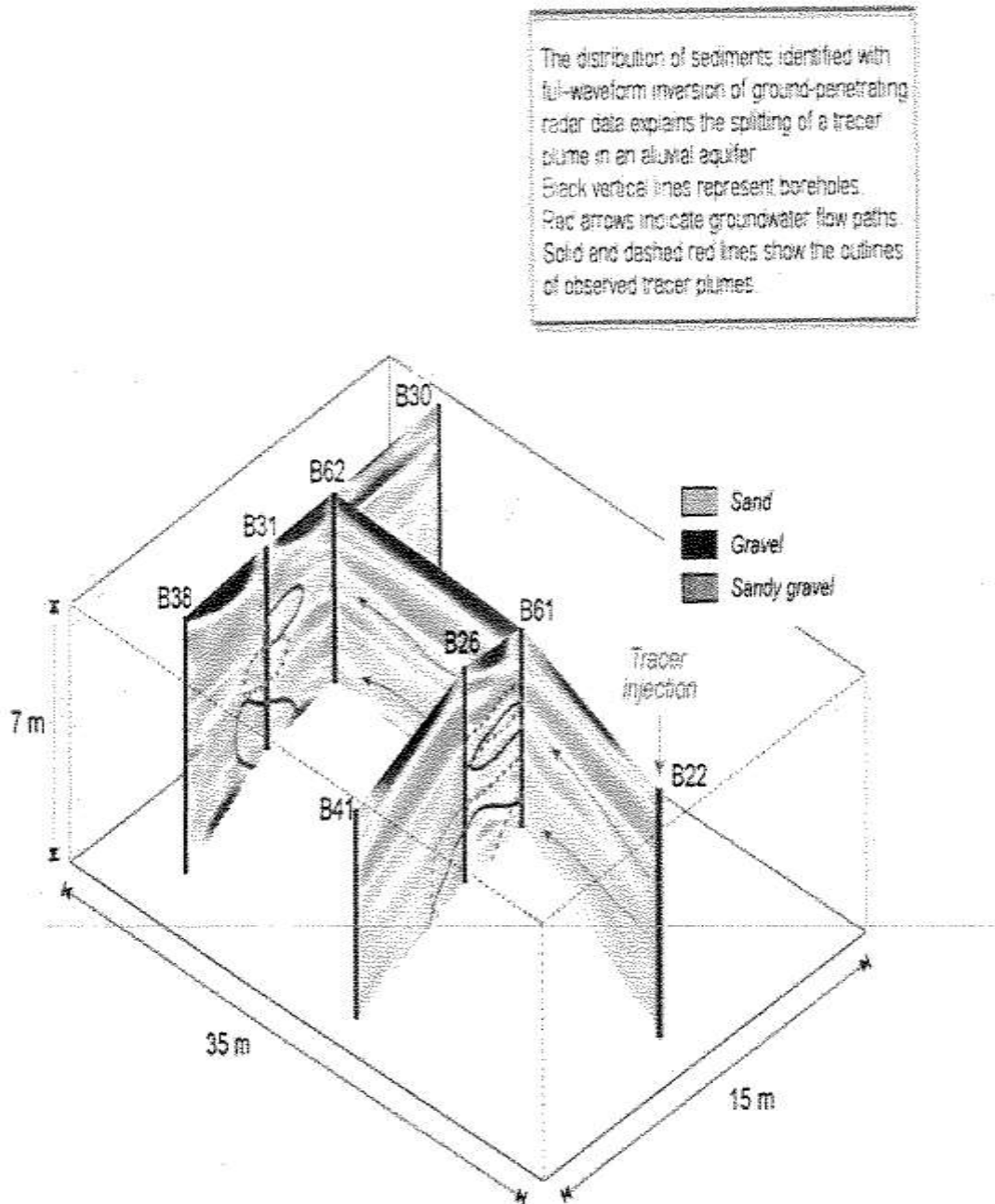
Figure 19 Πρόσφατες αναλύσεις GPR (Ground-Penetrating Radar) απο υπόγειες δομές υδάτων – Ένα παράδειγμα. A technique called full-waveform inversion more accurately reconstructs the wave's path, allowing for improved resolution.
