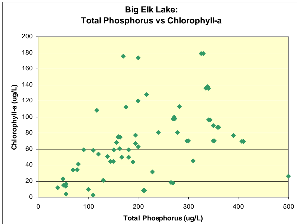
Figure 5.6 Discrete chlorophyll-a concentrations versus discrete total phosphorus concentrations for Big Elk Lake
