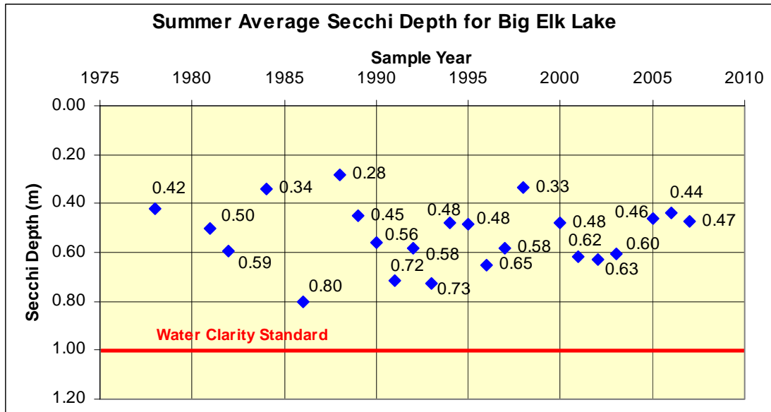
Figure 5.3 Summer average Secchi depth readings for Big Elk Lake
