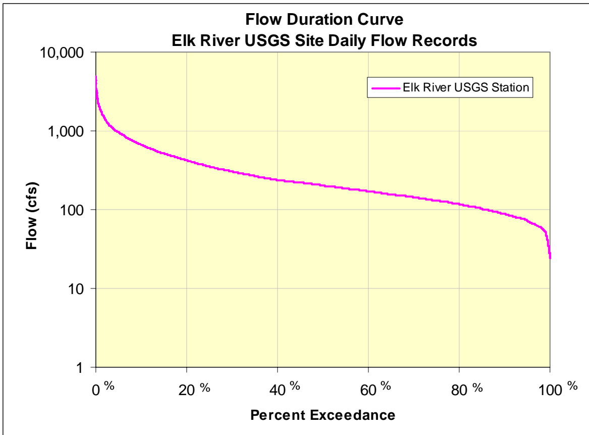
Figure 5.9 Elk River flow duration curve, river mile 9.5
