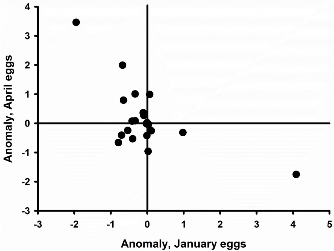
526 Figure 5. Scatterplot of relationship between egg abundances by season: anomalies from 527 common annual mean are shown (Spearman rho = -0.63).
