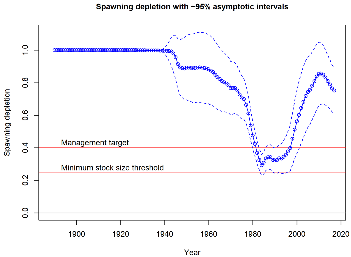
Figure e: Estimated relative depletion with approximate 95% asymptotic confidence intervals (dashed lines) for the Northern model.
