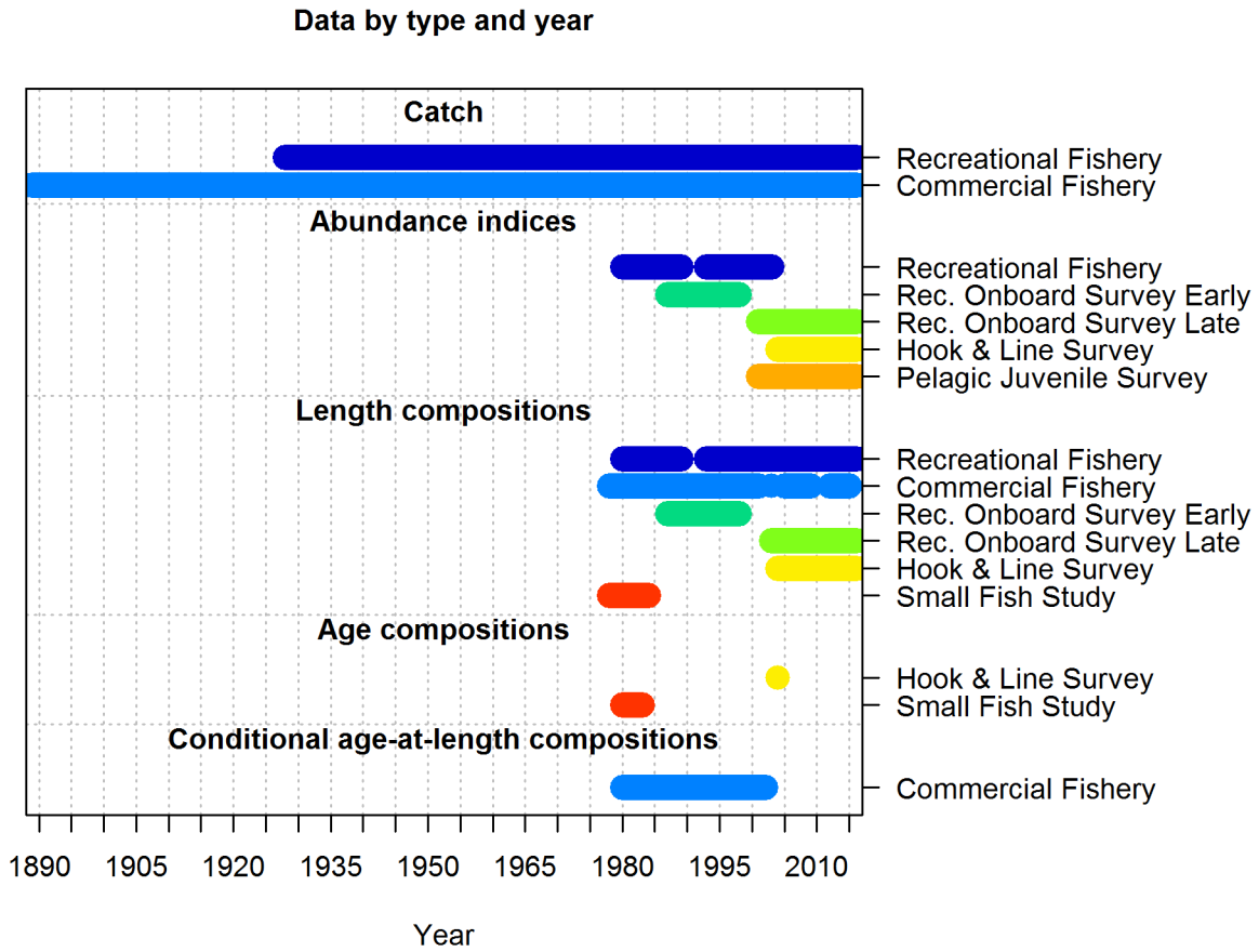
Figure 70: Summary of data sources used in the Southern model.
