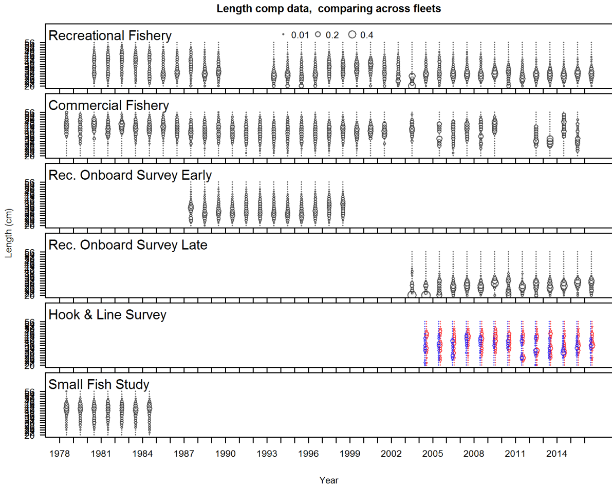
Figure 75: Length compositions for all fleets in the Southern model. Bubble size is proportional to proportions within each year.
