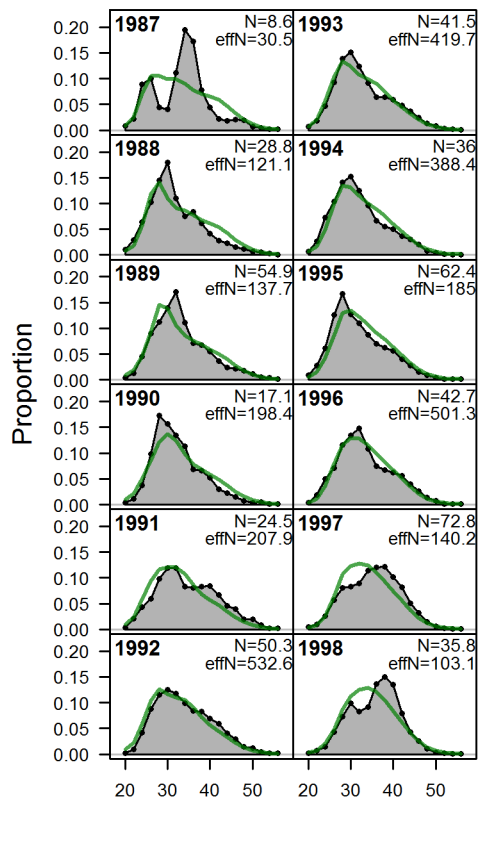
Figure 80: Southern model Length comps, retained, Rec. Onboard Survey Early
