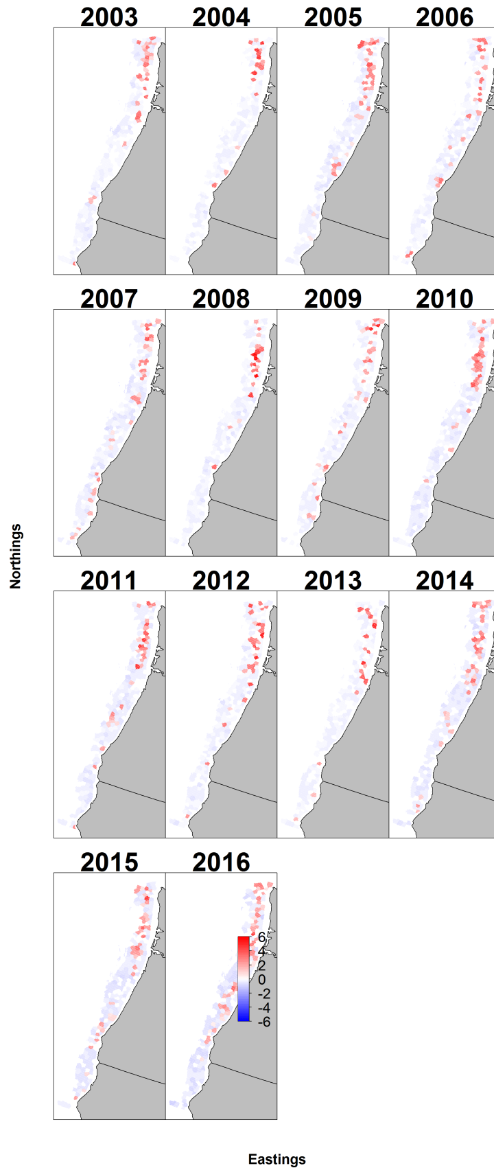
Figure 2: Pearson residuals for encounter probability in non-spatial model. D-3
