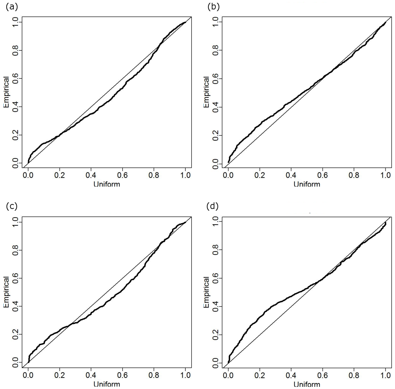
Figure 17: Quantile-Quantile plot for the VAST models for the Triennial and NWFSC Combo bottom trawl surveys for the Northern area. Panels are (a) Triennial with log-normal error distribution, (b) Triennial with gamma error distribution, (c) NWFSC Combo with log-normal error distribution, and (d) NWFSC Combo with gamma error distribution.
