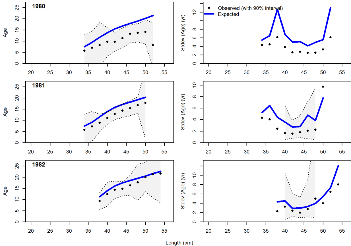
Figure 99: Southern model Conditional AAL plot, retained, Commercial Fishery (plot 1 of 8) These plots show mean age and std. dev. in conditional AAL. Left plots are mean AAL by size_class (obs. and pred.) with 90% CIs based on adding 1.64 SE of mean to the data. Right plots in each pair are SE of mean AAL (obs. and pred.) with 90% CIs based on the chi_square distribution.
