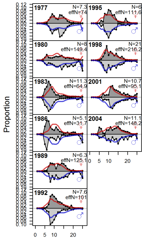
Figure 47: Northern model Age comps, retained, Triennial Survey
