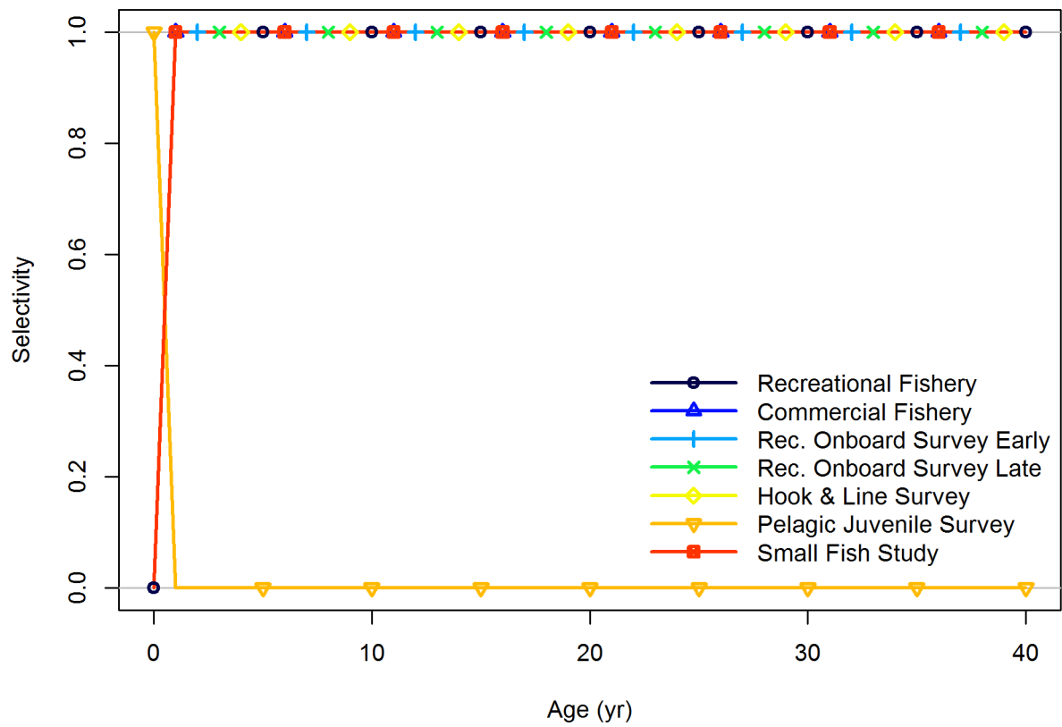
Figure 73: Fixed age-based component of selectivity for each fishery and survey in the Southern model. The Pelagic Juvenile Survey is assumed to select only age-0 fish while all other fleets are assumed to not select any age-0 fish.
