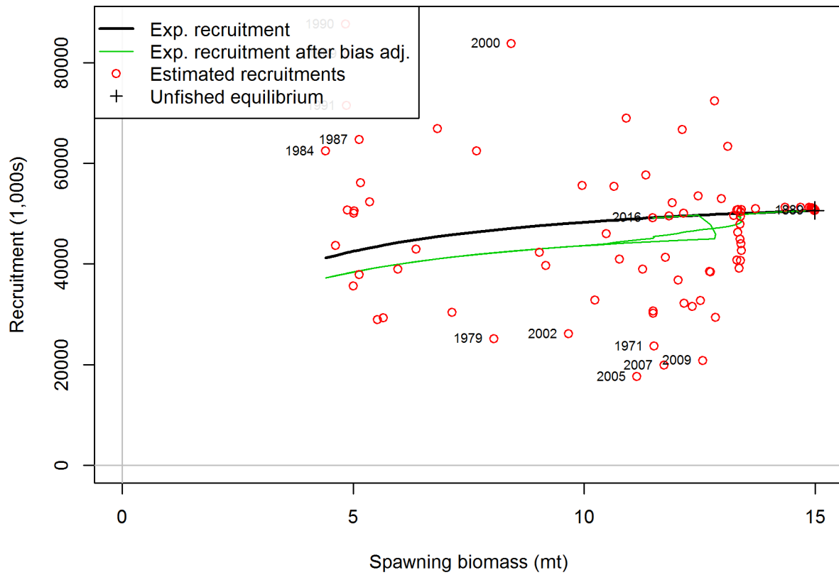
Figure 60: Estimated recruitment (red circles) for the Northern model relative to the stock-recruit relationship (black line). The green line shows the effect of the bias correction for the lognormal distribution
