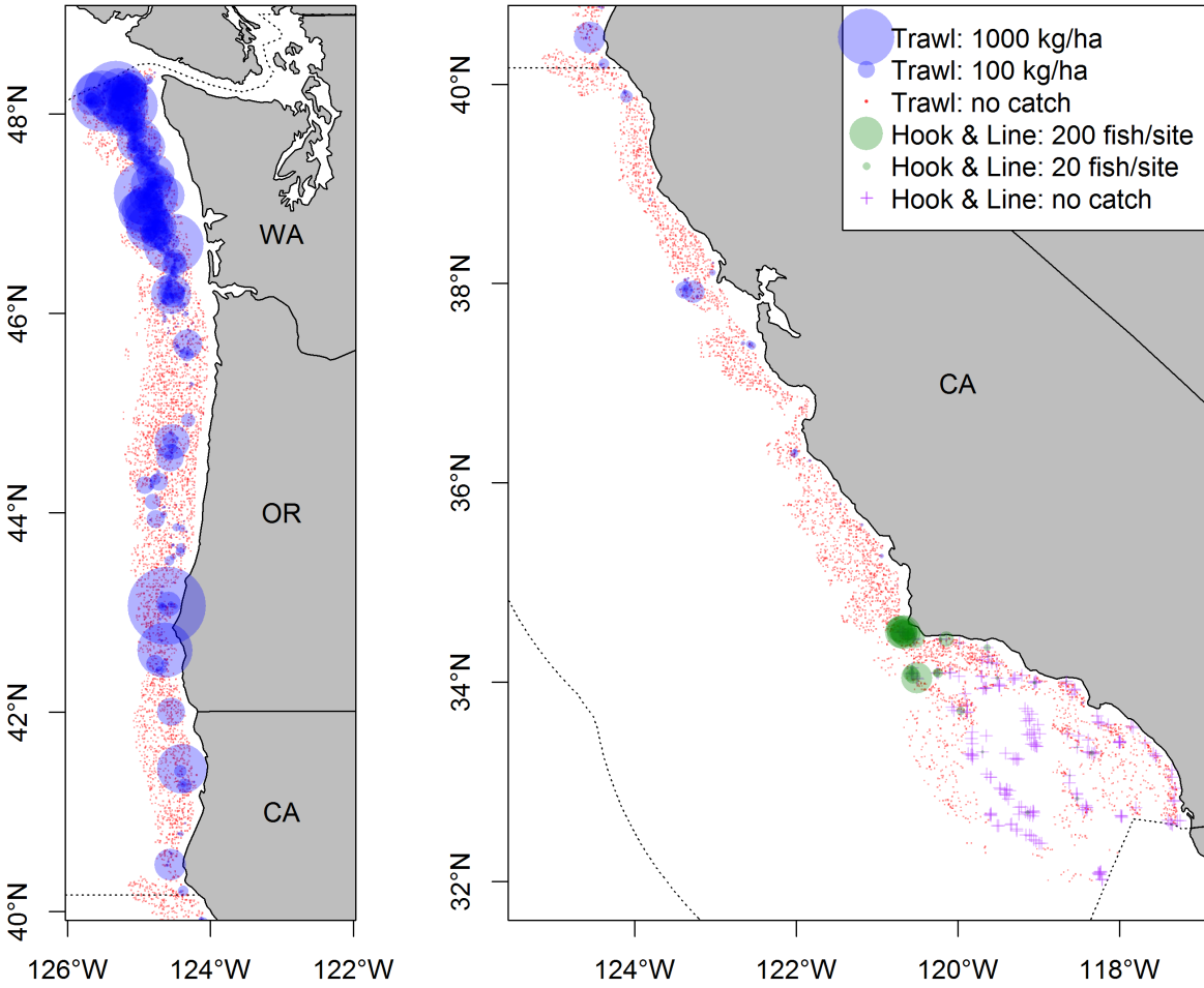
Figure 2: Map showing observations of Yellowtail Rockfish in the NWFSC Combo Survey and in the Hook & Line Survey.
