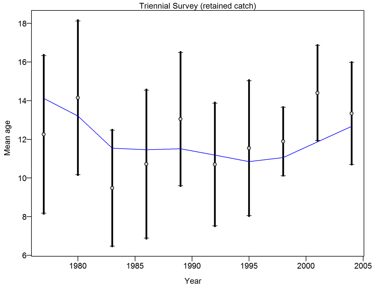
Figure 48: Northern model Mean age for Triennial Survey with 95% confidence intervals based on current samples sizes. Francis data weighting method TA1.8: thinner intervals (with capped ends) show result of further adjusting sample sizes based on suggested multiplier (with 95% interval) for age data from Triennial Survey: 1.0397 (0.6408_3.8318) For more info, see Francis, R.I.C.C. (2011). Data weighting in statistical fisheries stock assessment models. Can. J. Fish. Aquat. Sci. 68: 1124_1138.
