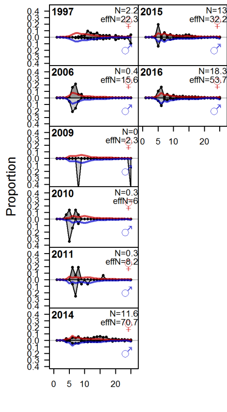
Figure 45: Northern model Age comps, retained, Recreational WA
