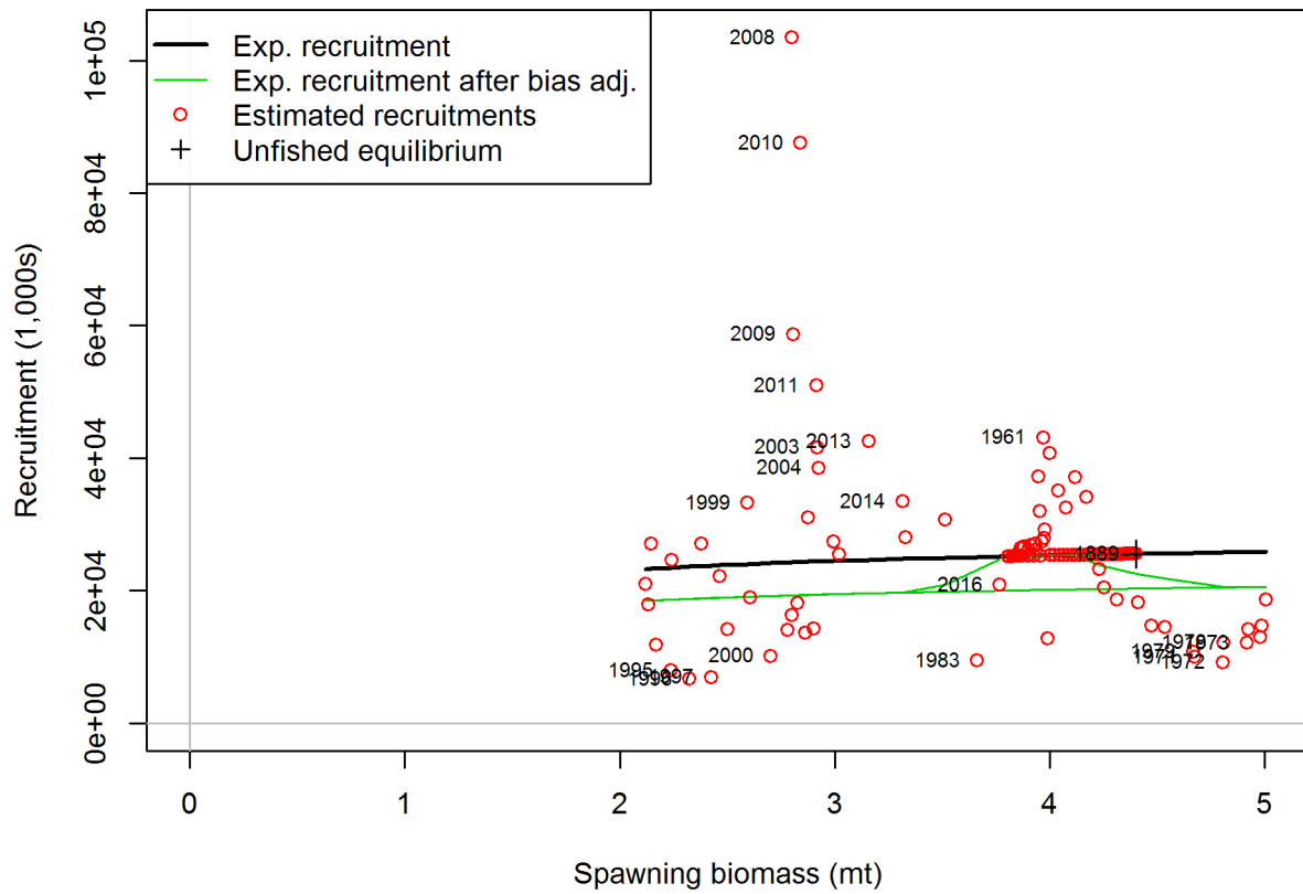
Figure 105: Estimated recruitment (red circles) for the Southern model relative to the stock-recruit relationship (black line). The green line shows the effect of the bias correction for the lognormal distribution
