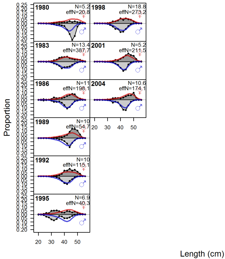
Figure 36: Northern model Length comps, retained, Triennial Survey
