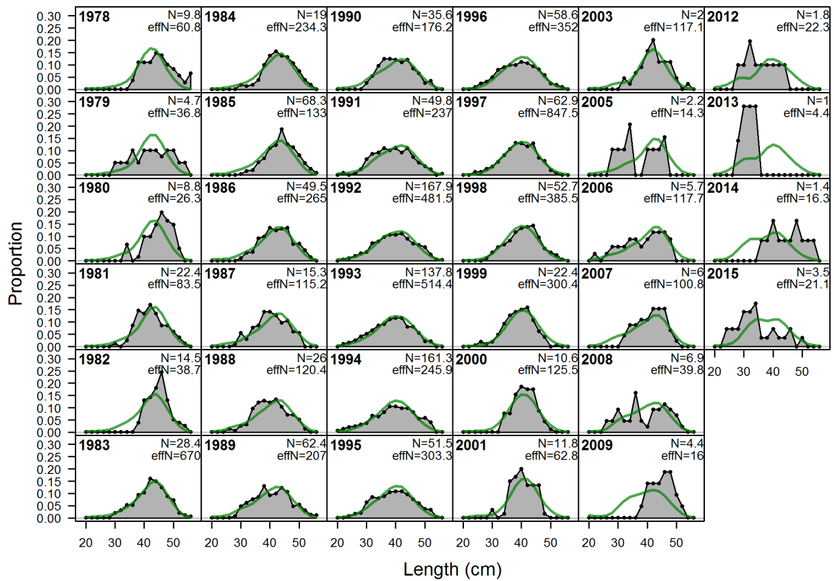
Figure 78: Southern model Length comps, retained, Commercial Fishery
