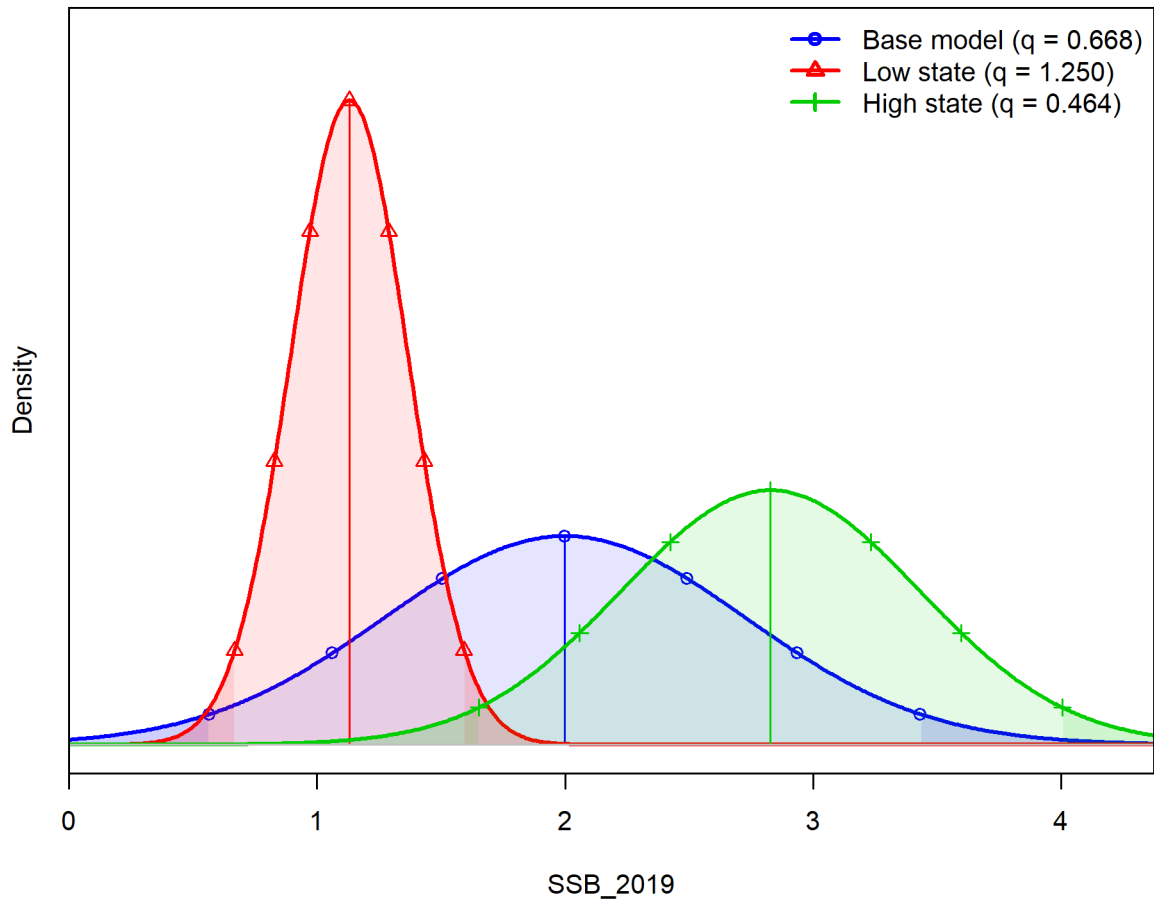
Figure B-15: Maximum likelihood estimates and approximate asymptotic uncertainty for 2019 spawning biomass (in thousands of tons) from the low and high states of nature compared to the base model. The symbols on each curve indicate the 2.5%, 10%, 25%, 50%, 75%, 90%, and 97.5% quantiles and the low and high MLE estimates are just inside the 10% and 90% quantiles.
