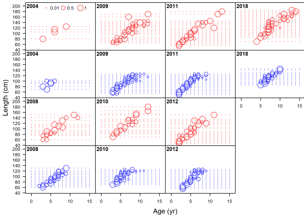
Figure 23: Conditional age-at-length data from the current fishery.
