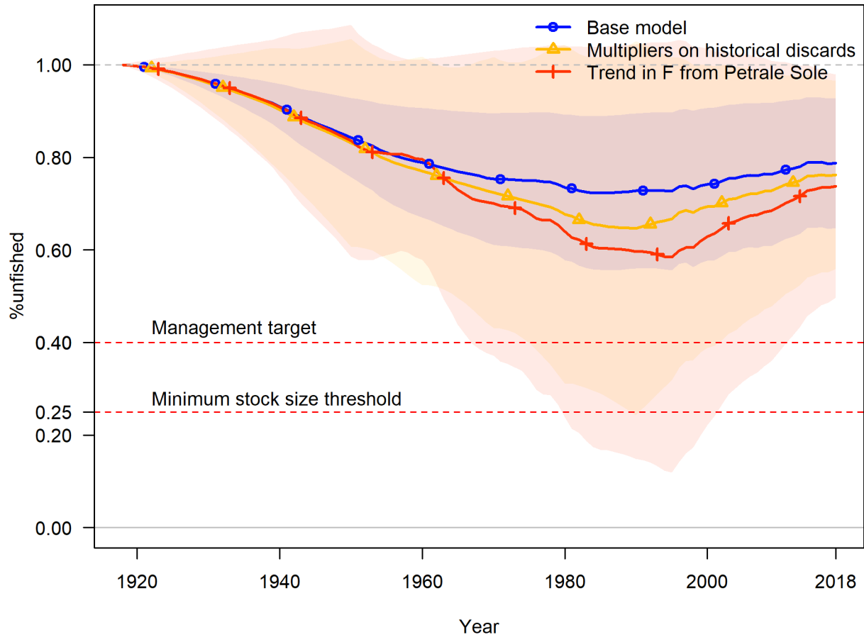
Figure 58: Time series of fraction unfished with approximate 95% asymptotic intervals estimated for the base model and the sensitivity analyses where historic catch was adjusted either by the estimated multipliers or to match the time series of F for Petrale Sole.
