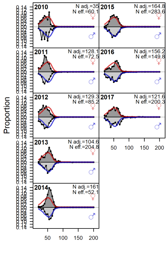
Figure A-2: Length comps, discard, Fishery. ‘N adj.’ is the input sample size after data_weighting adjustment. N eff. is the calculated effective sample size used in the McAlister_Iannelli tuning method.
