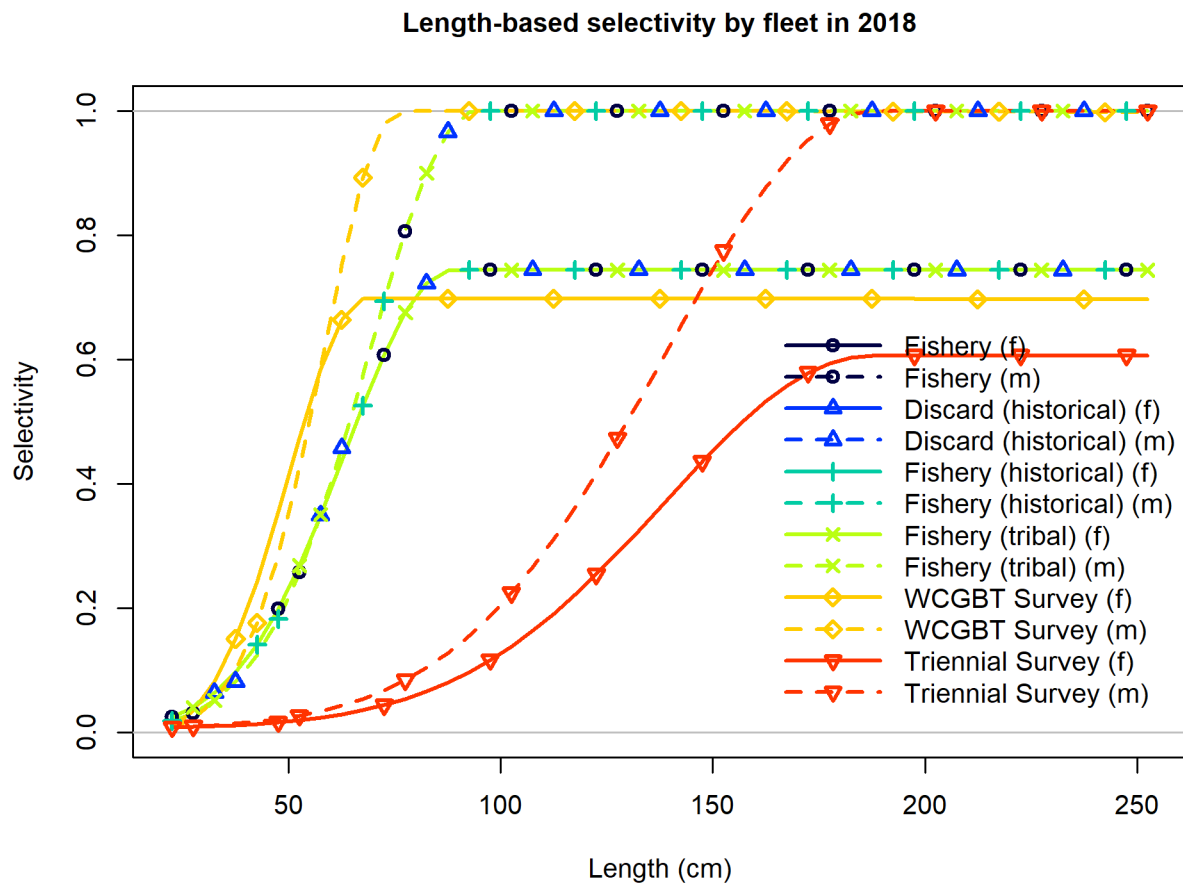
Figure 30: Selectivity at length for all of the fleets in the base model. Female selectivity is shown in the solid lines and males in the dashed lines.
