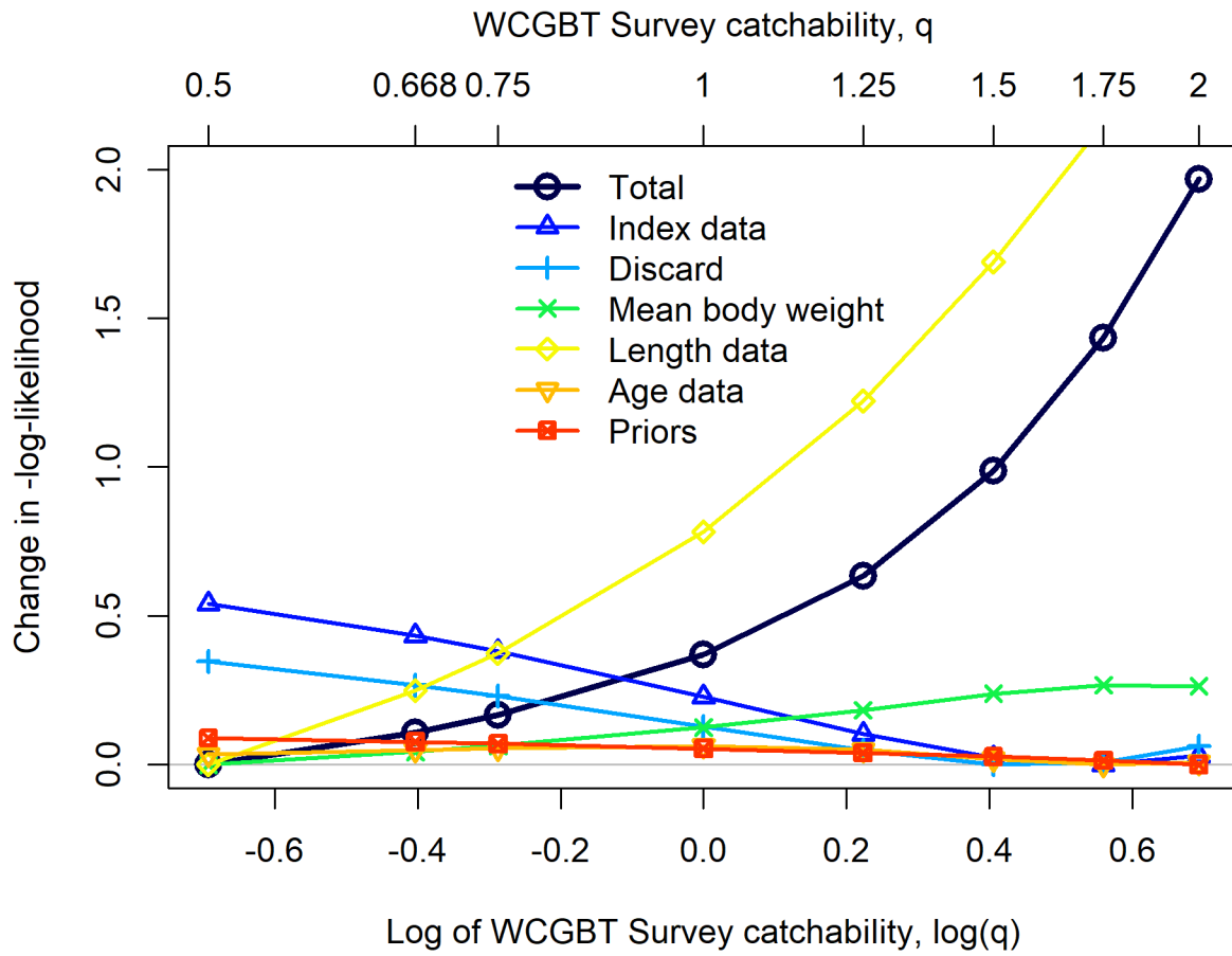
Figure 62: Likelihood profile over the catchability of the WCGBT survey ( q ) without the addition of the prior likelihood for q (the prior on natural mortality remains).
