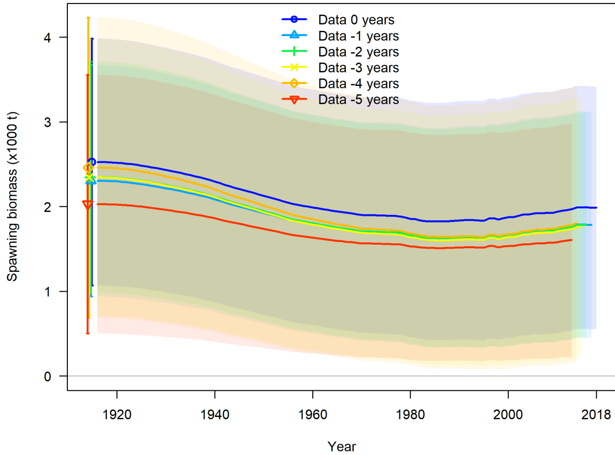
Figure 59: Time series of spawning biomass (mt) with approximate 95% asymptotic intervals estimated in retrospective analyses in which the final 5 years of data are successively removed from the model.
