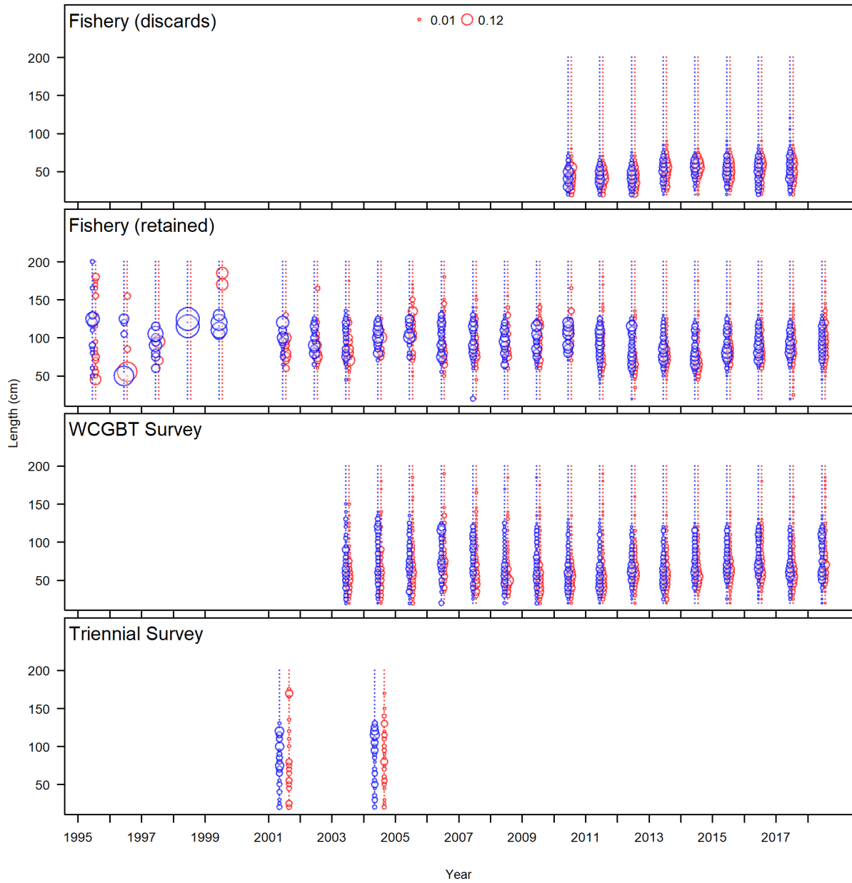
Figure 22: Length comp data for all years and fleets. Bubble size indicates the observed proportions, with females in red and males in blue.
