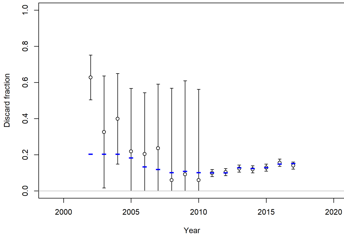
Figure 42: Fit to the discard fraction estimates. Points are model estimates with 95% uncertainty intervals. The model estimate is shown in the blue lines.
