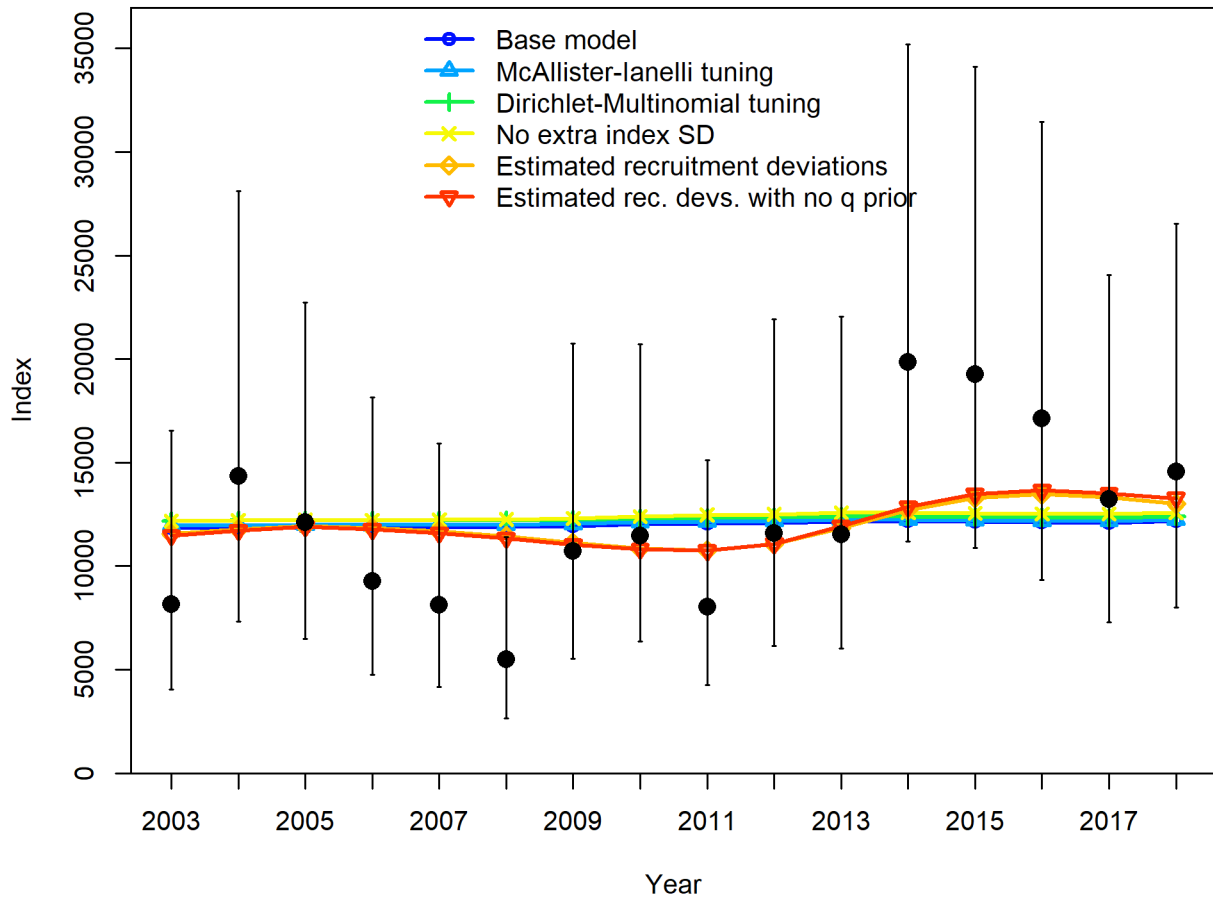
Figure 52: Fit to the WCGBT Survey estimated in the sensitivity analyses related to data weighting and recruitment.
