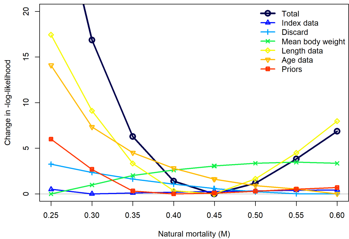
Figure 67: Likelihood profile over natural mortality ( M ).
