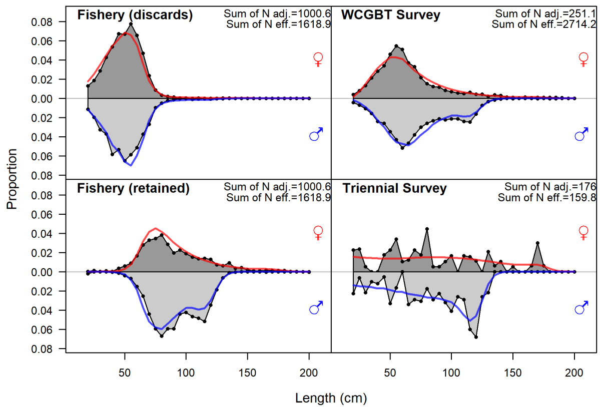
Figure 36: Fits to length composition data, aggregated across time by fleet.
