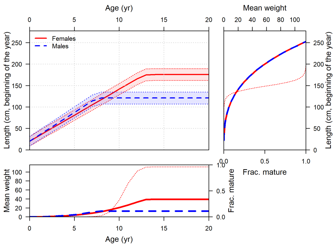
Figure 28: Estimated length-at-age for female and male Big Skate (top left panel). Shaded areas indicate 95% intervals for distribution of lengths at each age. Values represent beginning-of-year growth. Weight (thick line) and maturity (thin line) are shown in the top-right and lower-left panels as a function of length and age, respectively, where the values-at-age are calculated by mapping the length-based relationships through the estimated distribution of length at each age.
