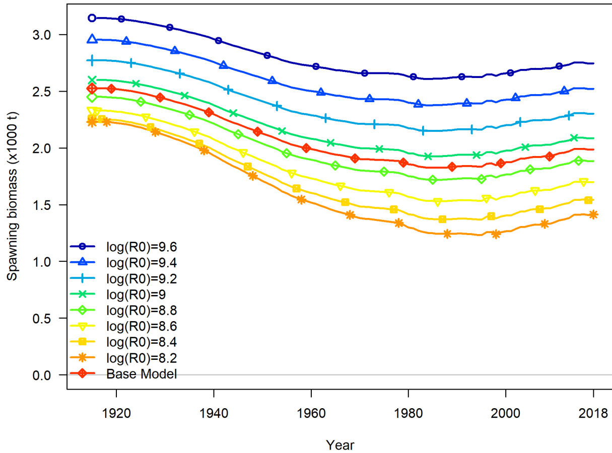
Figure 61: Time series of spawning biomass (mt) estimated for the models included in the profile over the log of equilibrium recruitment ( R_0 ).
