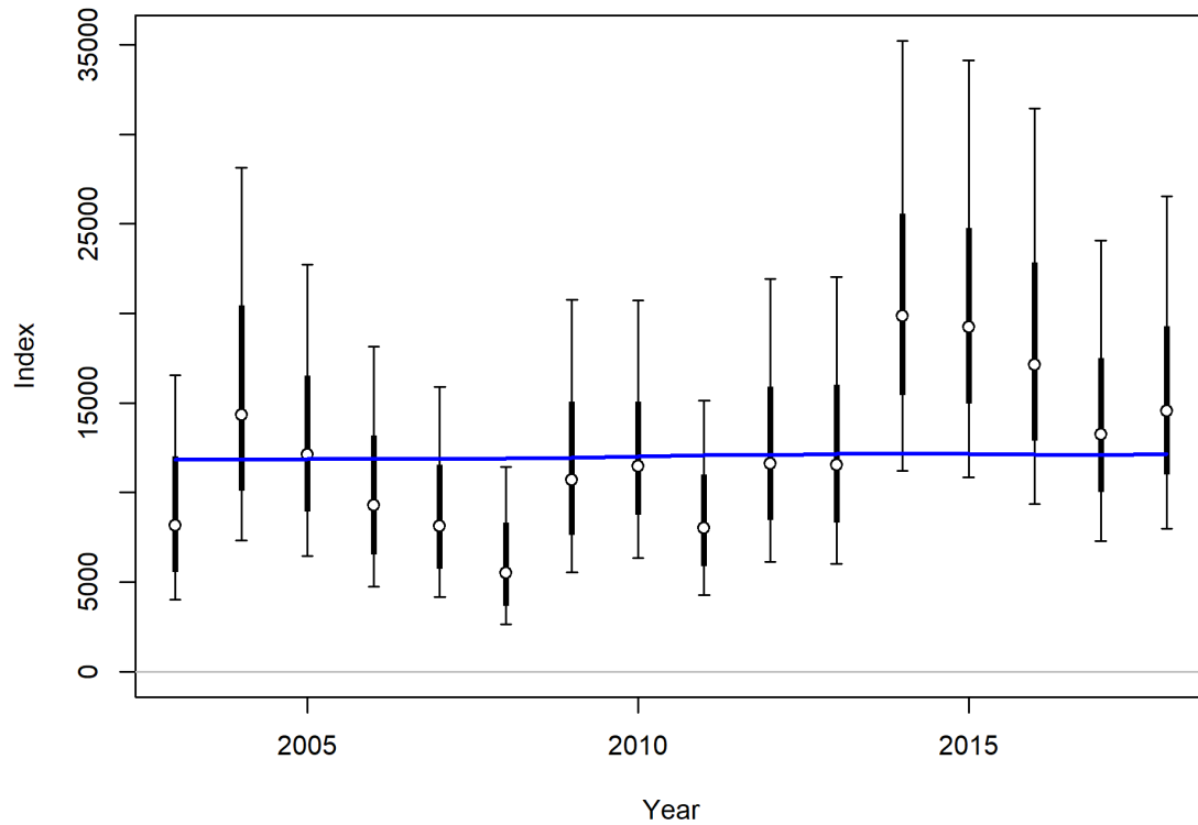
Figure 34: Fit to index data for WCGBT Survey.
