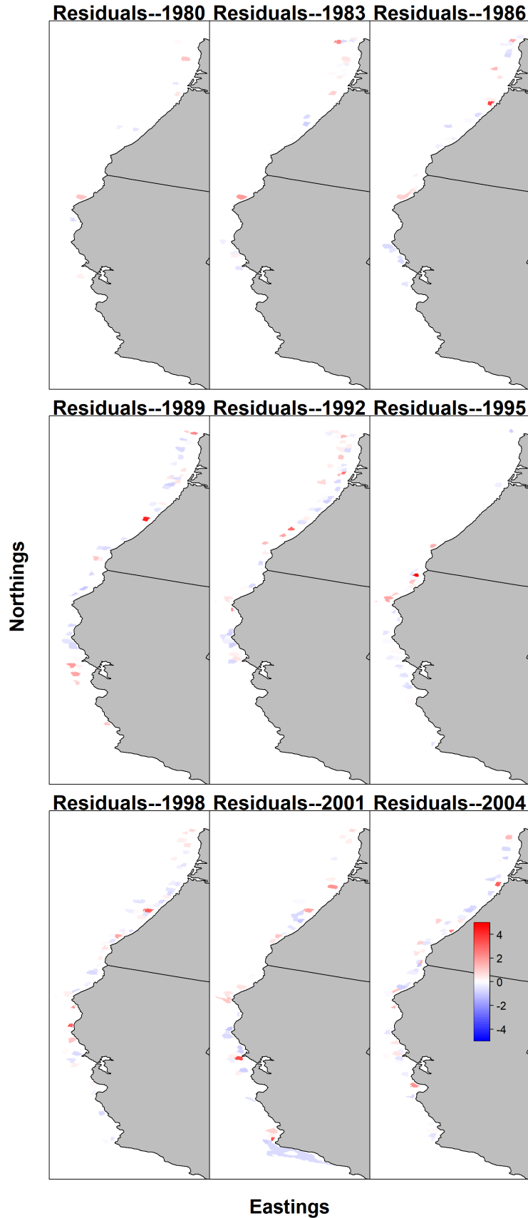
Figure 16: Map of Pearson residuals for the catch rate in the Triennial Survey associated with each knot in the VAST standardization. 85
