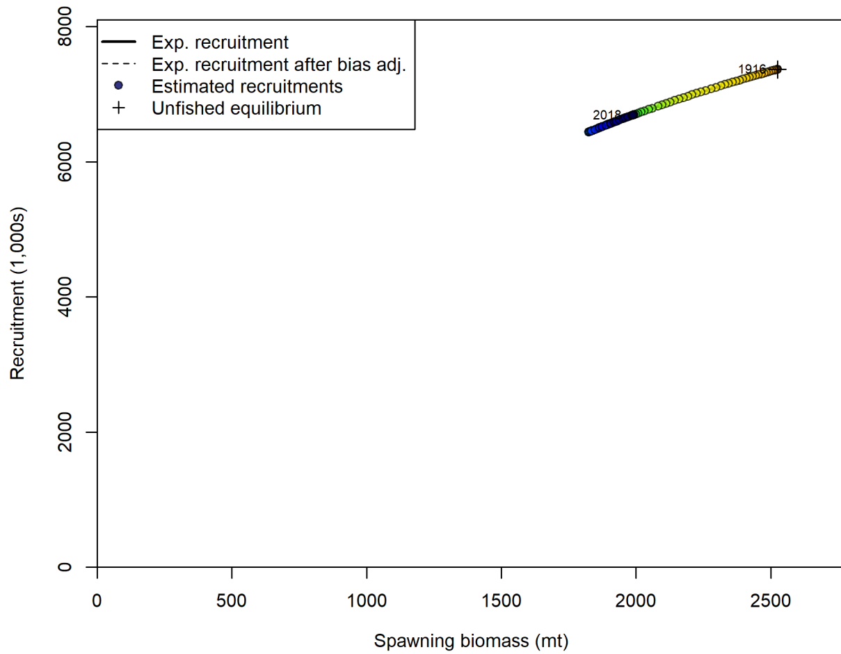
Figure 47: Estimated recruitment and the assumed stock-recruit relationship.
