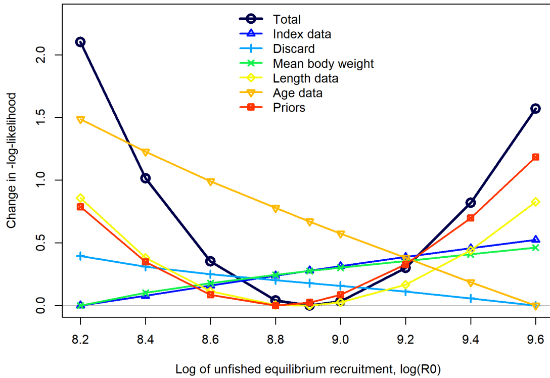
Figure 60: Likelihood profile over the log of equilibrium recruitment ( R_0 ).
