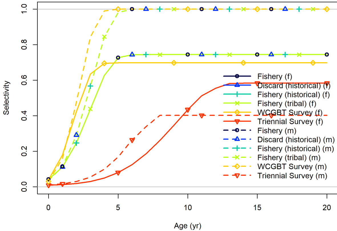
Figure 31: Selectivity at age derived from the combination of selectivity-at-length (shown above) and the estimated distribution of length at each age for all of the fleets in the base model. Female selectivity is shown in the solid lines and males in the dashed lines.
