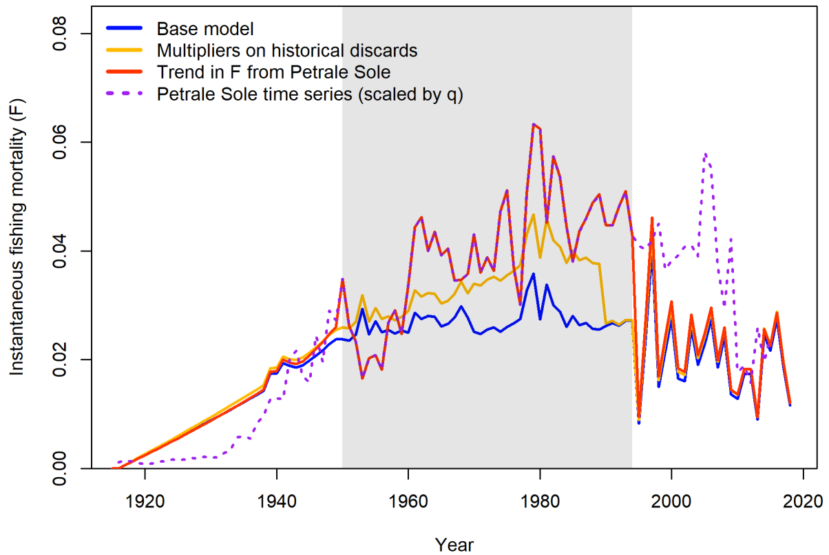
Figure 56: Comparison of the instantaneous rate of fishing mortality for fully selected ages for the base model and the sensitivity analyses where historic catch was adjusted either by the estimated multipliers or to match the time series of F for Petrale Sole. The Petrale Sole time series is shown for comparison, where the F for Petrale divided by 2.54 to match the estimated Big Skate F . The 1950–1994 period in which the Big Skate F was fit to the Petrale F is shaded in gray.
