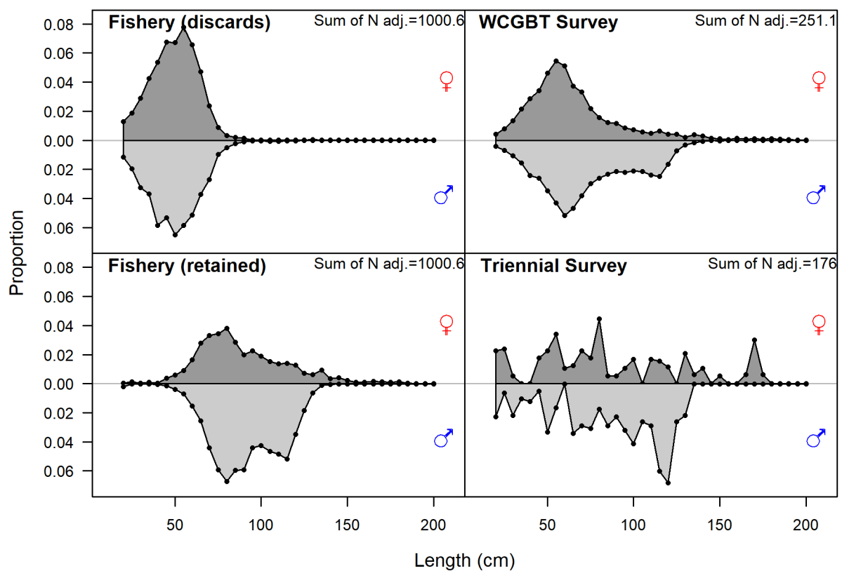
Figure 21: Length comp data, aggregated across time by fleet.
