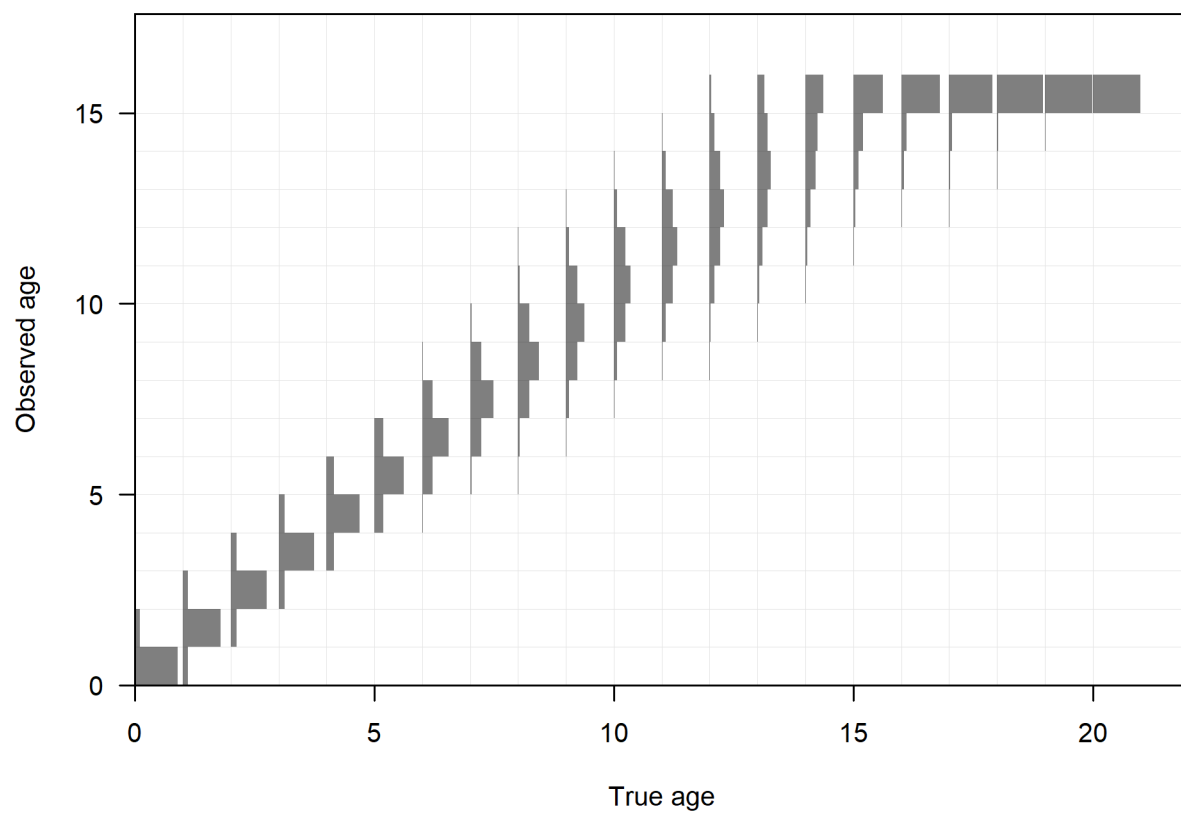
Figure 26: Estimated ageing imprecision.
