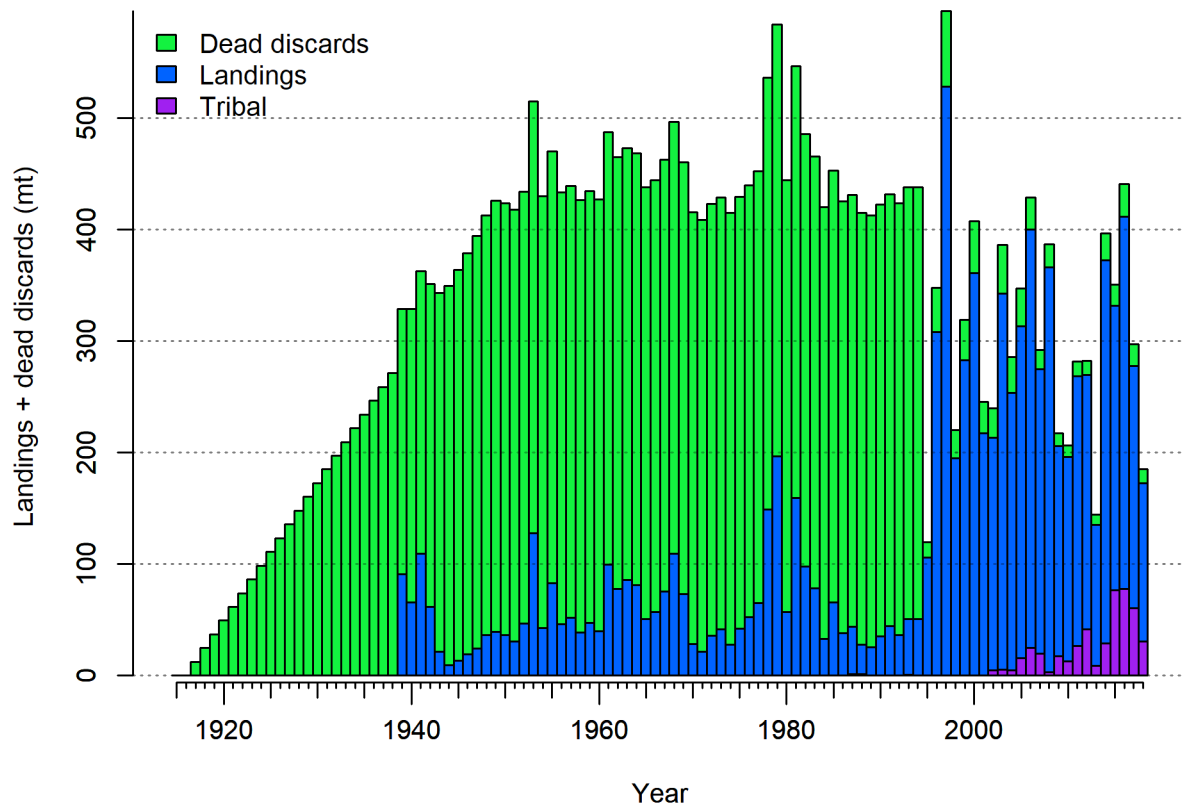
Figure 6: Estimated catch history of Big Skate. Discards prior to 1995 were estimated outside the model while those from 1995 onward are estimated internally based on a time-varying retention function.
