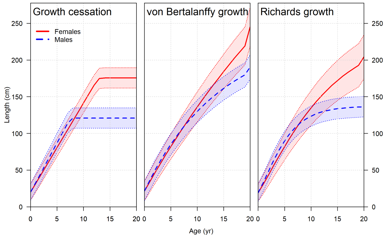
Figure 50: Comparison of the estimated growth curves from the sensitivities analyses. The increase at age 20 in the von Bertalanffy and Richards growth models is an adjustment to account for average size in the plus group based on an assumed exponential decay of the numbers at age beyond age 20.
