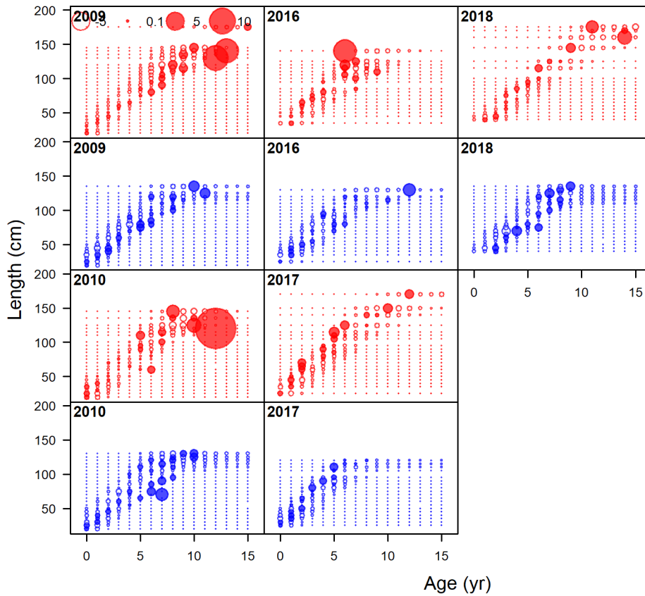
Figure 39: Pearson residuals for the fit to conditional age-at-length data from the WCGBT Survey. Closed bubbles are positive residuals (observed > expected) and open bubbles are negative residuals (observed < expected).
