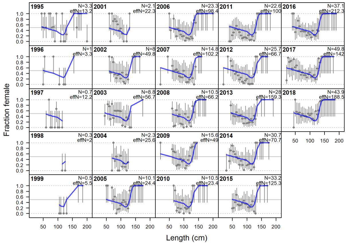
Figure 40: Observed sex ratios (points) from the fishery length composition data with 75% intervals (vertical lines) calculated as a Jeffreys interval based on the adjusted input sample size. The model expectation is shown in the blue line.
