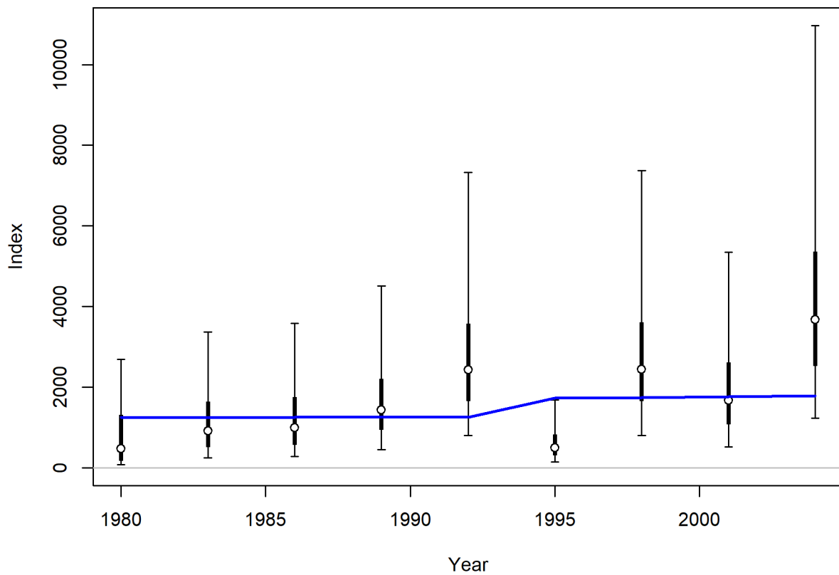
Figure 35: Fit to index data for Triennial Survey. Lines indicate 95% uncertainty interval around index values. Thicker lines indicate input uncertainty before addition of estimated additional uncertainty parameter. The blue line indicates the model estimate with a change between 1992 and 1995 associated with the estimated change in catchability.
