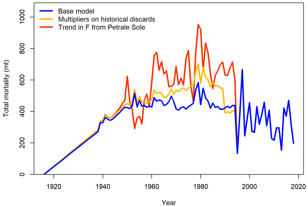
Figure 57: Comparison of total mortality for the base model and the sensitivity analyses where historic catch was adjusted either by the estimated multipliers or to match the time series of F for Petrale Sole. Total mortality shown here includes discards with the discard rate applied.
