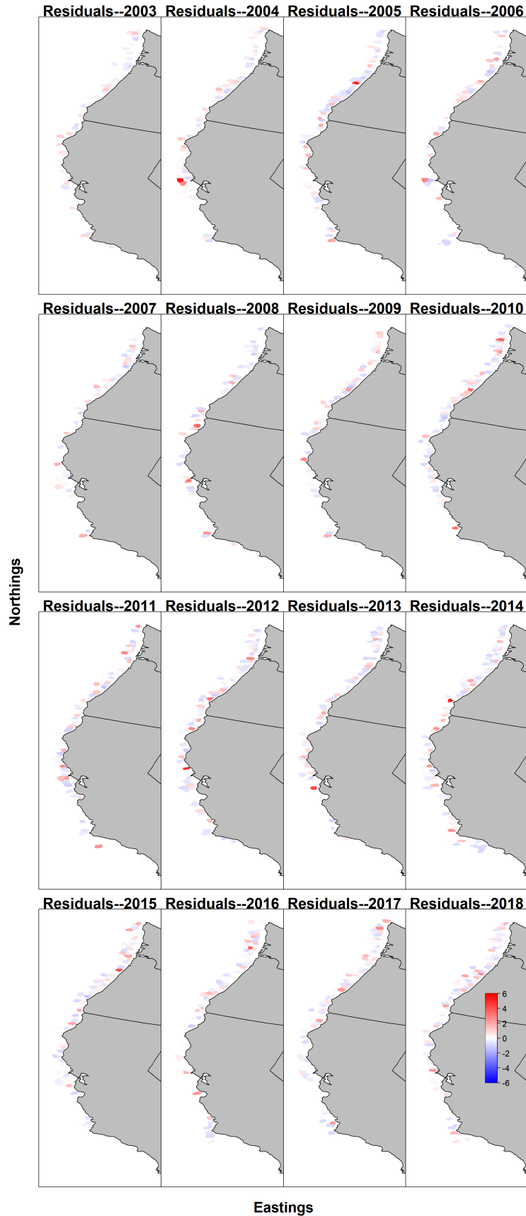
Figure 18: Map of Pearson residuals for the catch rate in the WCGBT Survey associated with each knot in the VAST standardization. 87
