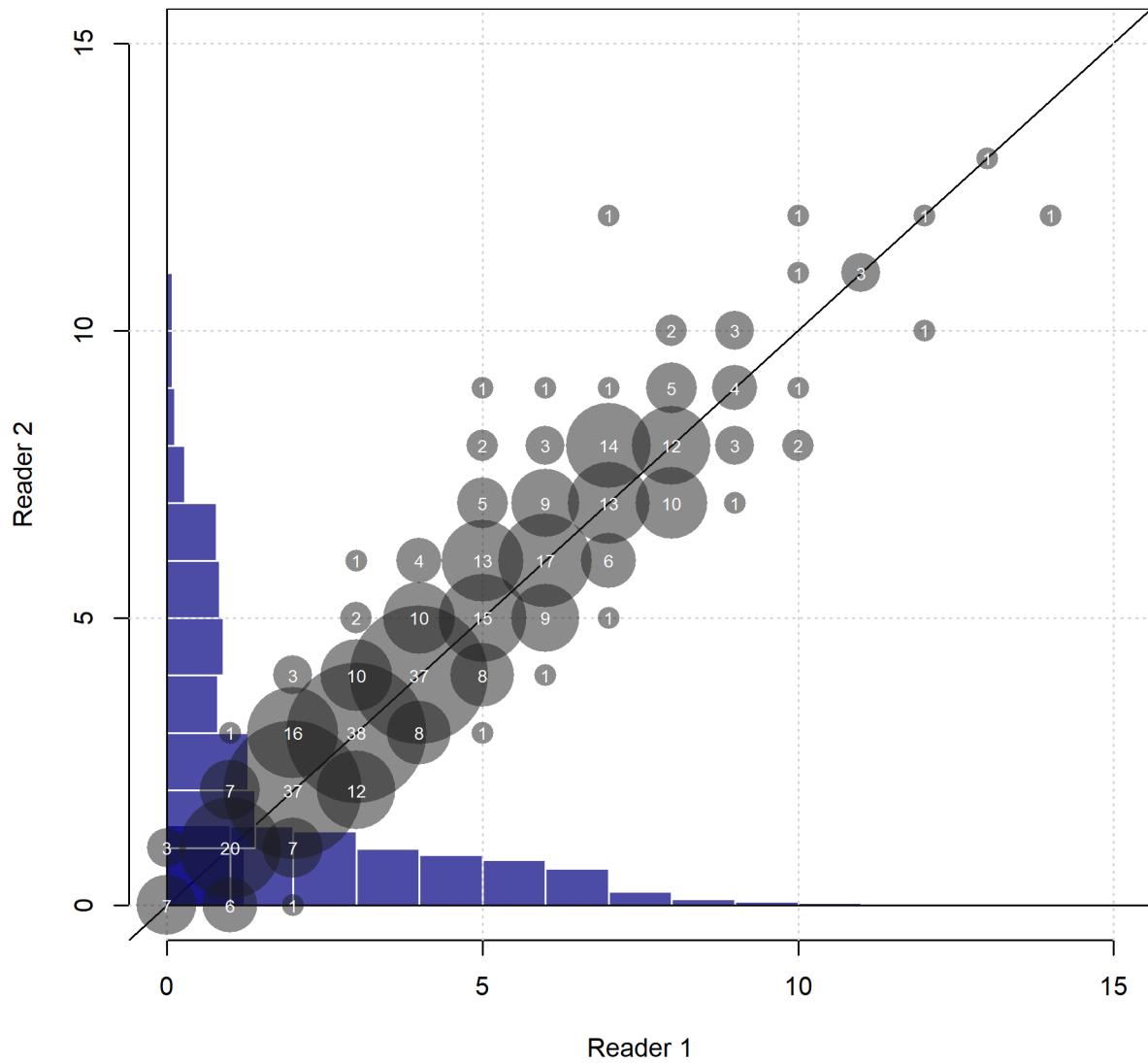
Figure 25: Comparison of reads from each of two age readers for Big Skate. Sample sizes associated with each combination of ages are shown by the size circles and the within them. The blue histograms show the distribution of ages estimated by each reader.
