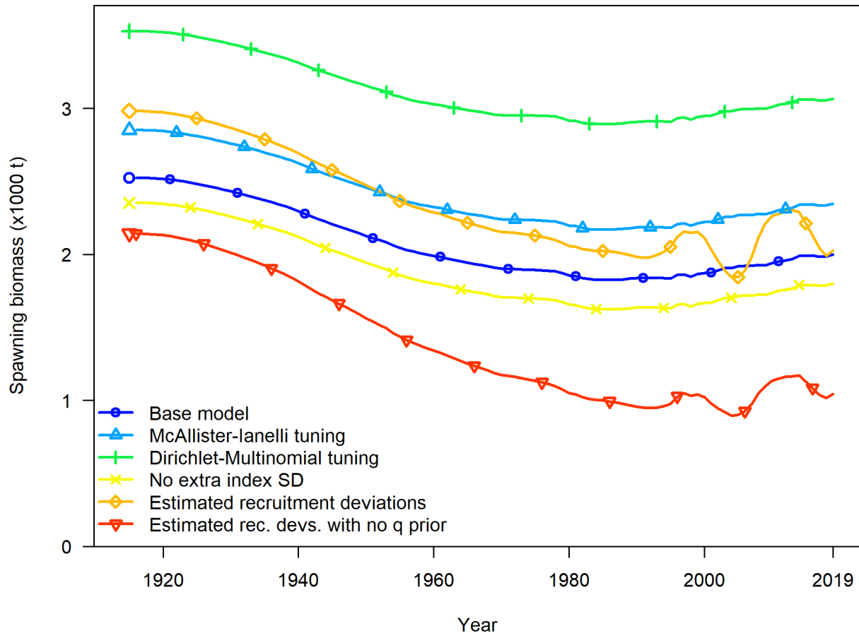
Figure 51: Time series of spawning biomass (mt) estimated in sensitivity analyses related to data weighting and recruitment.
