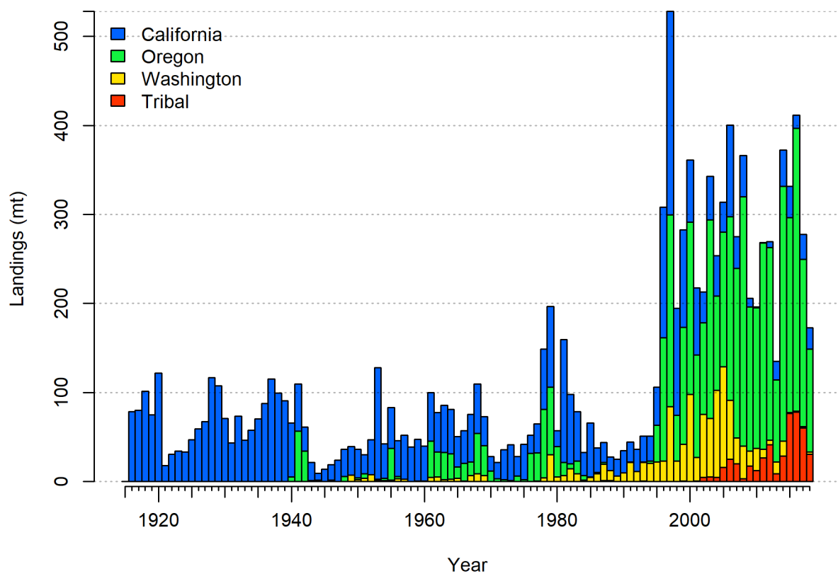
Figure 3: Reconstructed landings by area. Tribal catch was all landed in Washington.
