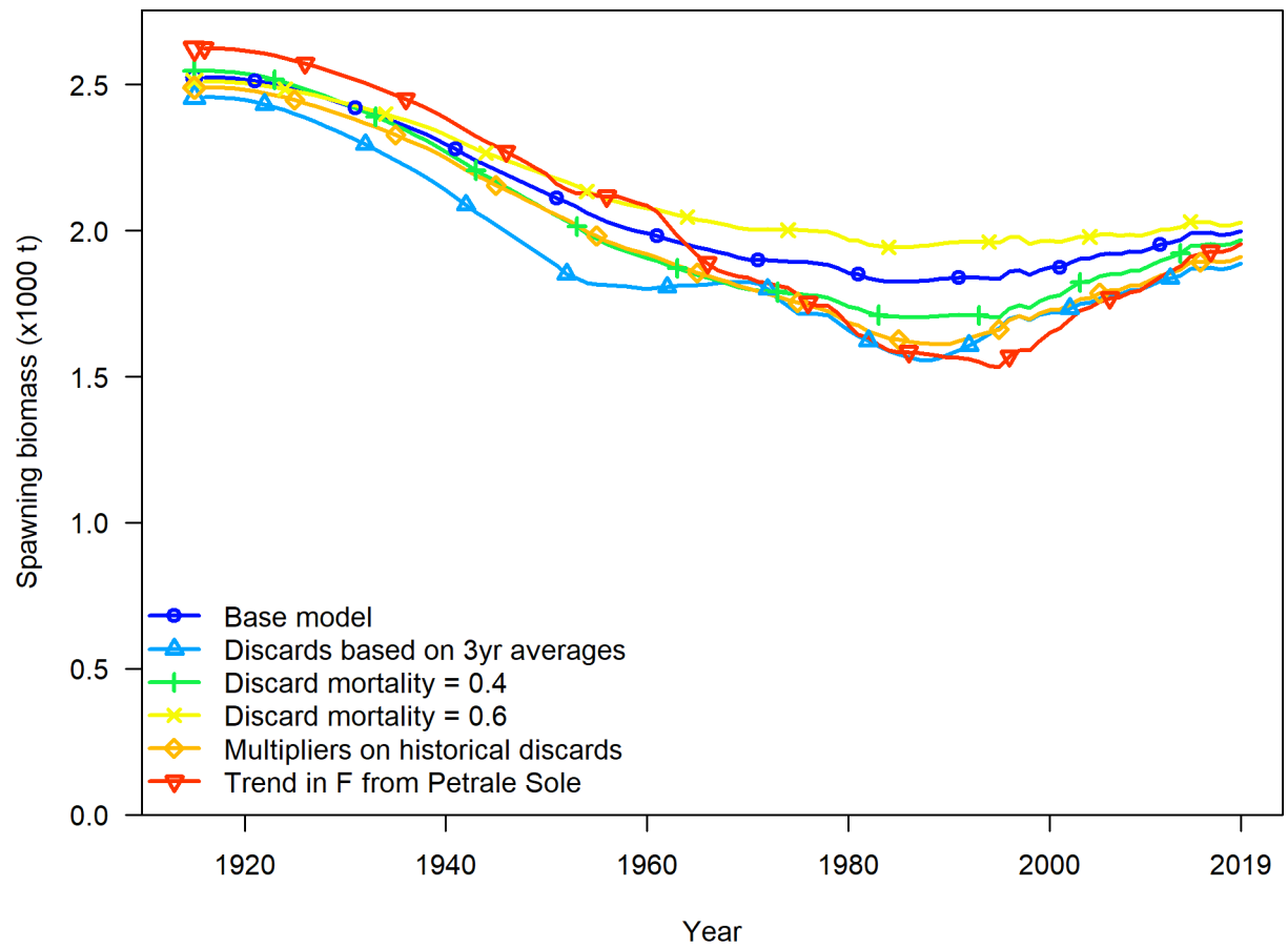
Figure 53: Time series of spawning biomass (mt) estimated in sensitivity analyses related to historic catch and discards.
