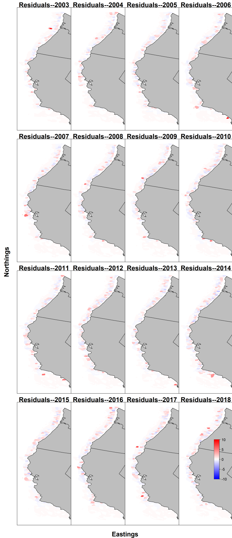
Figure 17: Map of Pearson residuals for the encounter probability in the WCGBT Survey associated with each knot in the VAST standardization.
