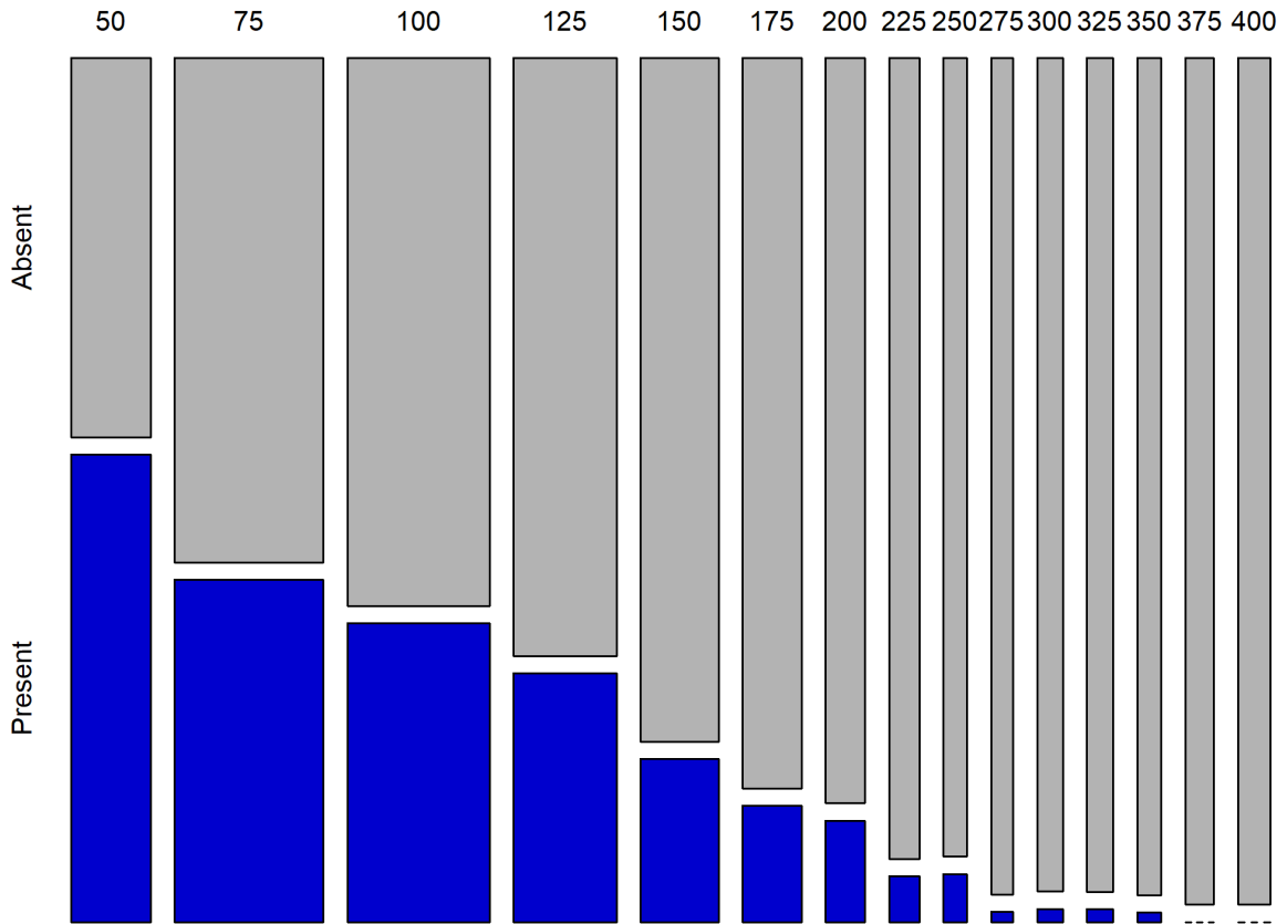
Figure 8: Presence or absence of Big Skate in the WCGBT Survey by 25 m depth bin for all 6,382 hauls with depth less than 425 m over the years 2003–2018. The height and width of each block are proportional to the number of hauls within that bin. For 50–75 m, there were 324 hauls with Big Skate present and 263 with no Big Skate.
