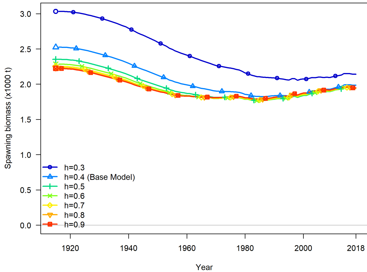
Figure 66: Time series of spawning biomass (mt) estimated for the models included in the profile over stock-recruit steepness ( h ).
