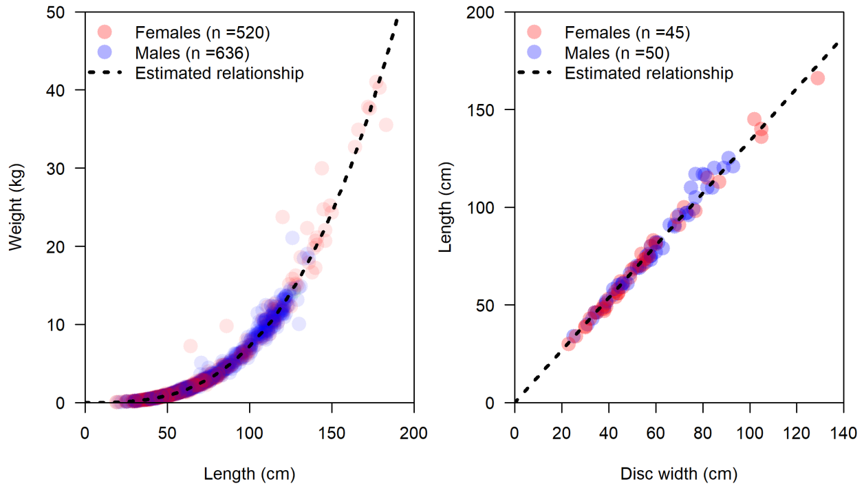
Figure 20: Estimated relationship between length and weight (left) and disc-width and length (right) for Big Skate. Colored points show observed values and the black line indicates the estimated relationship W = 0.0000074924L^{2.9925} .
