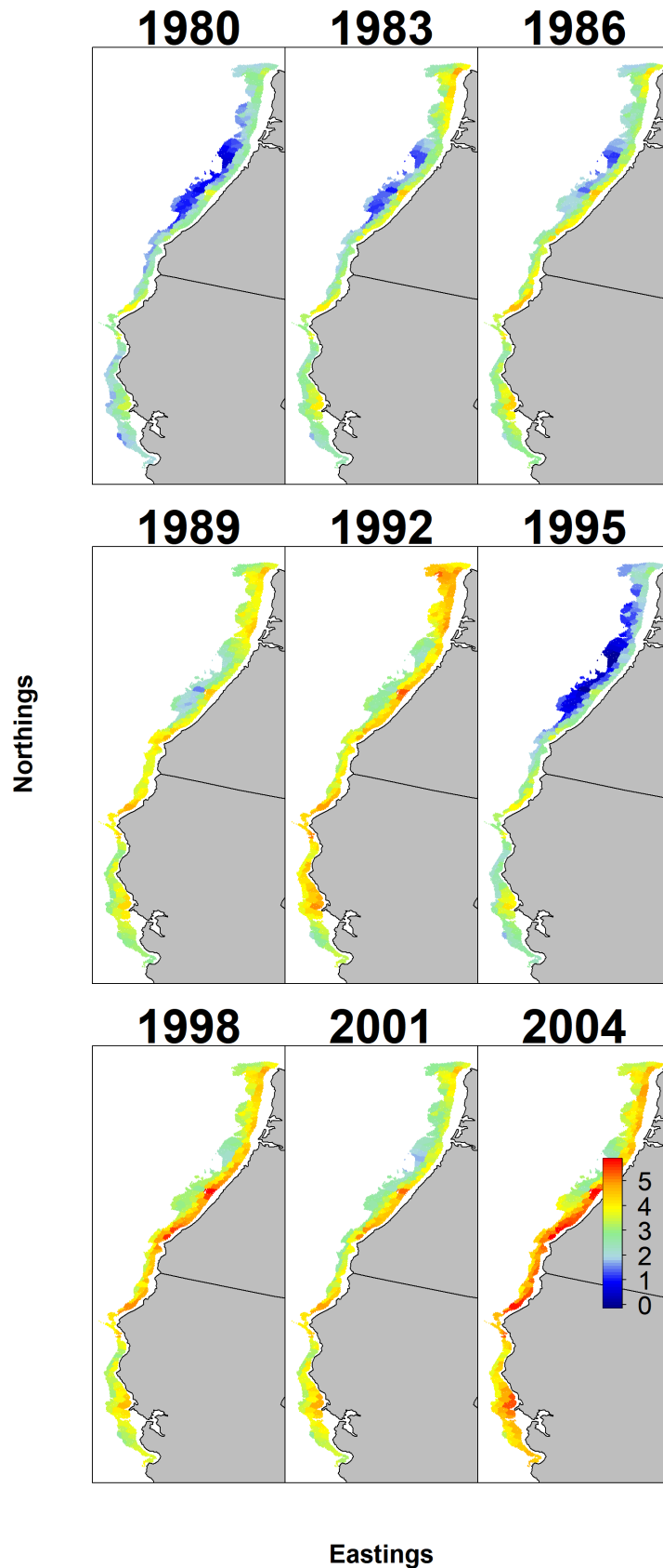
Figure 13: Map of estimated density by year for Big Skate in the Triennial survey calculated using VAST with a Gamma error structure. 82
