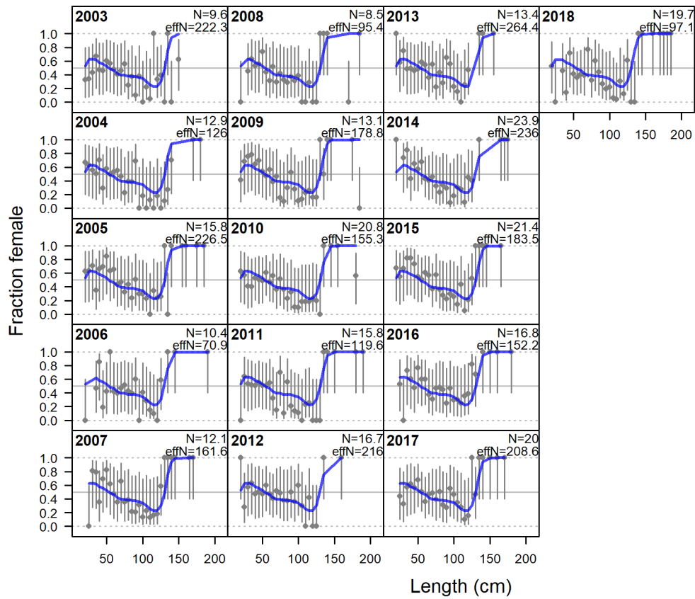
Figure 41: Observed sex ratios (points) from the WCGBT Survey length composition data with 75% intervals (vertical lines) calculated as a Jeffreys interval based on the adjusted input sample size. The model expectation is shown in the blue line.
