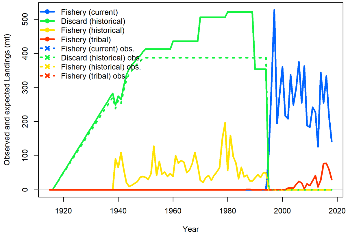
Figure 55: Catch by category for the sensitivity analysis where multipliers on historical discards were estimated. The estimated time series including the multipliers is shown in the solid green line and the input values in the base model are shown in the dashed green line.
