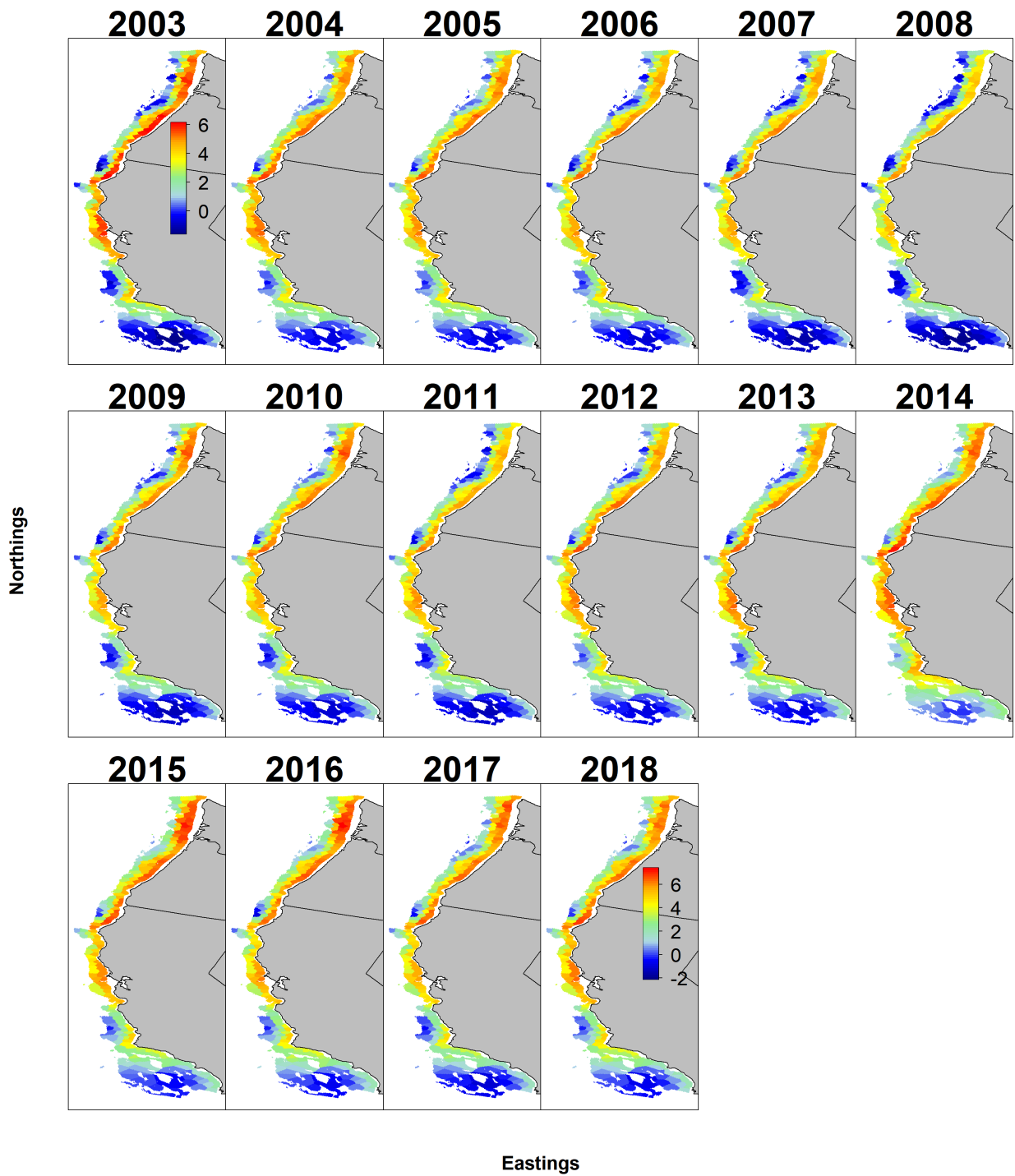
Figure 14: Map of estimated density by year for Big Skate in the WCGBT Survey calculated using VAST with a Gamma error structure.
