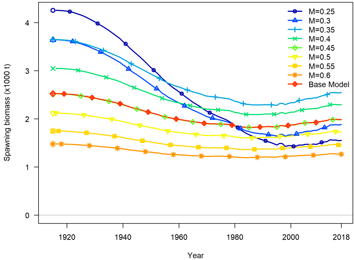
Figure 68: Time series of spawning biomass (mt) estimated for the models included in the profile over natural mortality ( M ).
