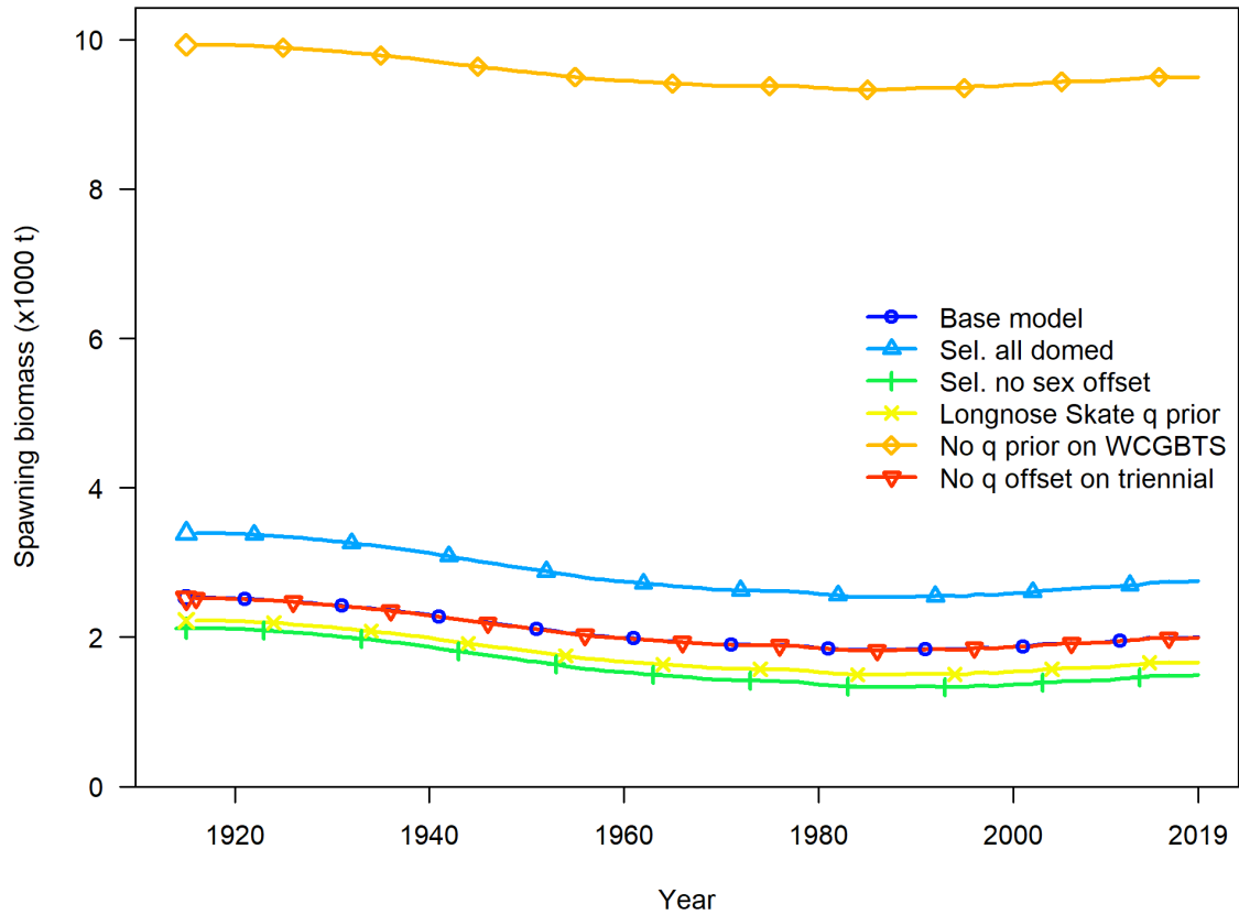
Figure 48: Time series of spawning biomass (mt) estimated in sensitivity analyses related to selectivity and catchability.
