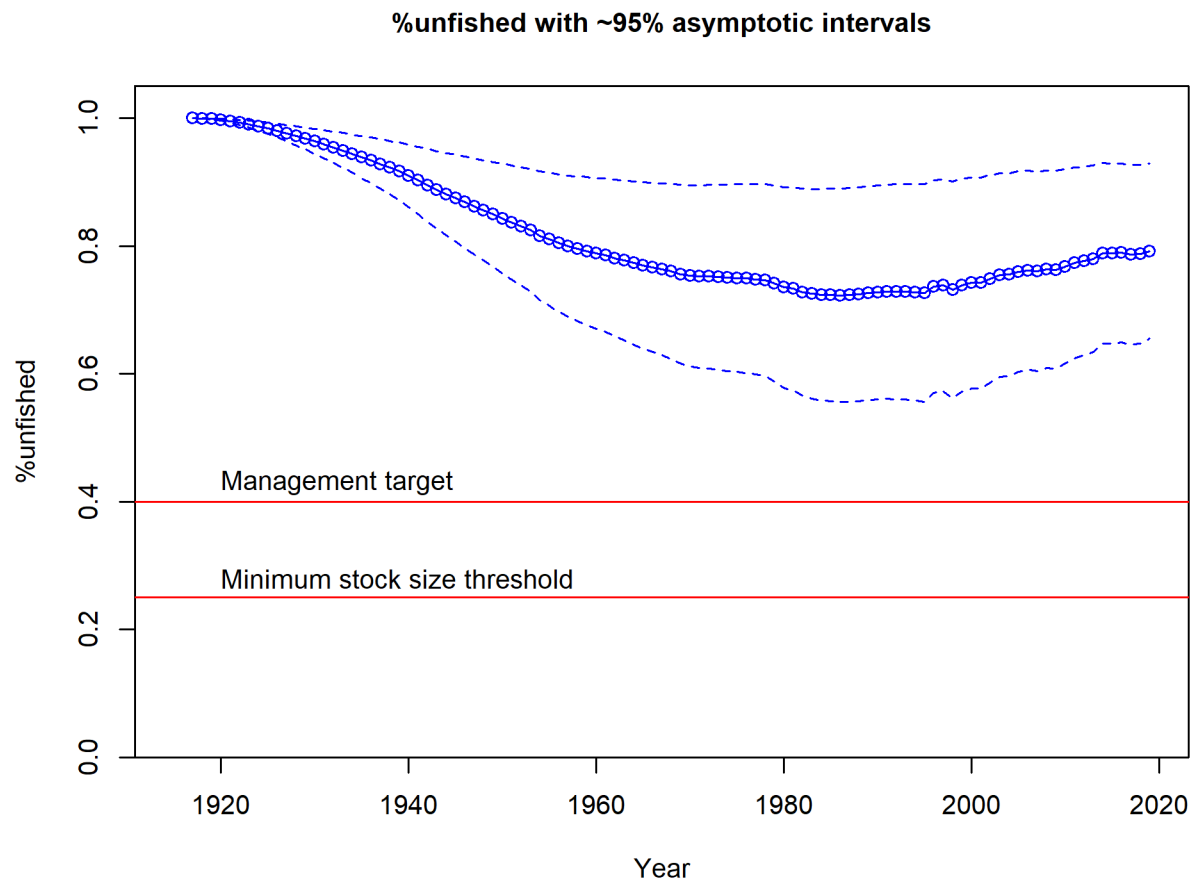
Figure 45: Estimated %unfished with approximate 95% asymptotic intervals.
