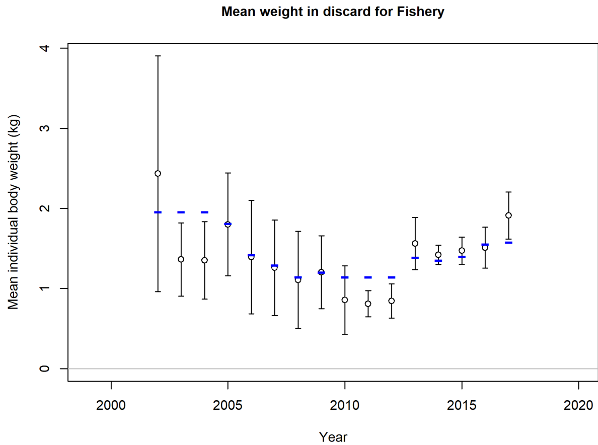
Figure 43: Fit to the mean weight of the discards. Points are model estimates with 95% uncertainty intervals. The model estimate is shown in the blue lines.
