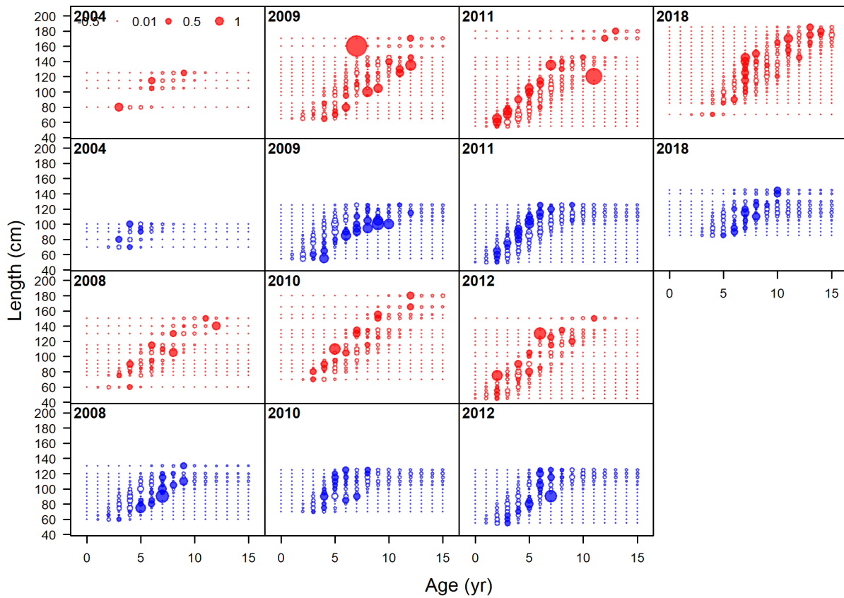
Figure 38: Pearson residuals for the fit to conditional age-at-length data from the fishery. Closed bubbles are positive residuals (observed > expected) and open bubbles are negative residuals (observed < expected).
