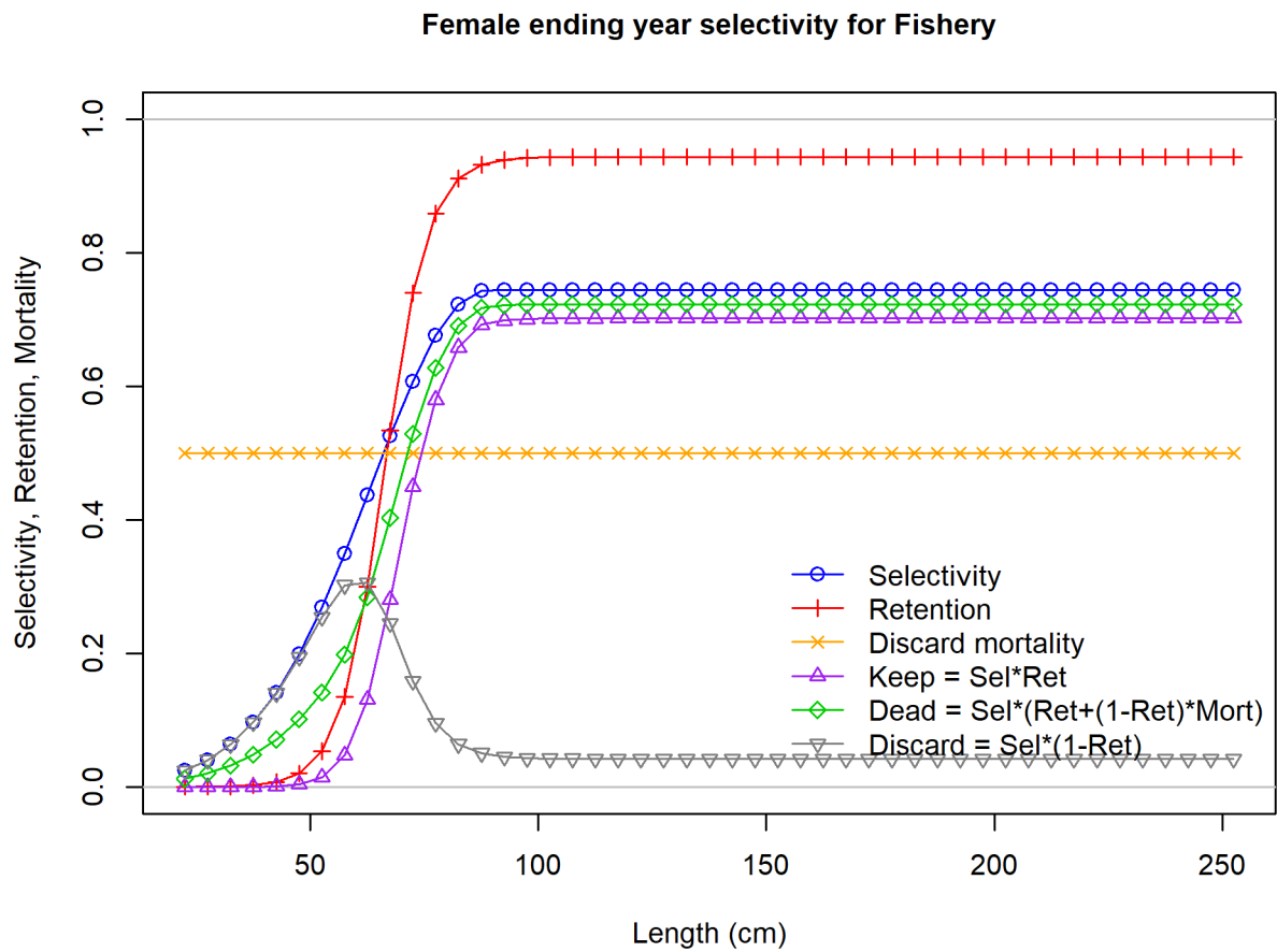
Figure 32: Female fishery selectivity and retention in 2018 with associated derived quantities.
