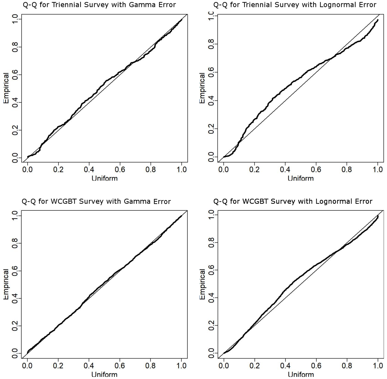
Figure 9: Quantile-quantile (Q-Q) plot showing empirical quantiles of the positive catch rate relative to their expected theoretical quantiles within the VAST geostatistical standardization for the two surveys with both Gamma and Lognormal error structures.
