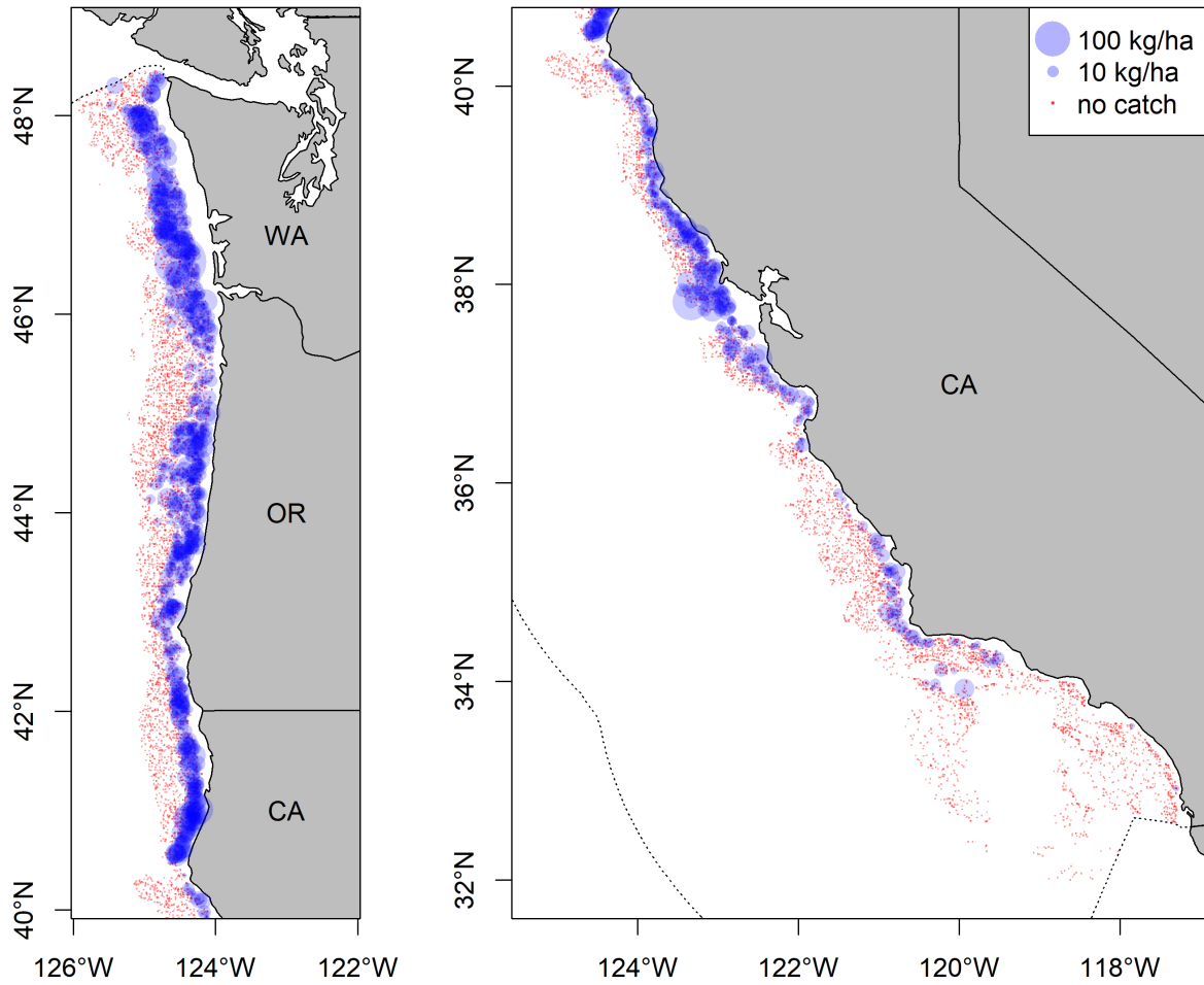
Figure 7: Map showing the distribution of Big Skate within the area covered by the West Coast Groundfish Bottom Trawl Survey aggregated over the years 2003–2018.
