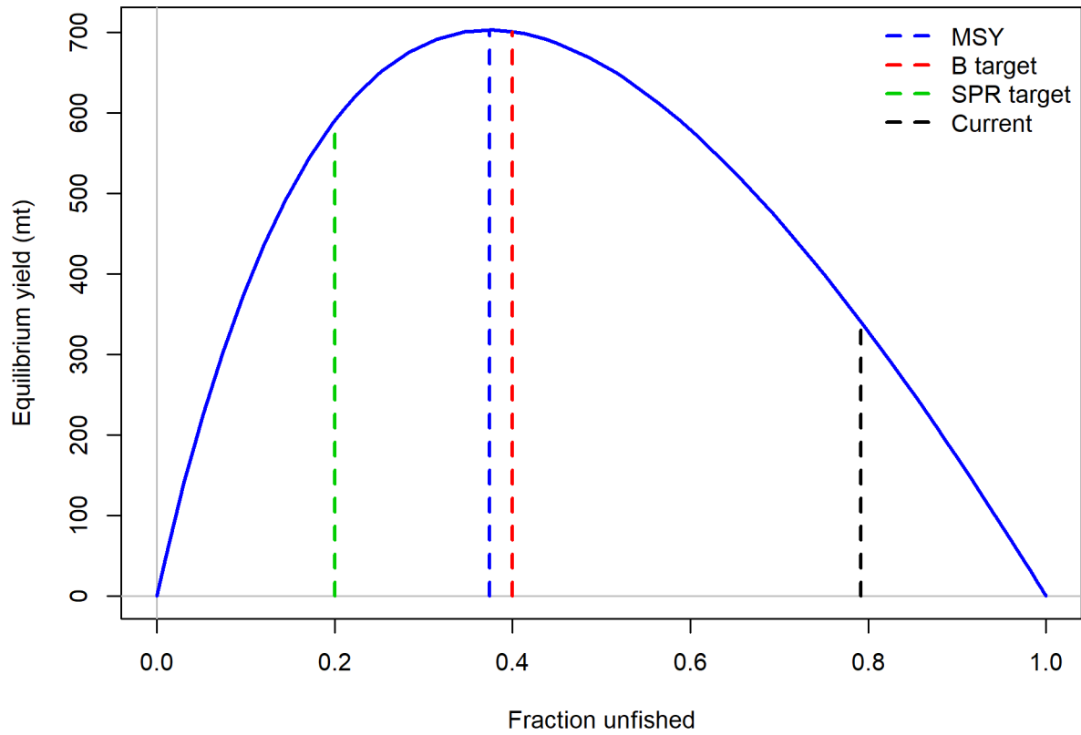
Figure 69: Equilibrium yield curve for the base case model. Values are based on the fishery selectivity and with steepness fixed at 0.4.
