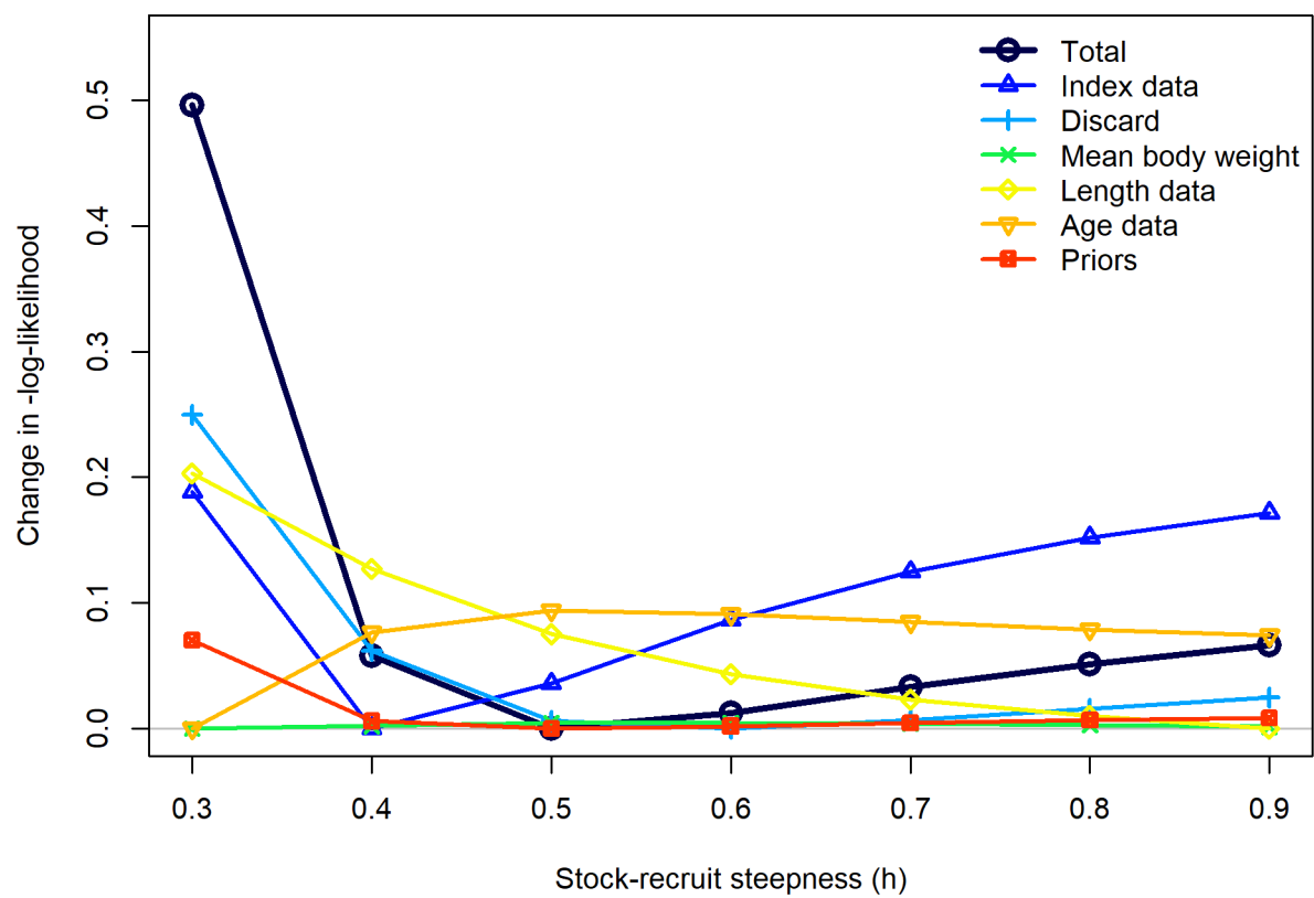
Figure 65: Likelihood profile over stock-recruit steepness ( h ).
