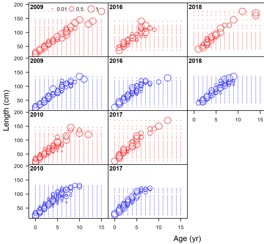
Figure 24: Conditional age-at-length data from the WCGBT Survey.
