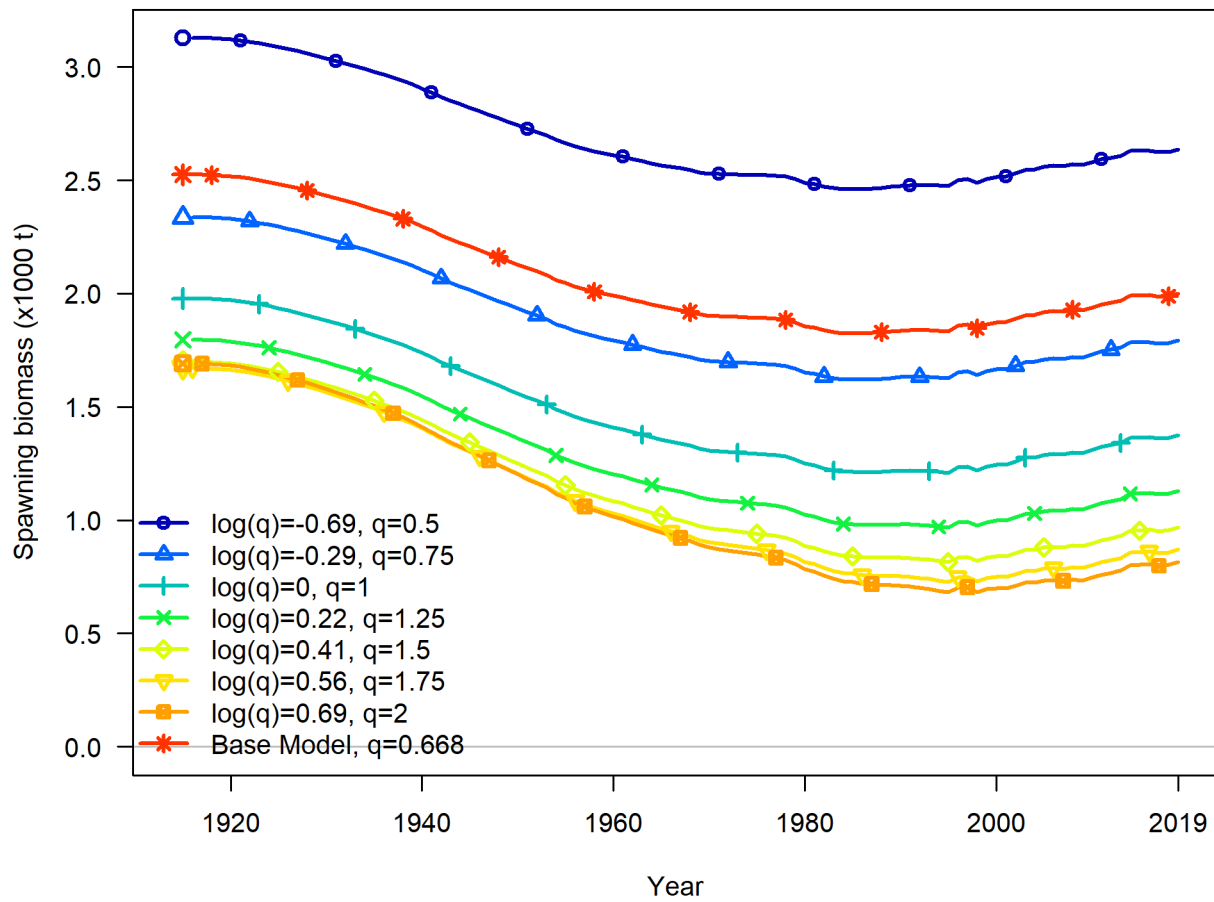
Figure 64: Time series of spawning biomass (mt) estimated for the models included in the profile over the catchability of the WCGBT Survey ( q ).
