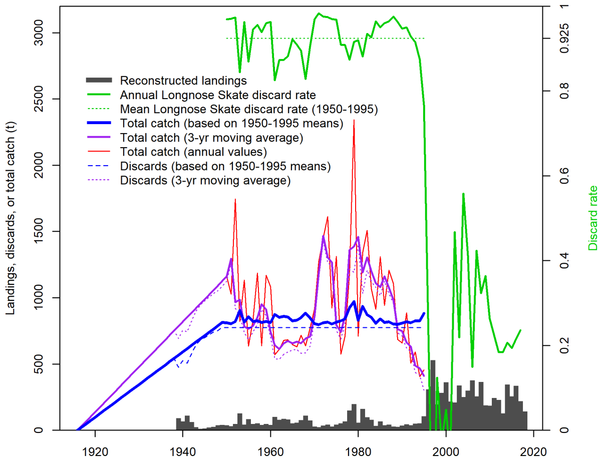
Figure 4: Estimated total catch using different assumptions for discards. The discard rates shown in green lines are relative to the right-hand axis while all other values are relative to the left-hand axis.
