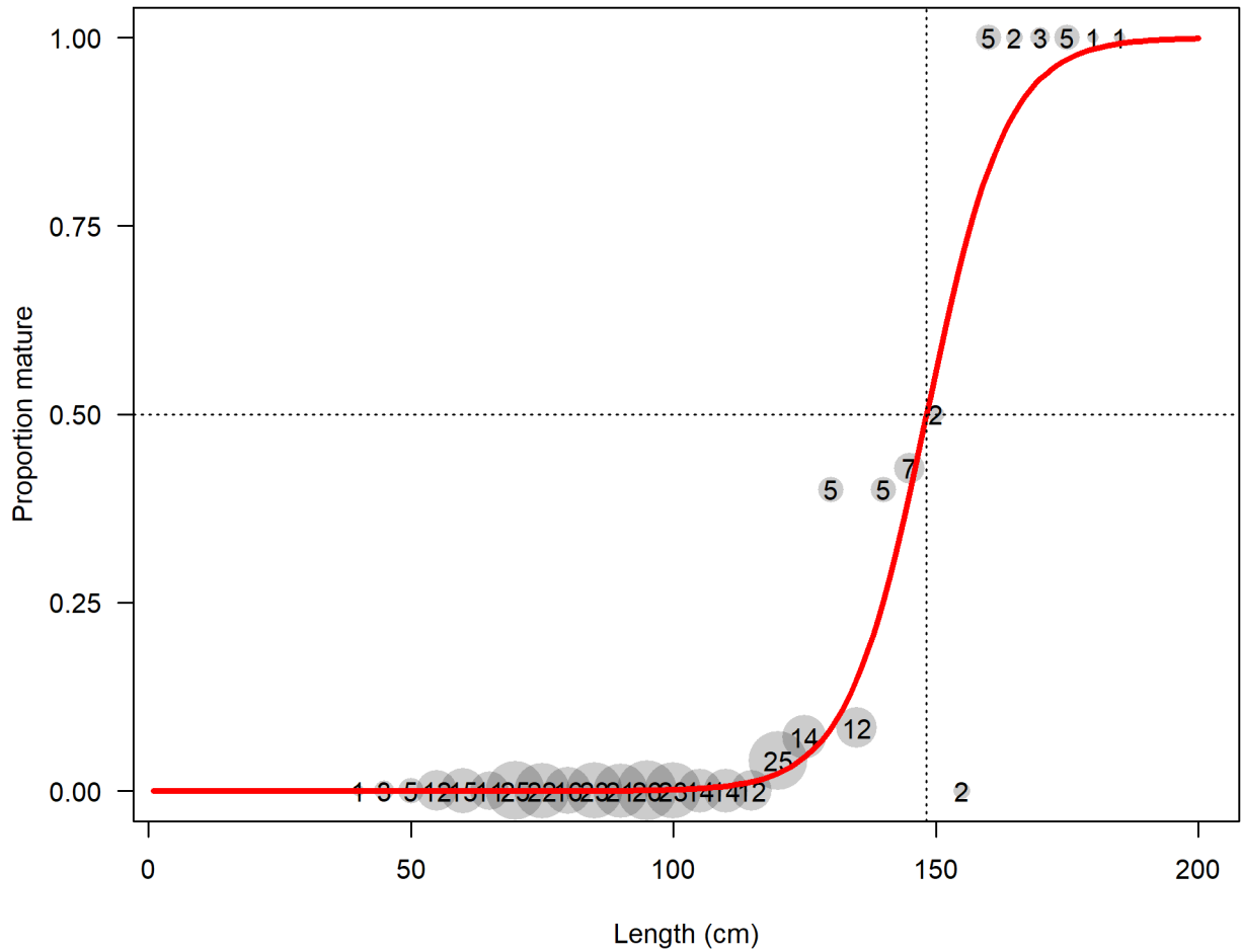
Figure 27: Estimated maturity relationship for female Big Skate. Gray points indicate average observed functional maturity within each length bin with point size proportional to the number of samples (indicated by text within each point).
