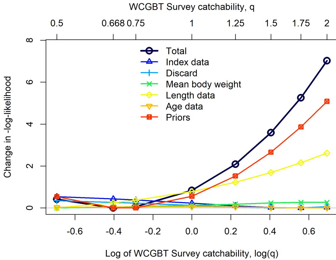
Figure 63: Likelihood profile over the catchability of the WCGBT survey ( q ) including the prior likelihood contribution.
