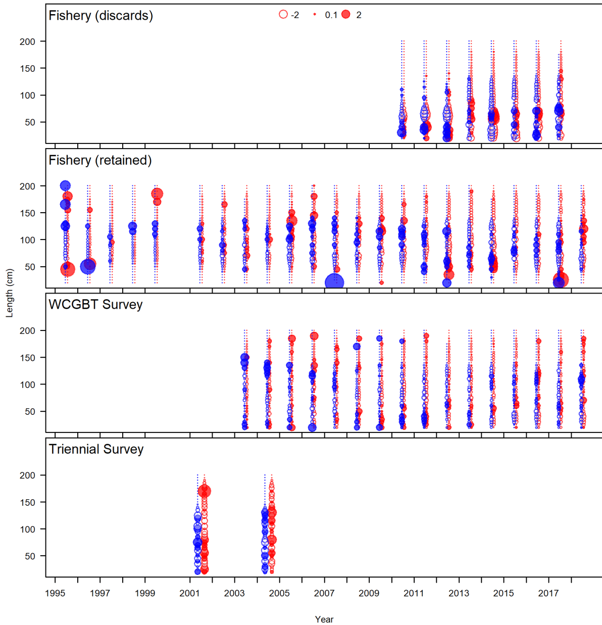
Figure 37: Pearson residuals for length composition data for all years and fleets, with females in red and males in blue. Closed bubbles are positive residuals (observed > expected) and open bubbles are negative residuals (observed < expected).
