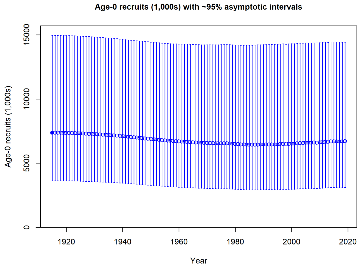
Figure 46: Estimated time-series of recruitment for Big Skate.
