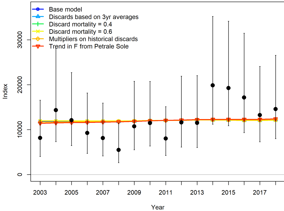
Figure 54: Fit to the WCGBT Survey estimated in the sensitivity analyses related to historic catch and discards.
