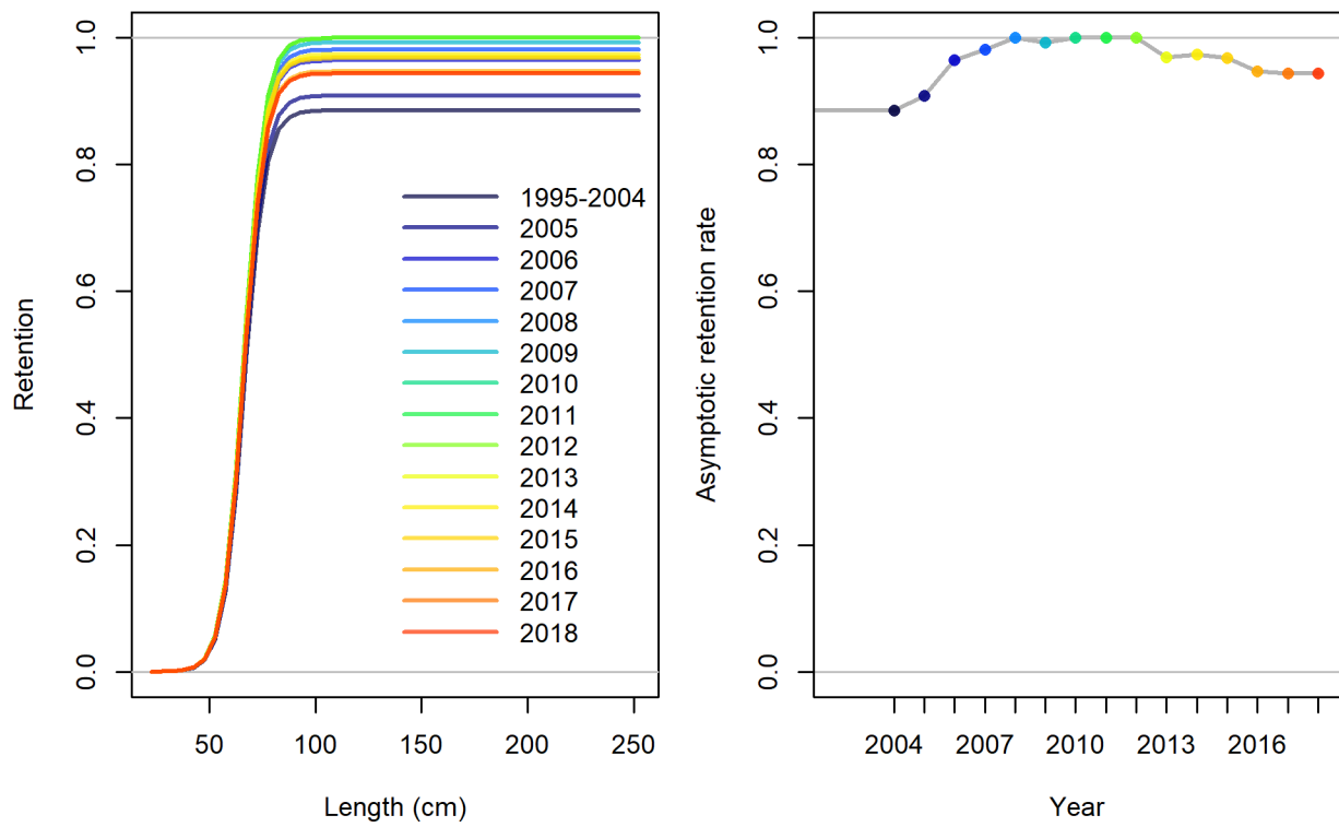
Figure 33: Time-varying retention for the fishery (left) with the time-series of asymptotic retention rates (right).
