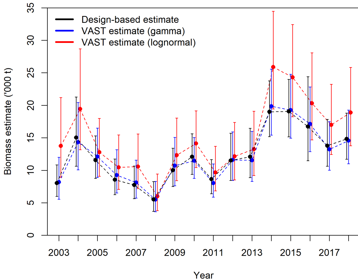
Figure 11: Index of abundance from the WCGBT Survey calculated as a design-based index and using the VAST geostatistical analysis with alternative error structures. Details on the alternative calculations are provided in the text.
