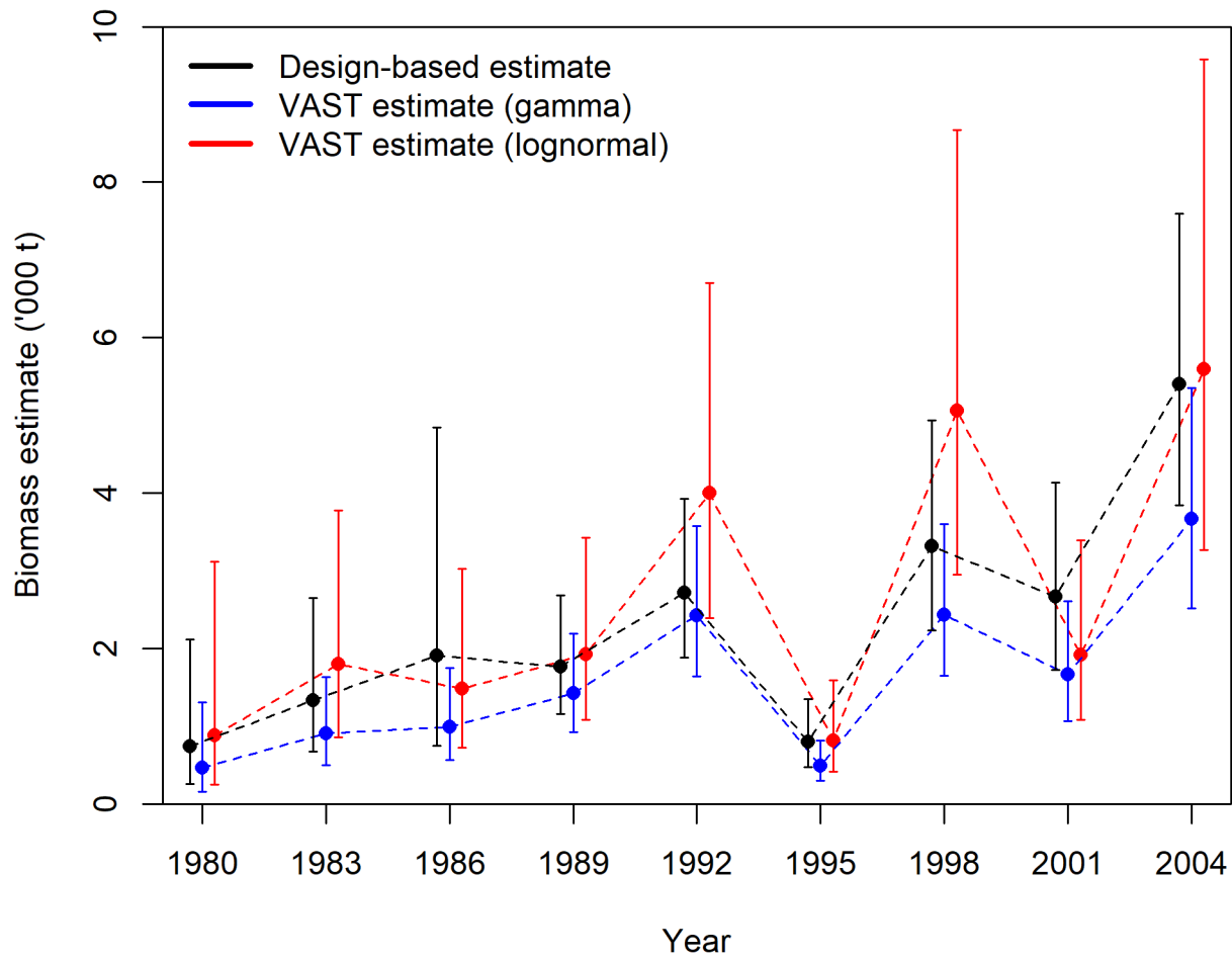
Figure 10: Index of abundance from the Triennial Survey calculated as a design-based index and using the VAST geostatistical analysis with alternative error structures. Details on the alternative calculations are provided in the text.
