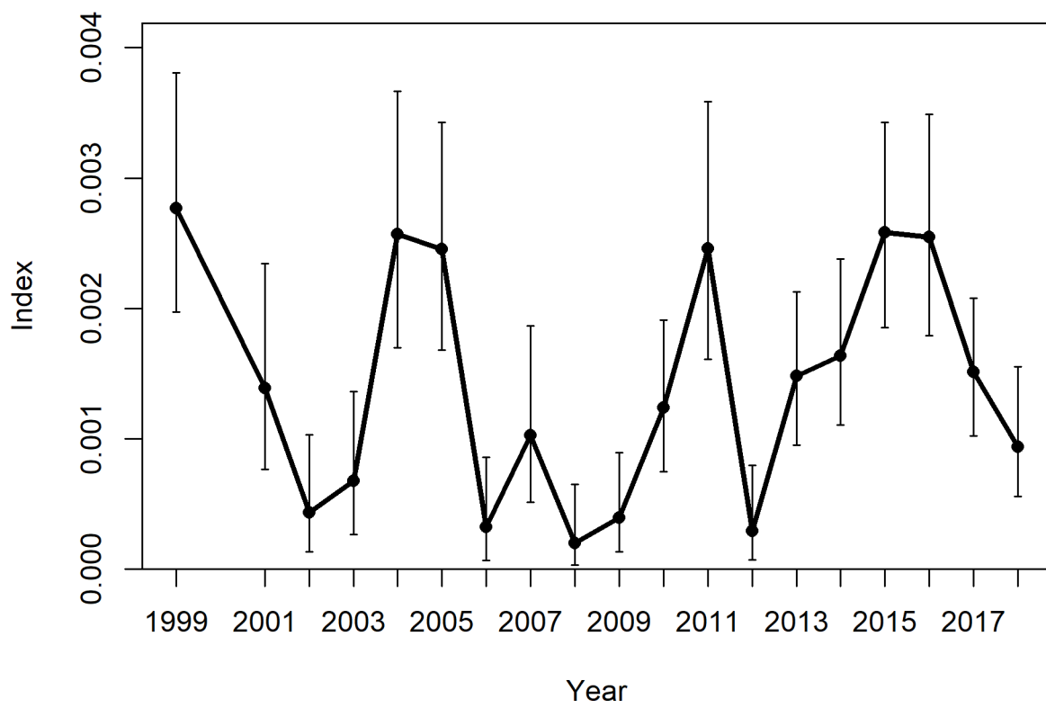
Figure 12: Index of abundance from the International Pacific Halibut Commission longline survey (not used in the assessment model).
