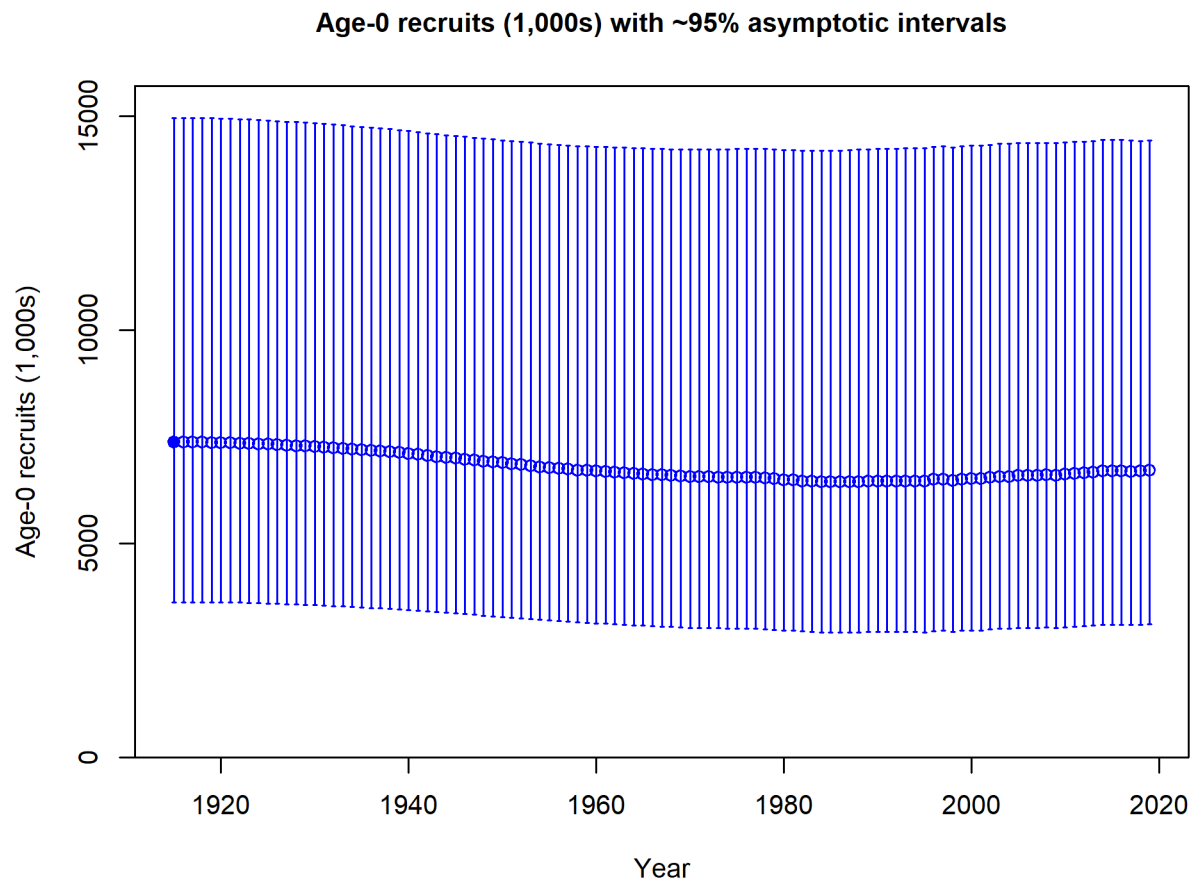
Figure d: Time series of estimated Big Skate recruitments for the base-case model with 95% confidence or credibility intervals.
