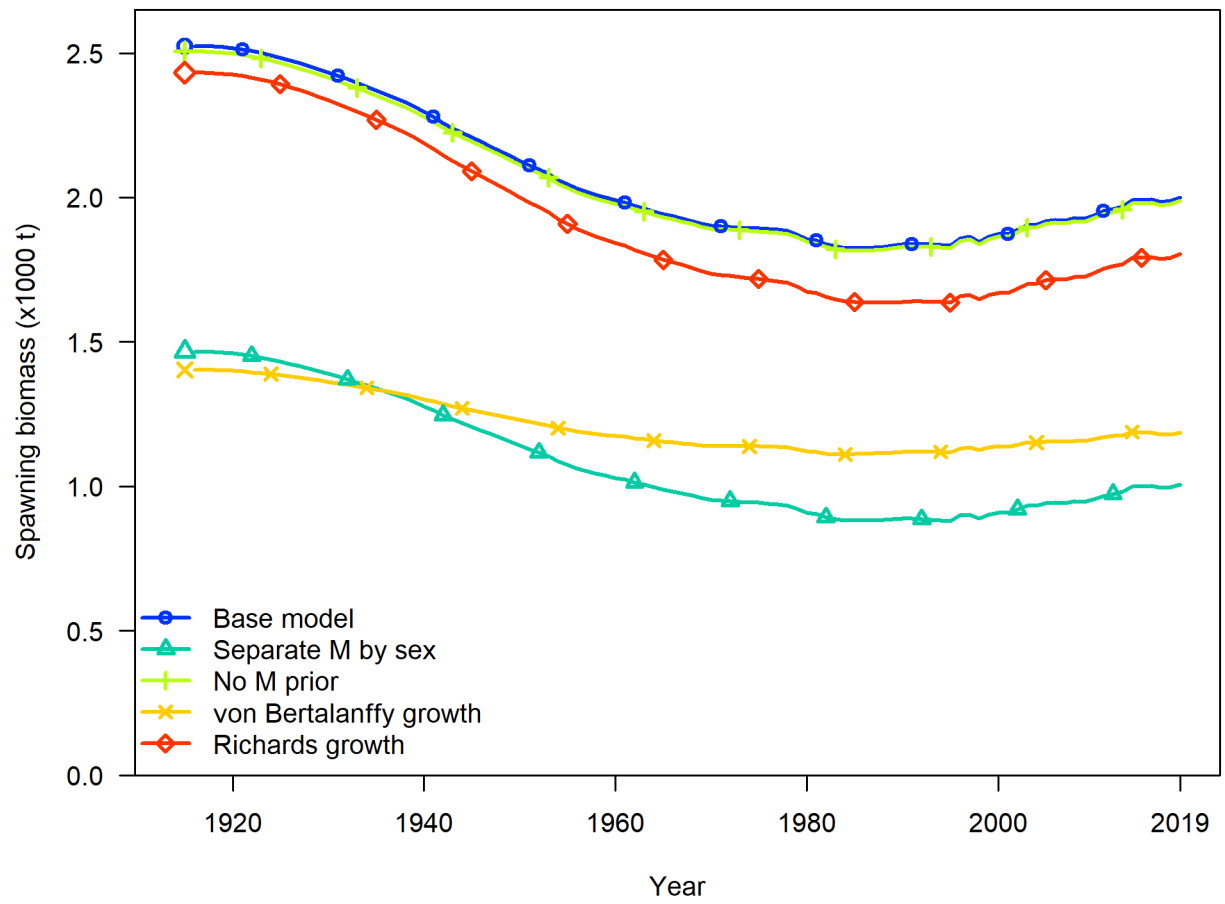
Figure 49: Time series of spawning biomass (mt) estimated in sensitivity analyses related to biology.
