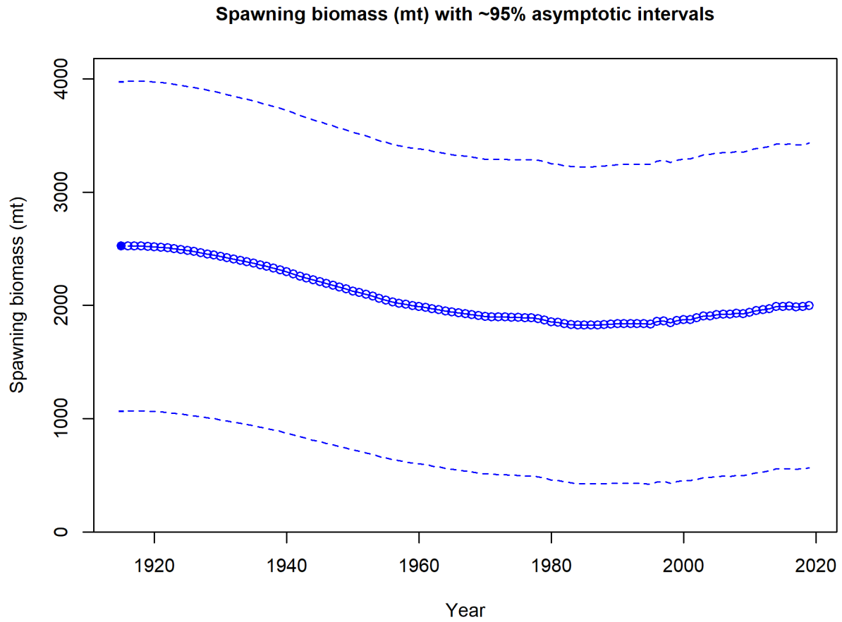
Figure 44: Estimated spawning biomass (mt) with approximate 95% asymptotic intervals.
