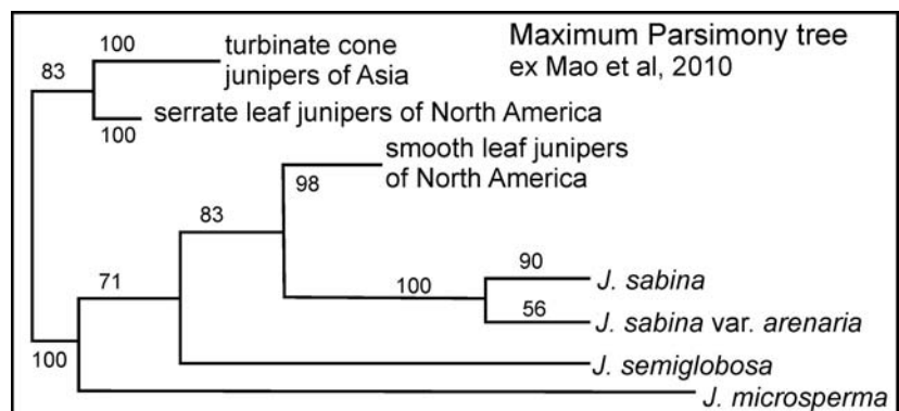
Figure 1. A maximum parsimony tree showing the clade with J. microsperma , J. sabina and smooth leaf junipers of North America. the numbers at the branch points are bootstrap support values (adapted from Mao et al., 2010).
