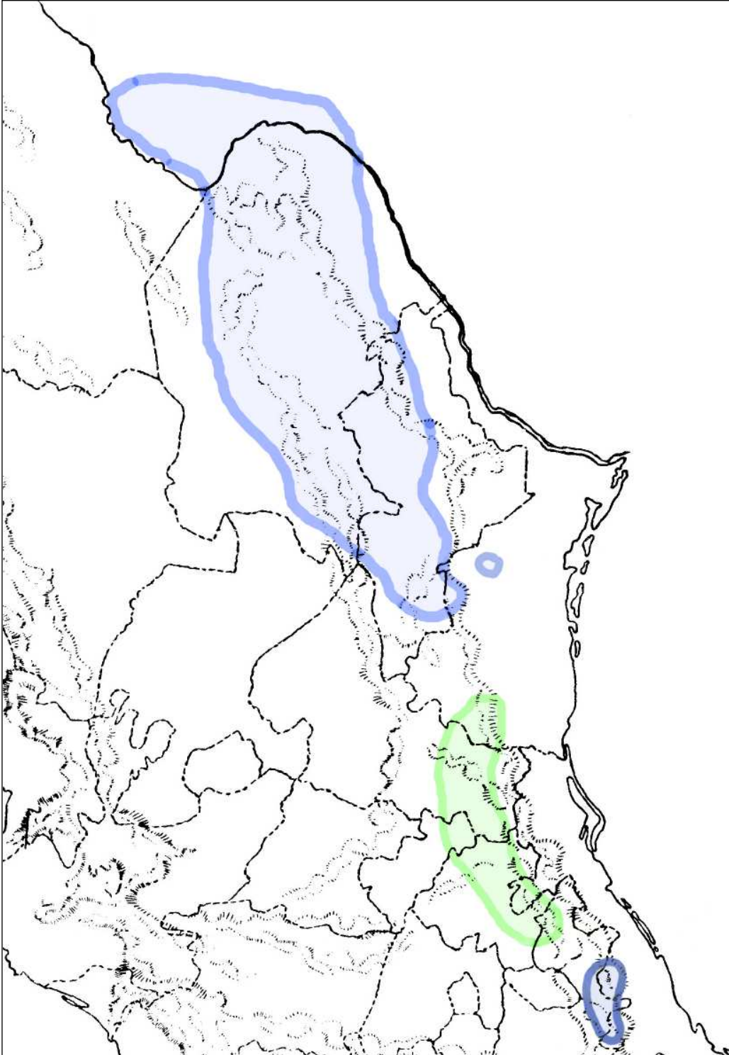
Map 1. General range outlines of Mimophytum (green) and North American Omphalodes (blue).
