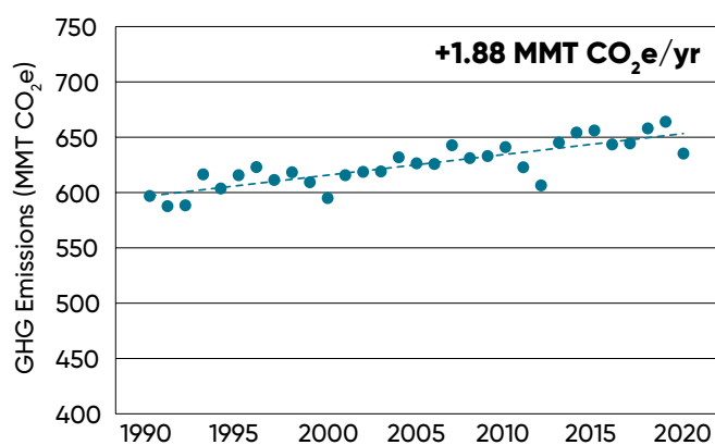
Figure 3. Recent trend in greenhouse gas emissions from the U.S. agriculture sector, 1990–2020. Source: EPA Inventory of U.S. Greenhouse Gas Emissions and Sinks 1990–2019.
