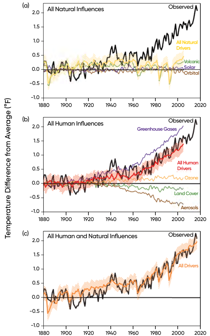
Figure 4. Human and natural influences on global temperature, 1880–2018 (Hayhoe, et al., 2018).
