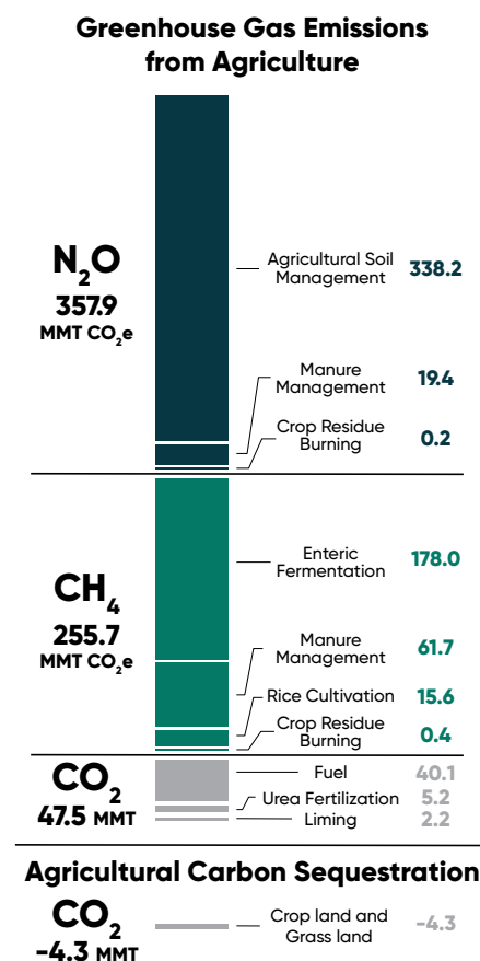
Figure 1. Greenhouse gas emissions from agriculture and sequestration in crop and grass land in the U.S., 2018. Source: EPA Inventory of U.S. Greenhouse Gas Emissions and Sinks 1990-2019.
