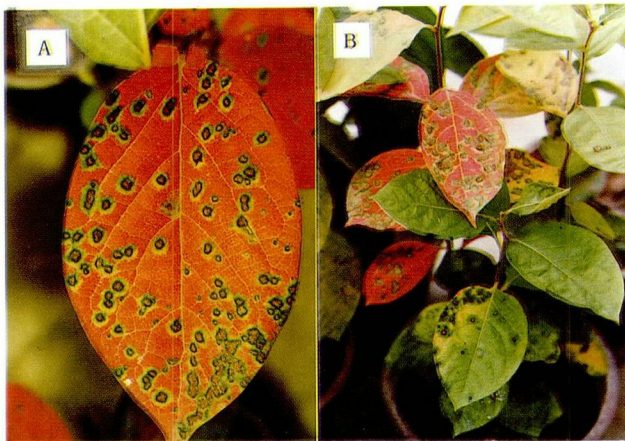
Fig. 3. Various symptoms of circular leaf spot disease of persimmon. A: Typical symptom, B: Symptom induced by conidia inoculation produced in PDA medium.
