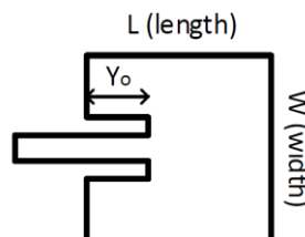
Patch Antenna Inset Feeding
