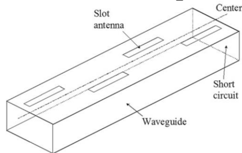
Slotted waveguide array antenna
