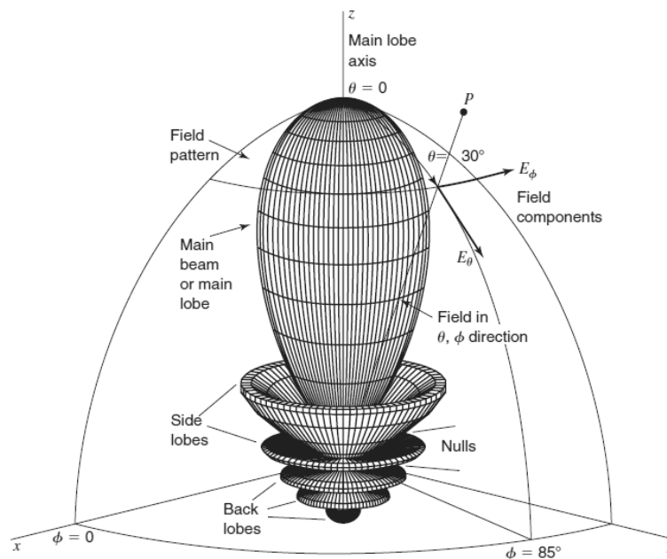
Antenna fields pattern in 3D coordinates
