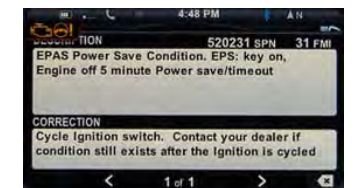
Diagnostics screen displays fault codes and suggested actions to take
