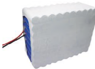
12,8V 4S20P • 182x146x68mm • c/ placa PCM MOD 8 036201 - 3000mAh
