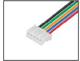
PHR5 • 30cm 036383 - 22AWG 036384 - 26AWG
