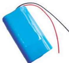
7,4V 2S1P • 38x20x68mm • c/ placa PCM MOD 1 036165 - 2200mAh 036166 - 2600mAh 036167 - 3000mAh
