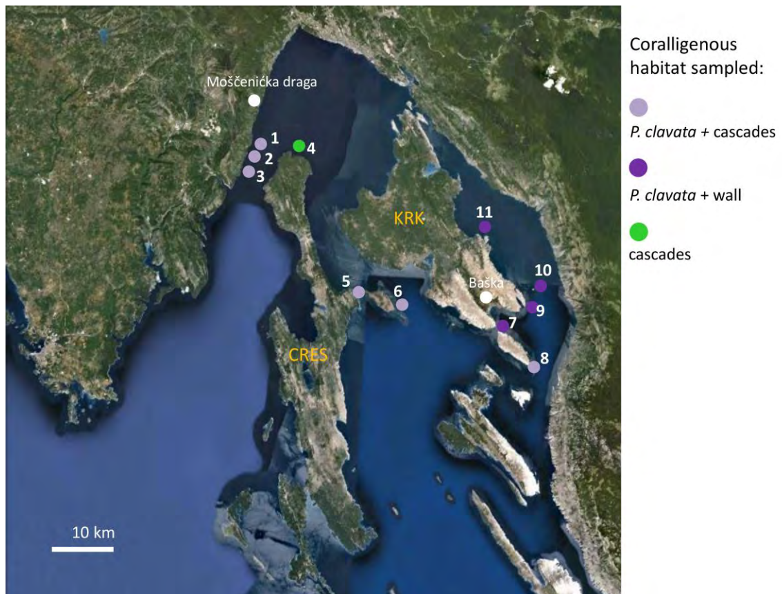
Fig. 2.6. Study sites of coralligenous habitat within Primorje-Gorski Kotar County (North Adriatic): 1 = Cape Kinkela; 2 = Cape Lonjica; 3 = Cape Stupova; 4 = Cape Jablanac; 5 = Plavnik; 6 = Mali Plavnik; 7 = Cape Stražica; 8 = Cape Šilo; 9 = Cape Sokol; 10 = Zečevo; 11 = Tenki. Characteristics of study sites are summarized in Table 2.1. More detailed maps and the overview of sites that have been assessed for the first time are provided in the Section 4. Map source: Google Earth, Image © 2014 DigitalGlobe.
