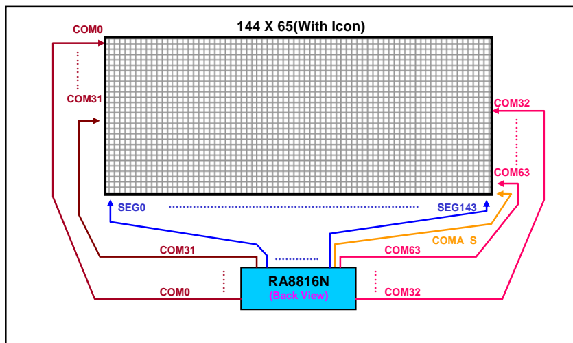
圖 A-5 : The Connection of RA8816N with LCD Panel (144x65)
