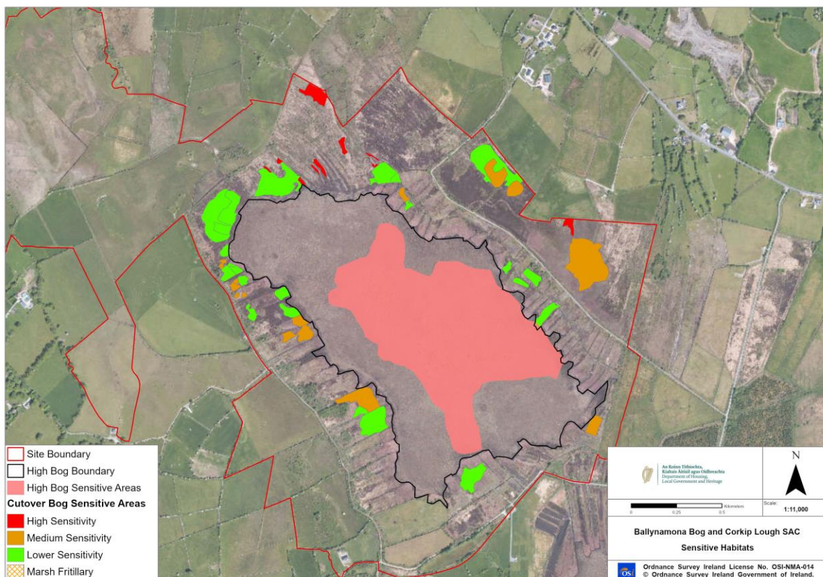
Figure 4.2 Sensitive habitats mapped at Ballynamona Bog SAC
