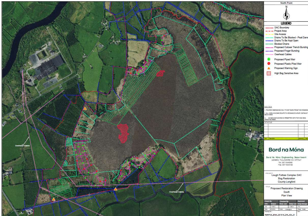
Figure 5.4 Contract Drawing of proposed Restoration Works at Fisherstown Bog
