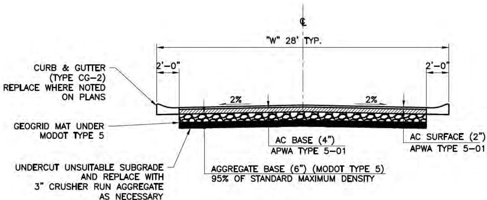
TYPICAL STREET SECTION
