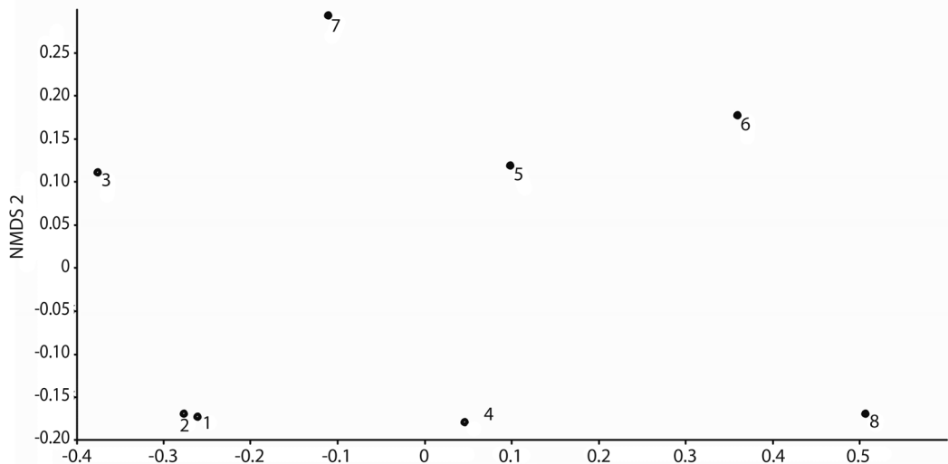
Fig. 1. Similarity among climber using non-metric multidimensional scaling (NMDS) ordination in plots in cerradão and Seasonal Deciduous Forest in the Serra de Maracaju, Mato Grosso do Sul, Brazil. Plots 1-4: Seasonal Deciduous Forest; plots 5-8: cerradão (number of dimensions k=2 ).
