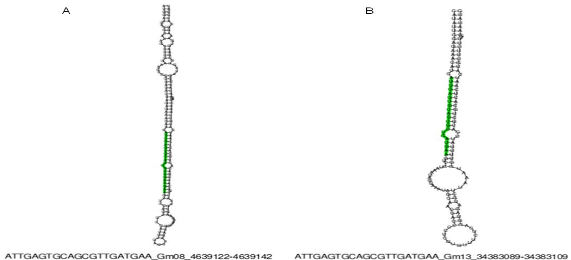
Figure 2. Secondary structure bioinformatically predicted of pre-miRNAs for sequence for four (miR397-5p). In green the miRNA sequence identified is shown. A) Location of chromosome eight of Glycine max . B) Location of chromosome 13 of Glycine max
