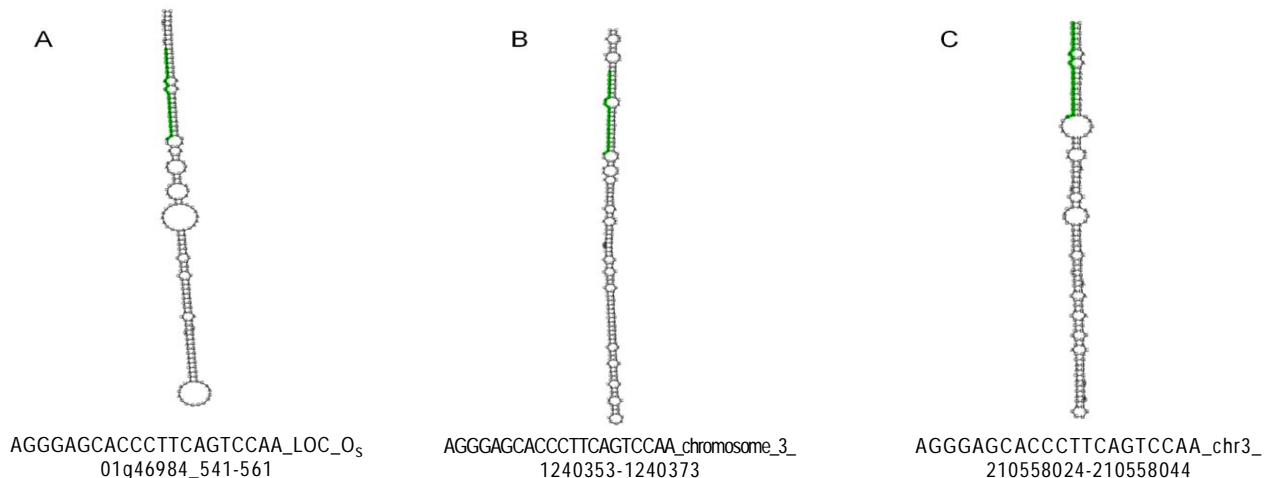
Figure 1. Secondary structure bioinformatically predicted of pre-miRNAs for sequence two (miR319-3p). Green indicates the miRNA sequence identified. A) Location of chromosome one of Oryza sativa . B) Location of chromosome three of Sorghum bicolor . C). Location of chromosome three of Zea mays
