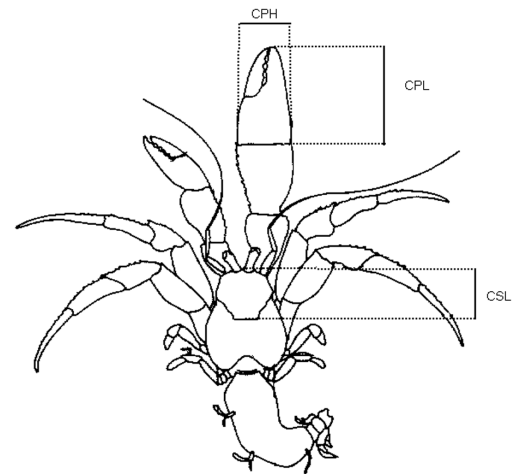
Fig. 1 – General scheme for hermit crab size dimensions (CSL = cephalothoracic shield length; CPL = chelar propodus length; CPH = chelar propodus height) (Modified from Lancaster 1988).
