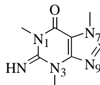
Fig 3. 1,3,7-trimethylguanine
