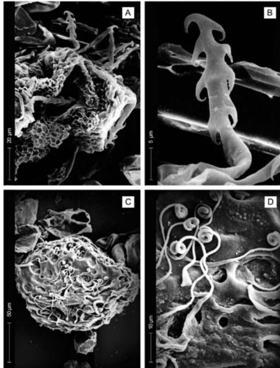
FIGURE 9 | A,B) Azollopsis (Azollopsis) tomentosa HALL, 1968, A: massula and glochidia, B: detail of glochidium [SEM]; C,D) Azollopsis (Spiralopsis) intermedia SWEET and HILLS, 1974, C: massula and glochidia, D: glochidia [SEM].
