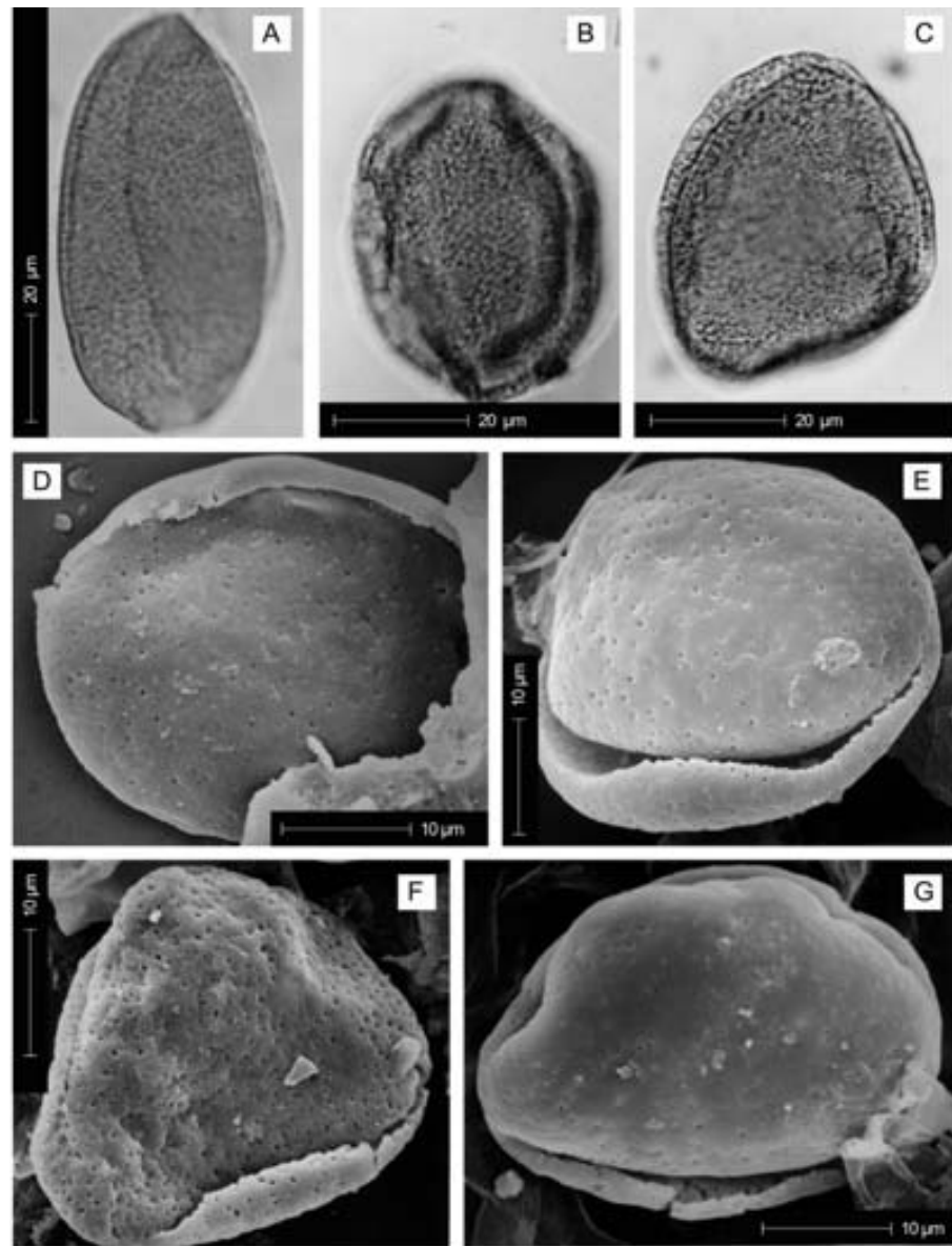
FIGURE 10 | A) Longapertites andreisii ARCHANGELSKY, 1973 [OM]; B) L. patagonicus ARCHANGELSKY, 1973 [OM]; C-G) Proxapertites -group, C: [OM], D-G: [SEM].
