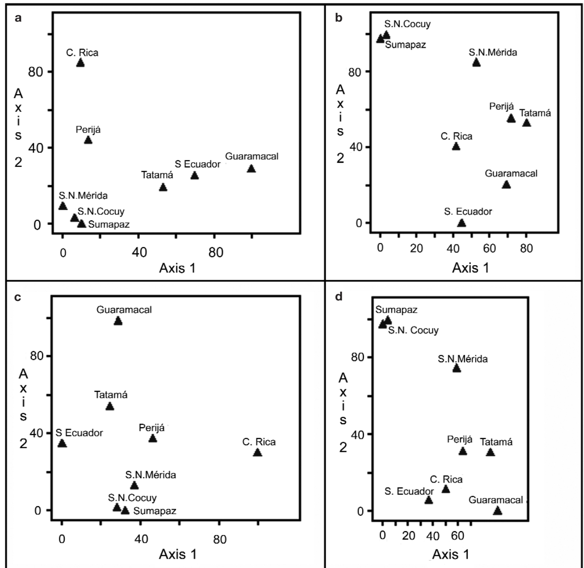
Fig. 4. DCA ( a, c ) and PCA ( b, d ) Ordination diagrams of 404 ( a, b , including páramo & SARF genera from Guaramacal) and 347 ( c, d , including only proper páramo datasets) genera for 8 páramo floras datasets. a , DCA Axis 1 Eig = 0.422; Axis 2 Eig = 0.321; b , PCA Axis 1 Eig = 473.827; Axis 2 Eig = 121.424; c , DCA Axis 1 Eig = 0.223; Axis 2 Eig = 0.189; d , PCA Axis 1 Eig = 803.377; Axis 2 Eig = 87.539.
