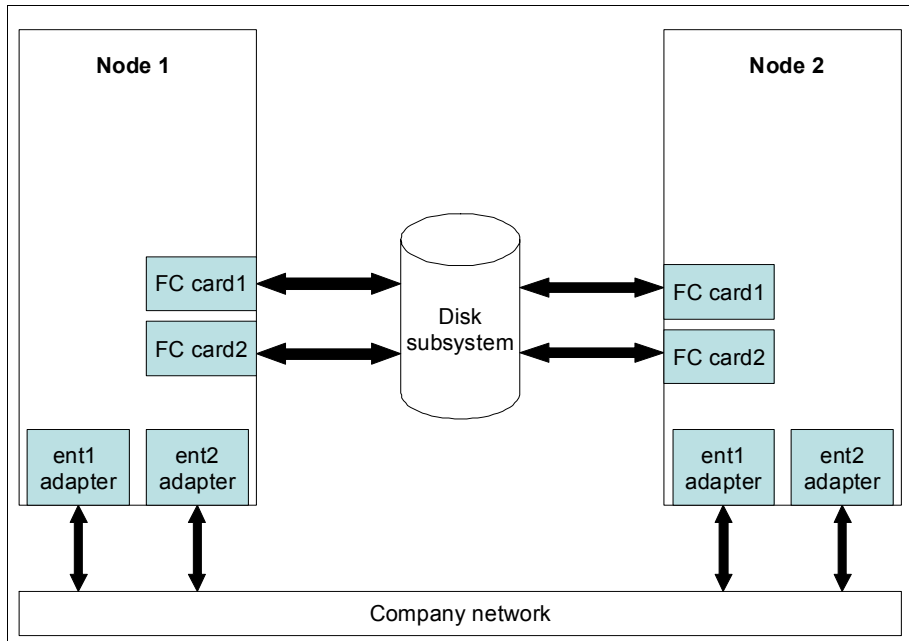
Figure 1-7 Standard 2-node cluster hardware configuration
