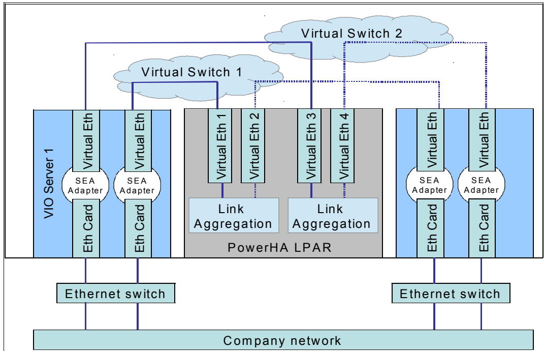
Figure 3-4 NIB with dual Ethernet adapters on the client LPAR
