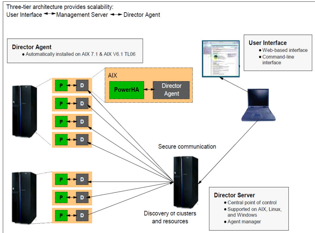
Figure 4-64 System Director architecture that involves the PowerHA plug-in
