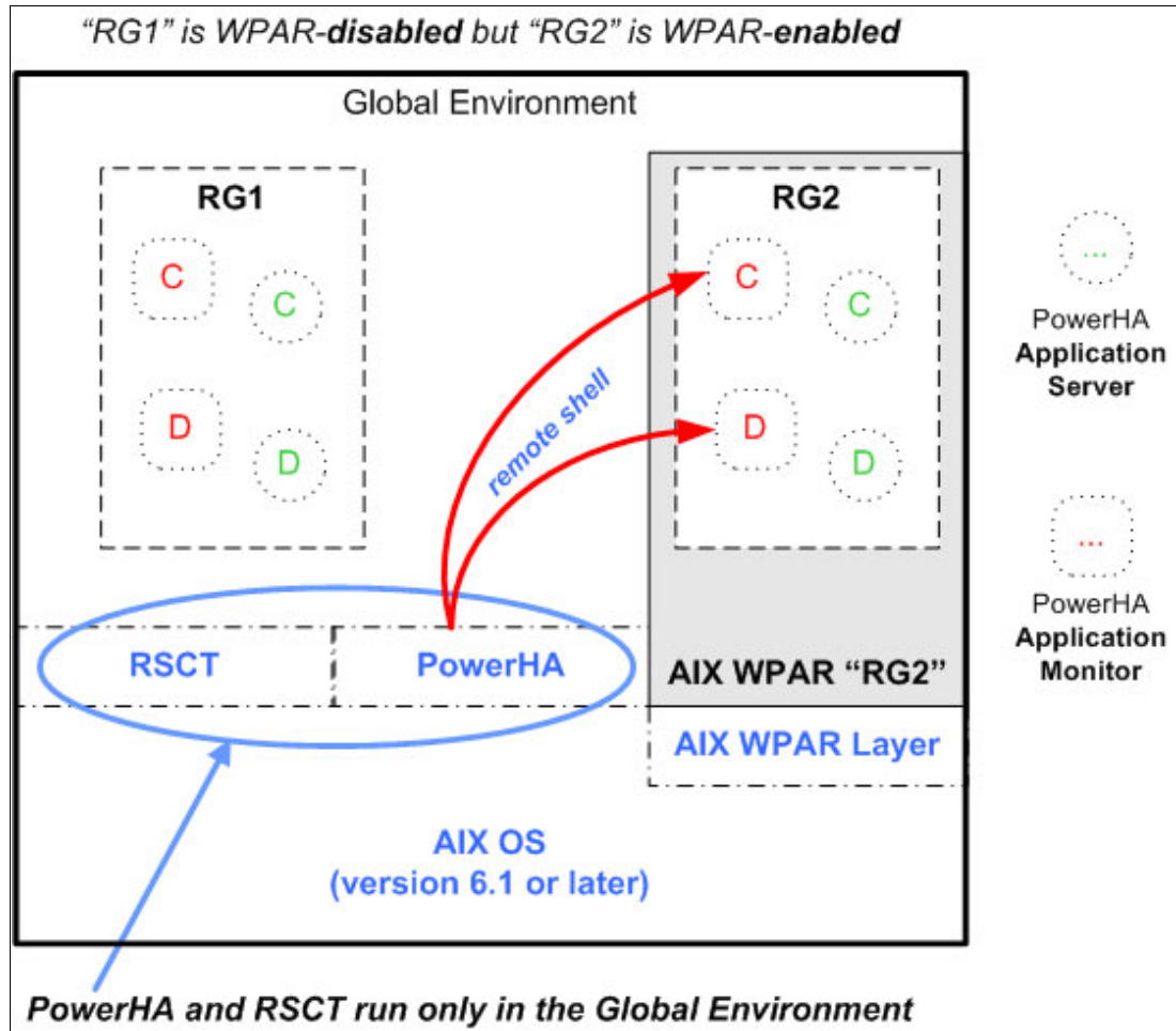
Figure 8-1 PowerHA and WPAR basics
