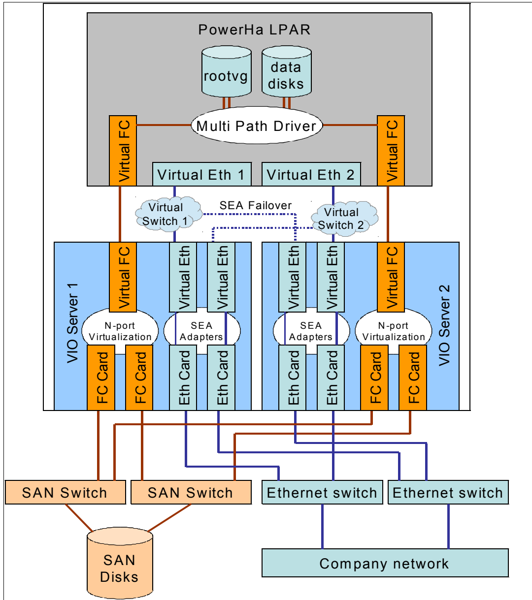
Figure 3-7 Redundant VIOS environment of our sample cluster
