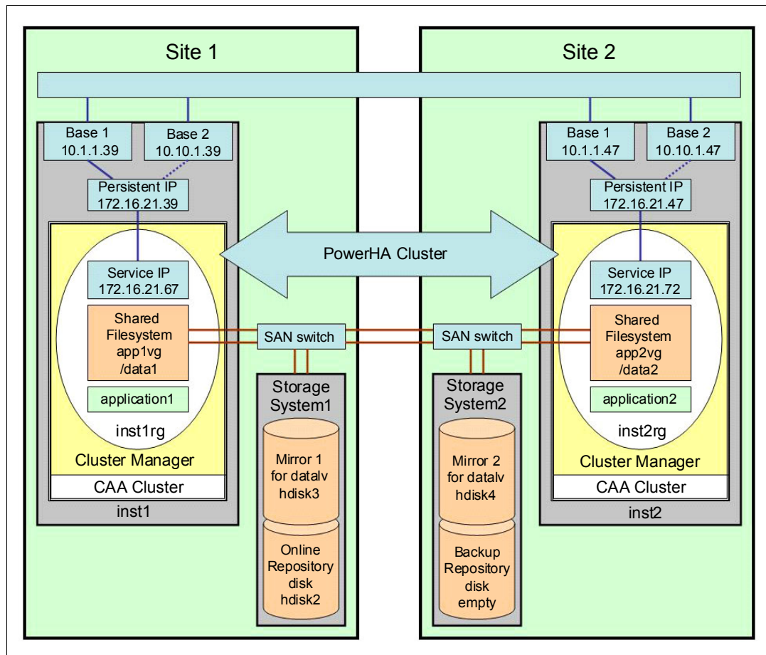
Figure 4-31 Cross-site mirroring solution with PowerHA SystemMirror
