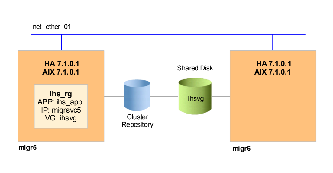
Figure 6-47 Initial cluster configuration
