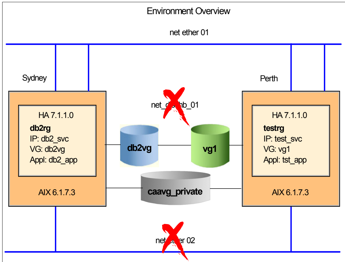
Figure 6-4 Cluster configuration after migration
