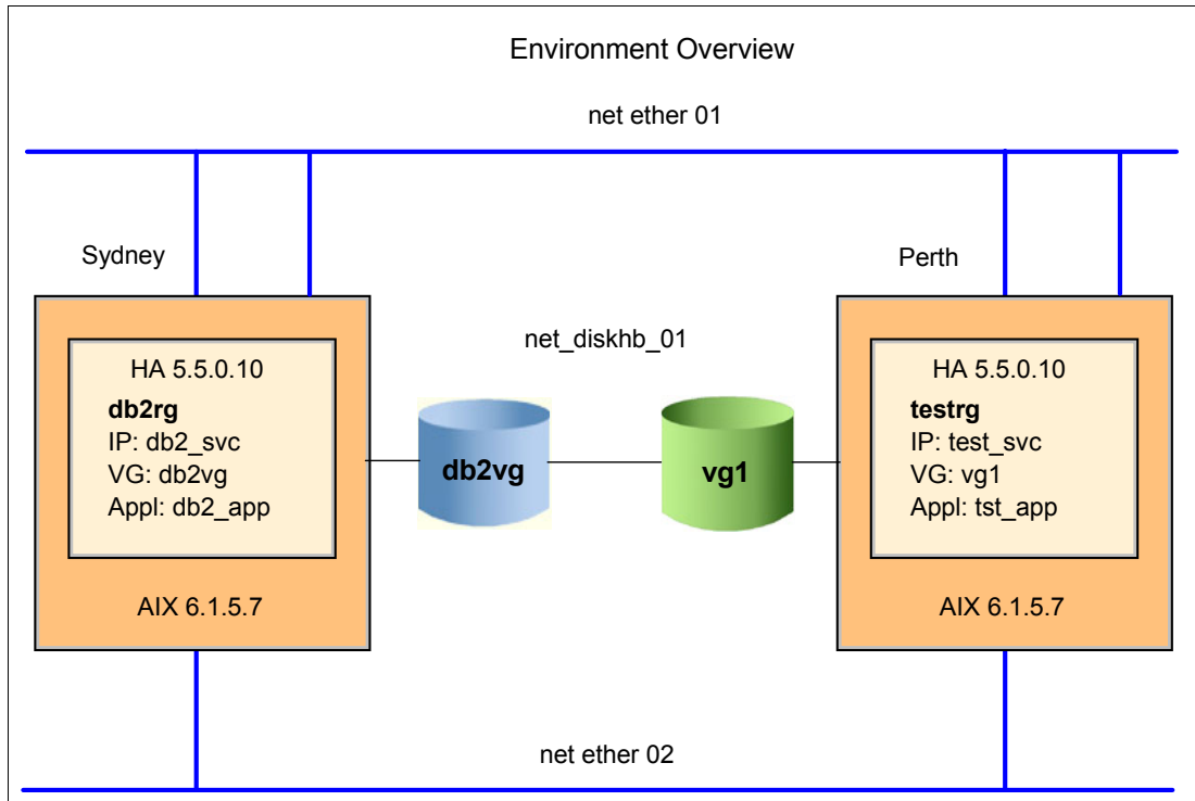
Figure 6-1 Initial cluster configuration
