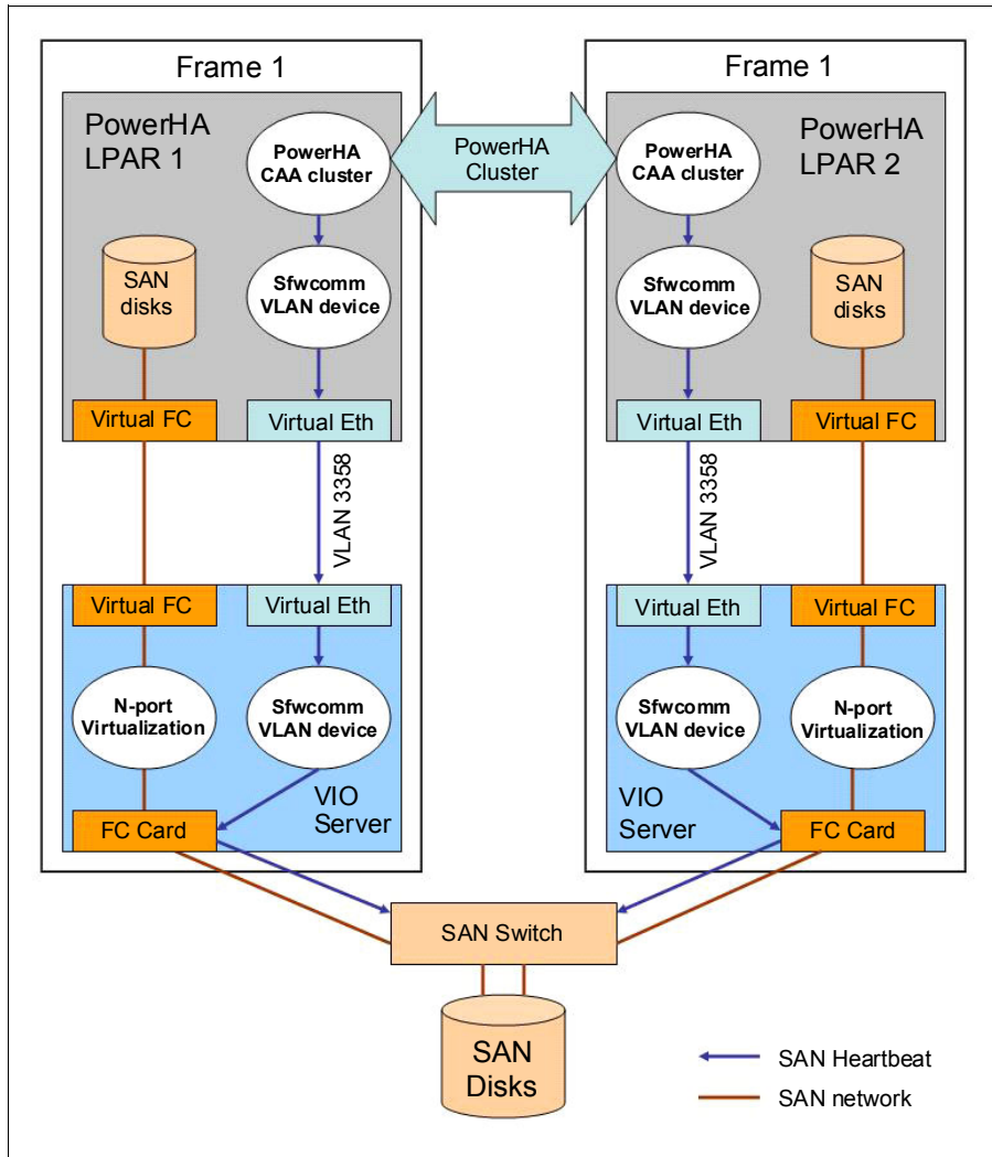
Figure 3-16 SAN heartbeating in a virtual environment
