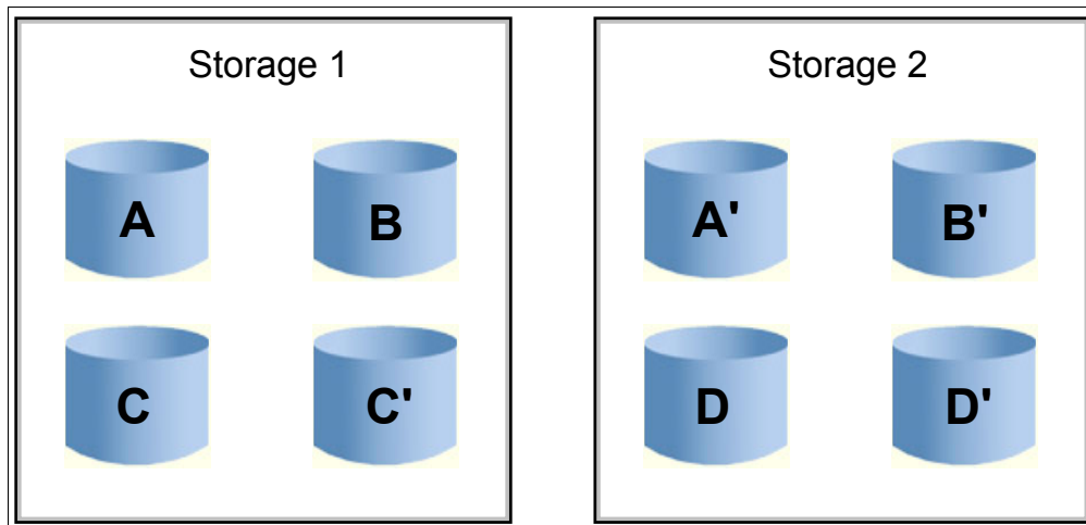
Figure 4-32 LVM mirroring without AIX Mirror Pools
