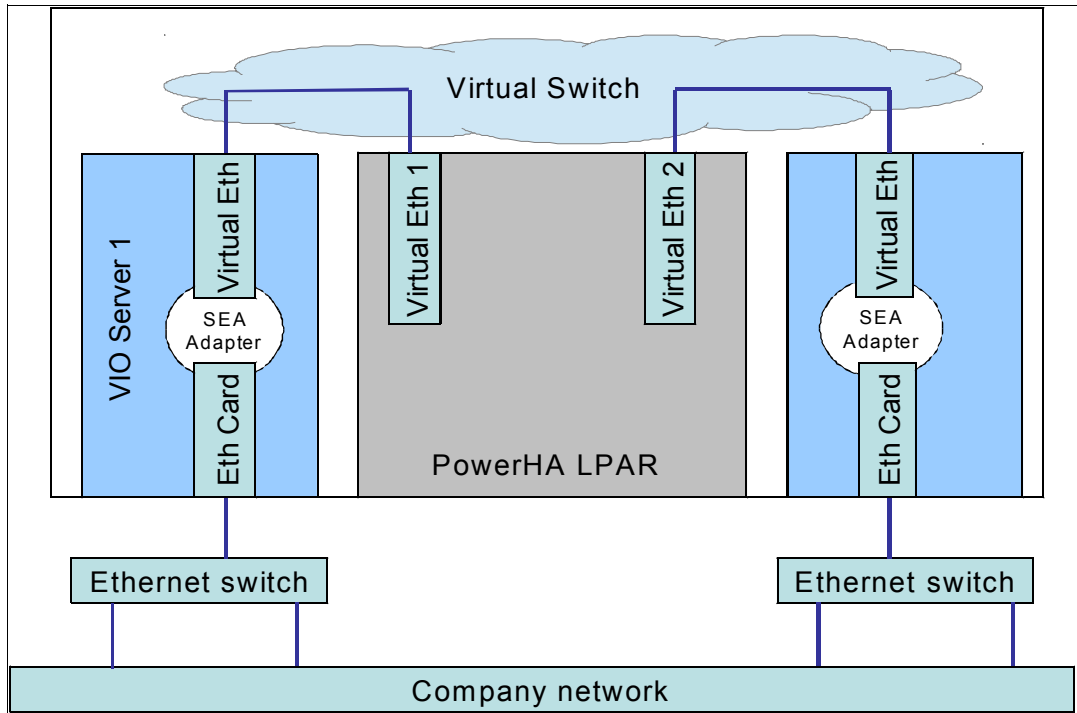
Figure 3-2 Configuration with two virtual Ethernet adapters without SEA failover or NIB
