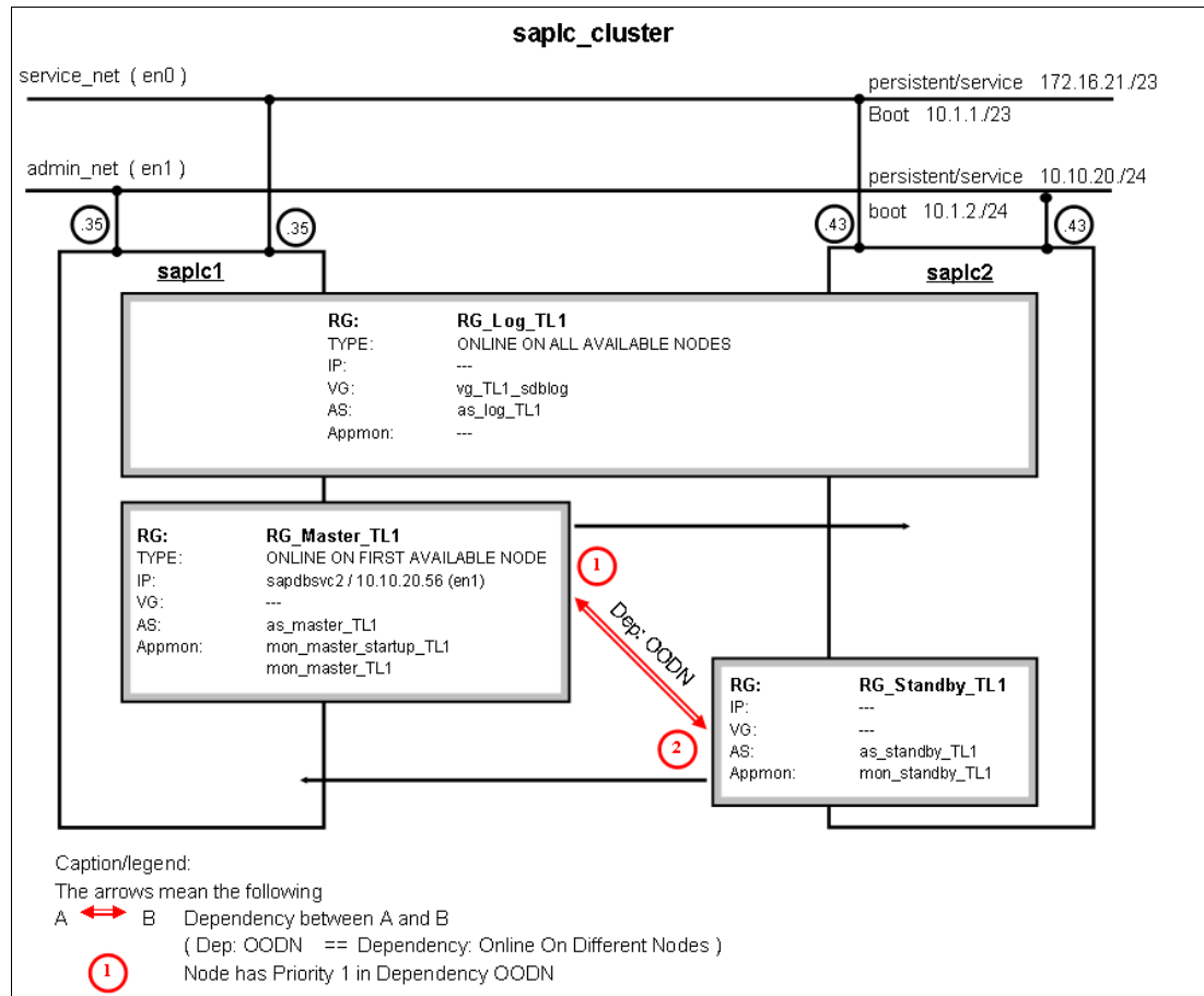
Figure 7-92 Schema overview of saplc_cluster
