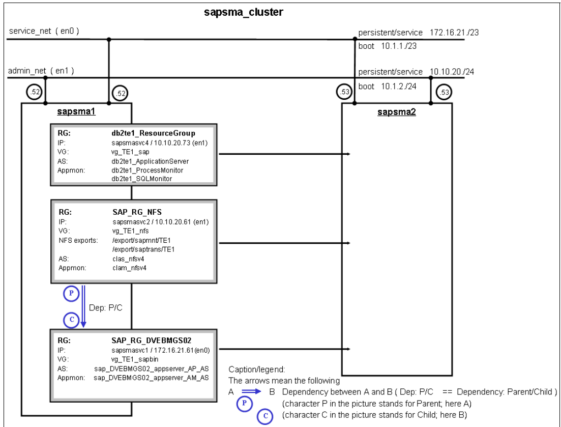
Figure 7-2 Schema overview alternative B for sapsma_cluster
