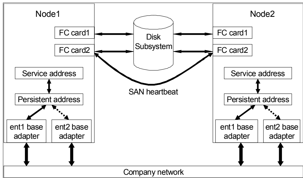
Figure 3-8 Typical cluster network topology
