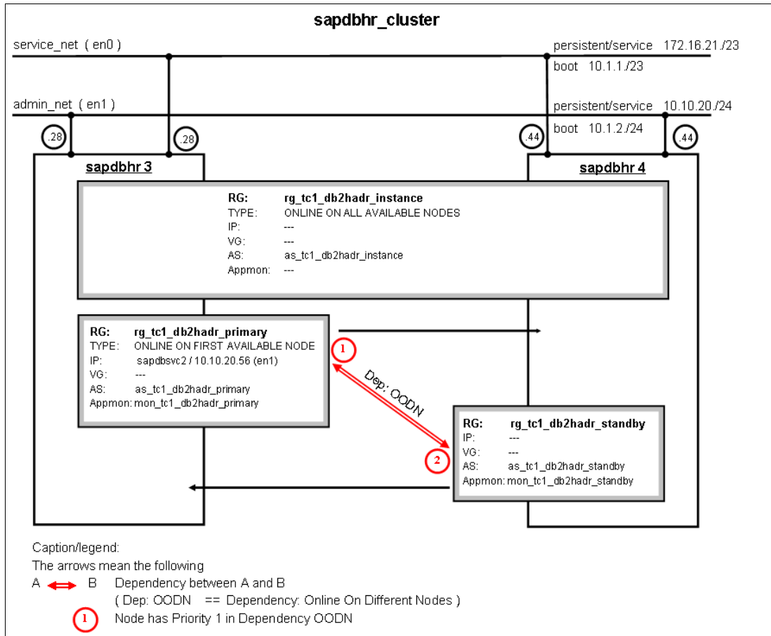
Figure 7-105 Schema overview for sapdbhr_cluster
