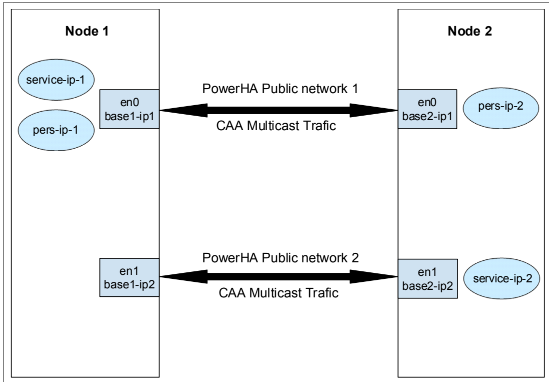
Figure 2-15 Two-node cluster with two defined networks
