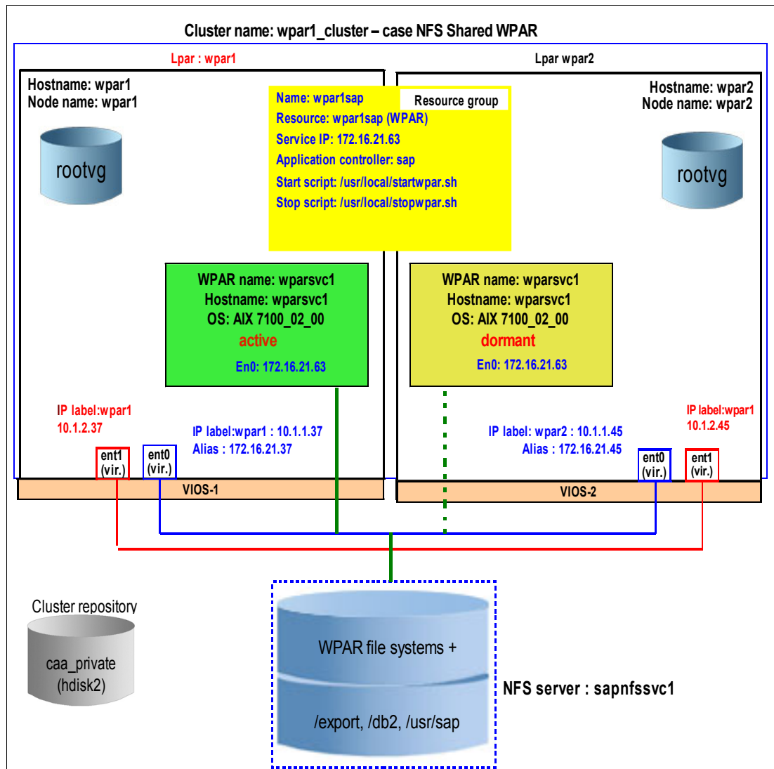
Figure 8-11 Configuration with an NFS WPAR
