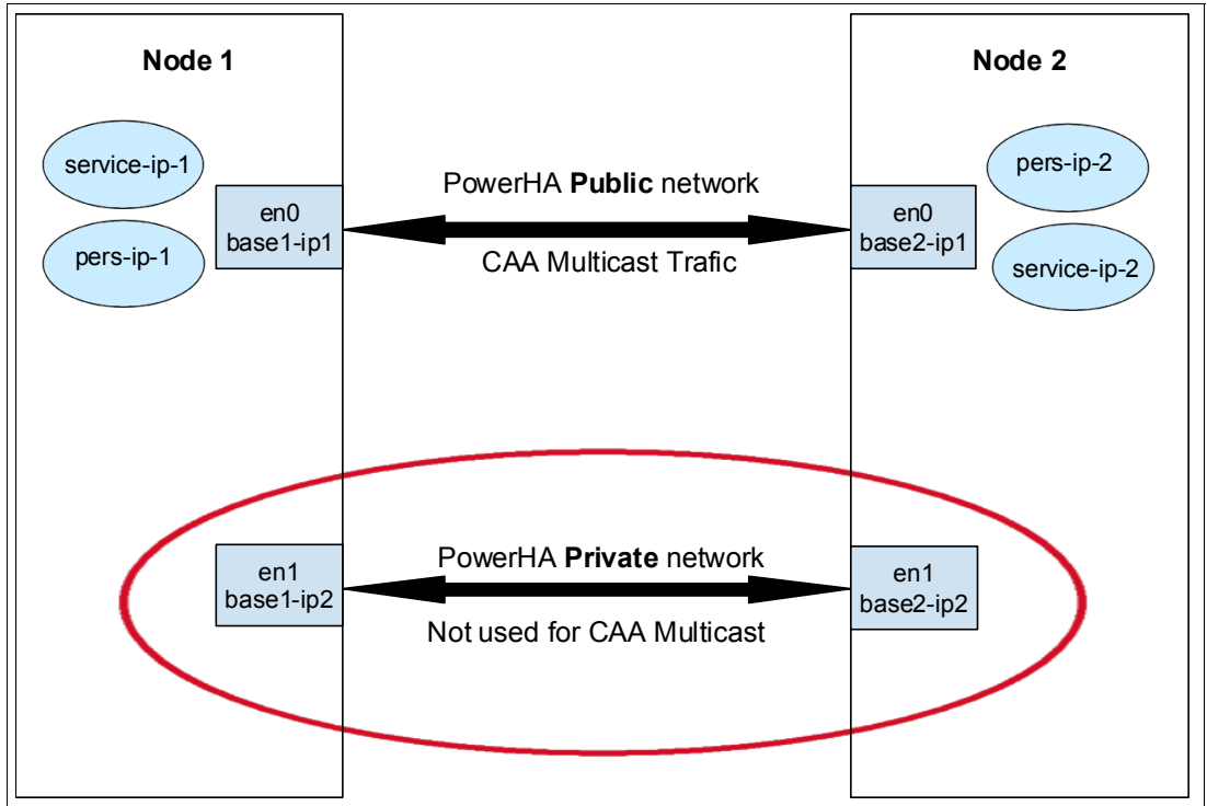
Figure 2-22 Two-node cluster with a public network and a private network
