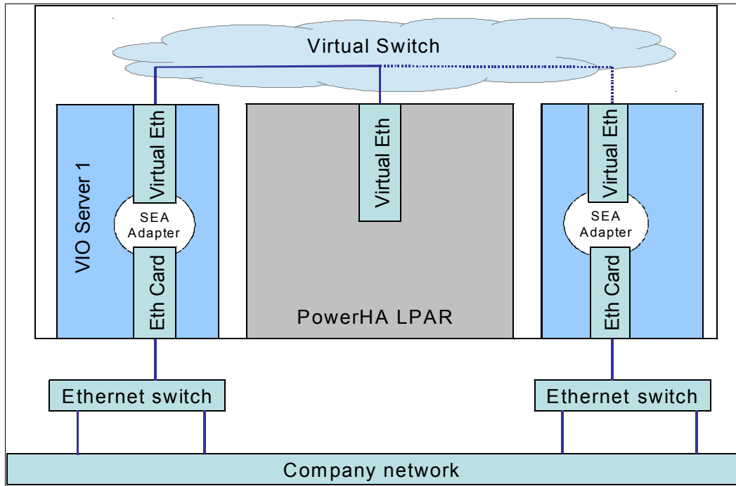
Figure 3-5 Simple SEA failover configuration
