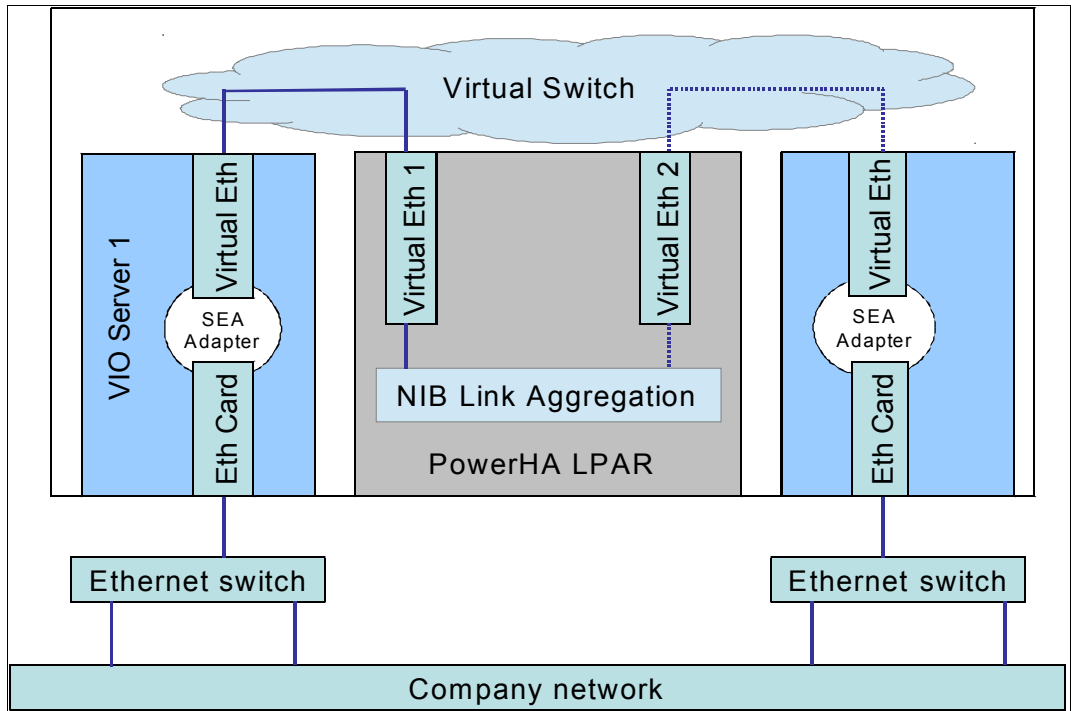
Figure 3-3 Simple NIB configuration
