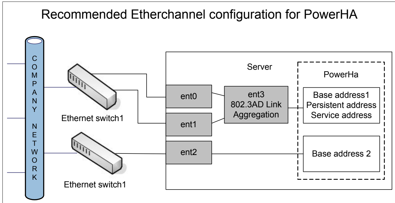
Figure 3-9 Suggested EtherChannel configuration for PowerHA cluster
