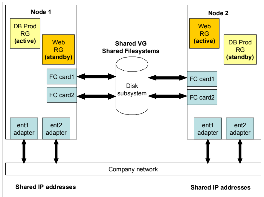
Figure 1-17 Sample mutual takeover cluster configuration
