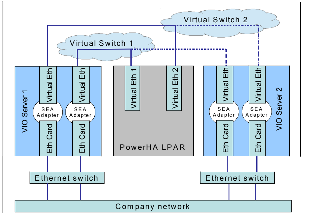
Figure 3-6 SEA failover with two virtual Ethernet adapters on the client side
