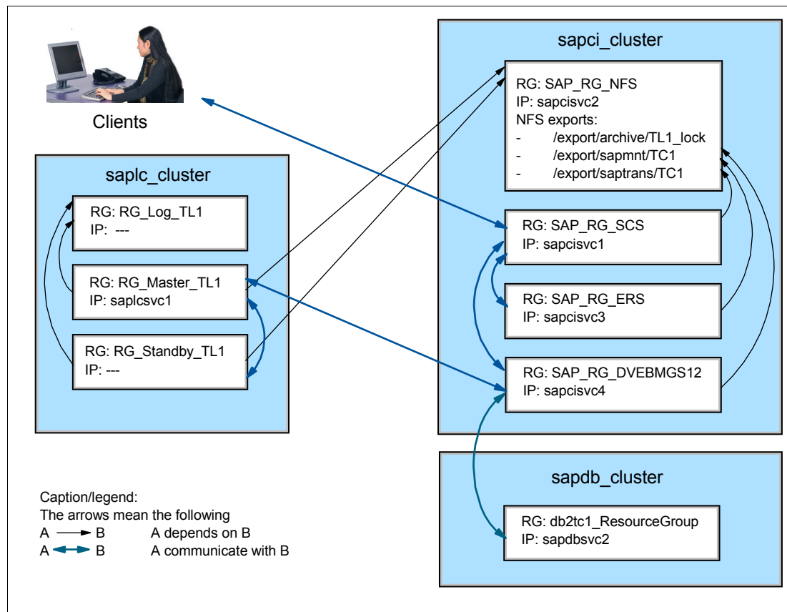
Figure 7-35 Overview of the scenario for a complete three-cluster solution for SAP and liveCache
