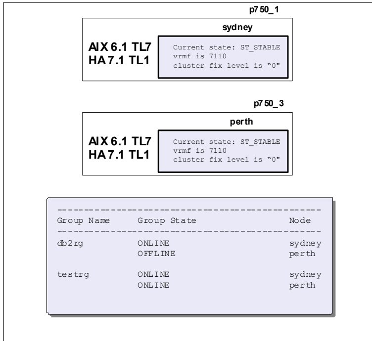
Figure 6-5 Two-node cluster configuration after migration
