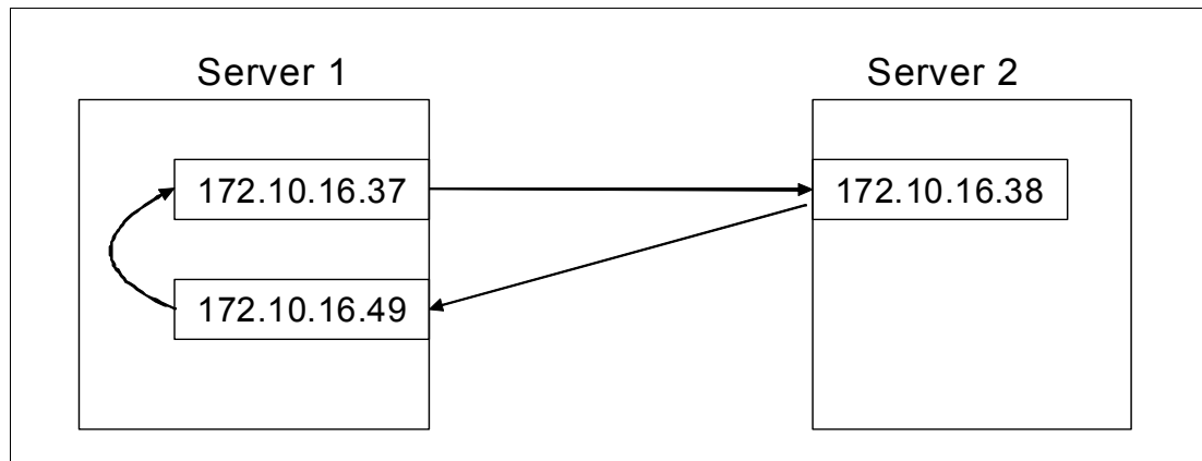
Figure 3-10 AIX server that is connected to same subnet by using two interfaces
