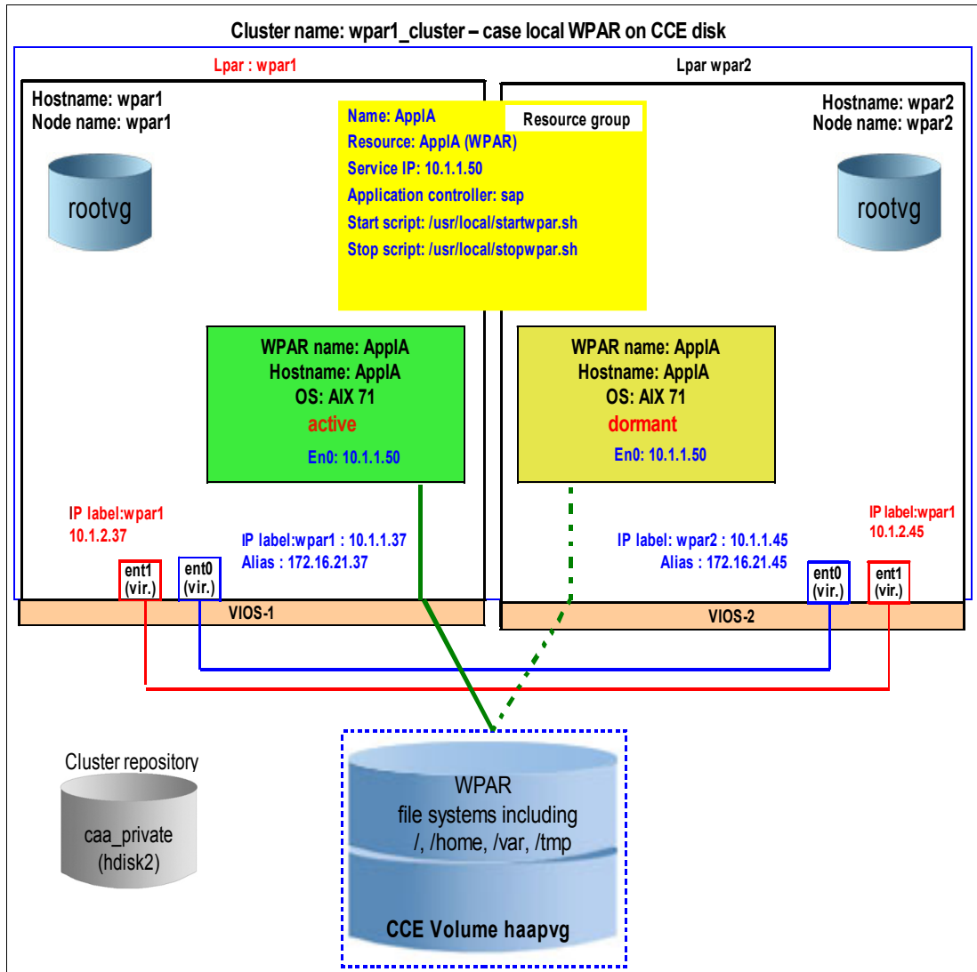
Figure 8-4 Overview of the local (namefs) WPAR environment
