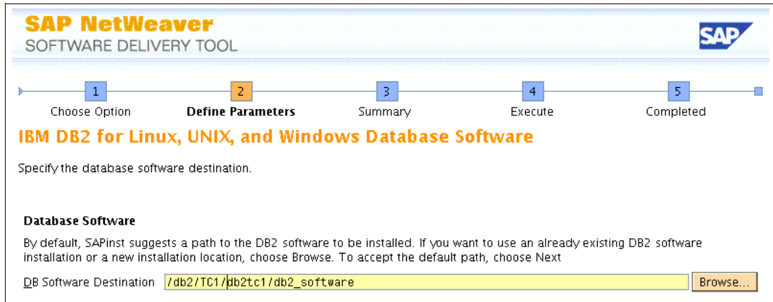
Figure E-16 SAPinst database installation screen capture 6: Database software
