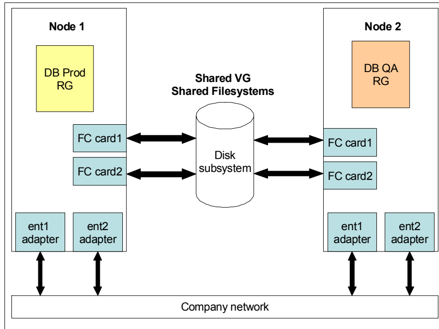
Figure 1-13 A sample cluster environment with location dependency policies
