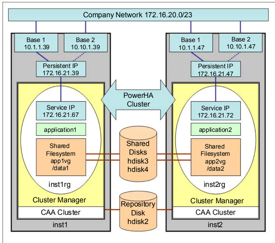
Figure 3-12 Our sample cluster configuration
