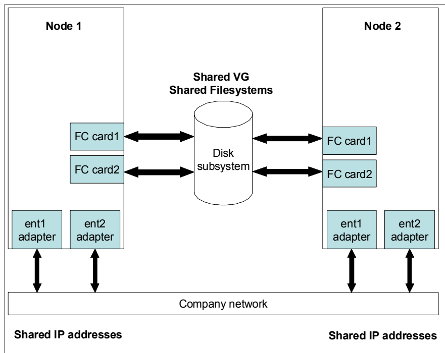
Figure 1-10 A sample cluster scenario with basic shared components
