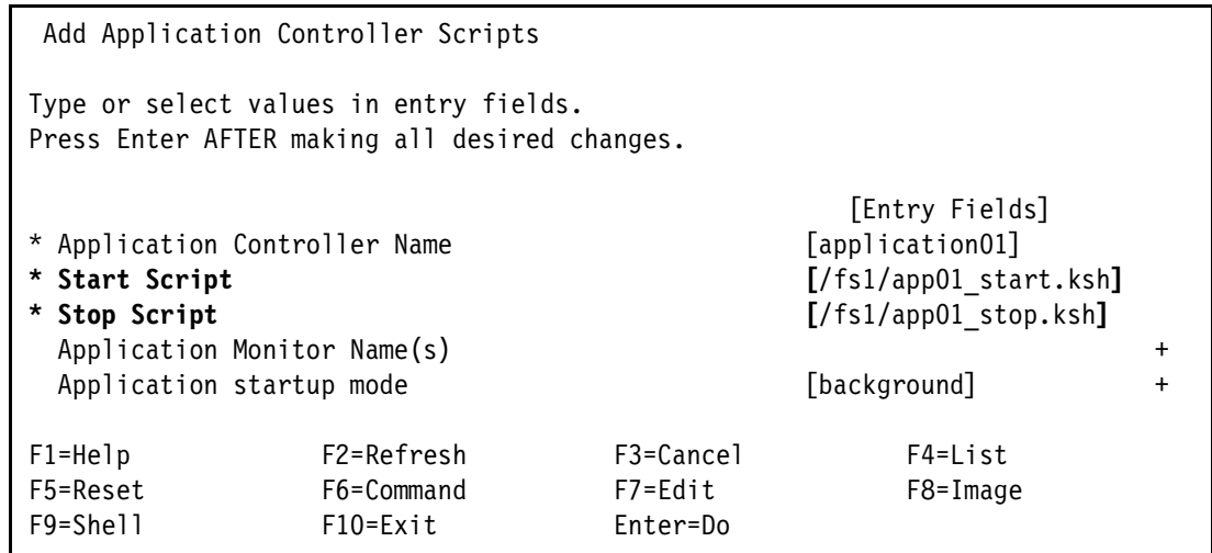
Figure 1-14 Defining Application Controller scripts by using smitty menus
