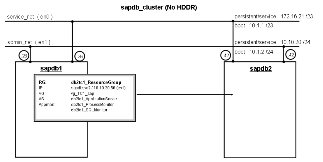
Figure 7-81 Schema overview for sapdb_cluster
