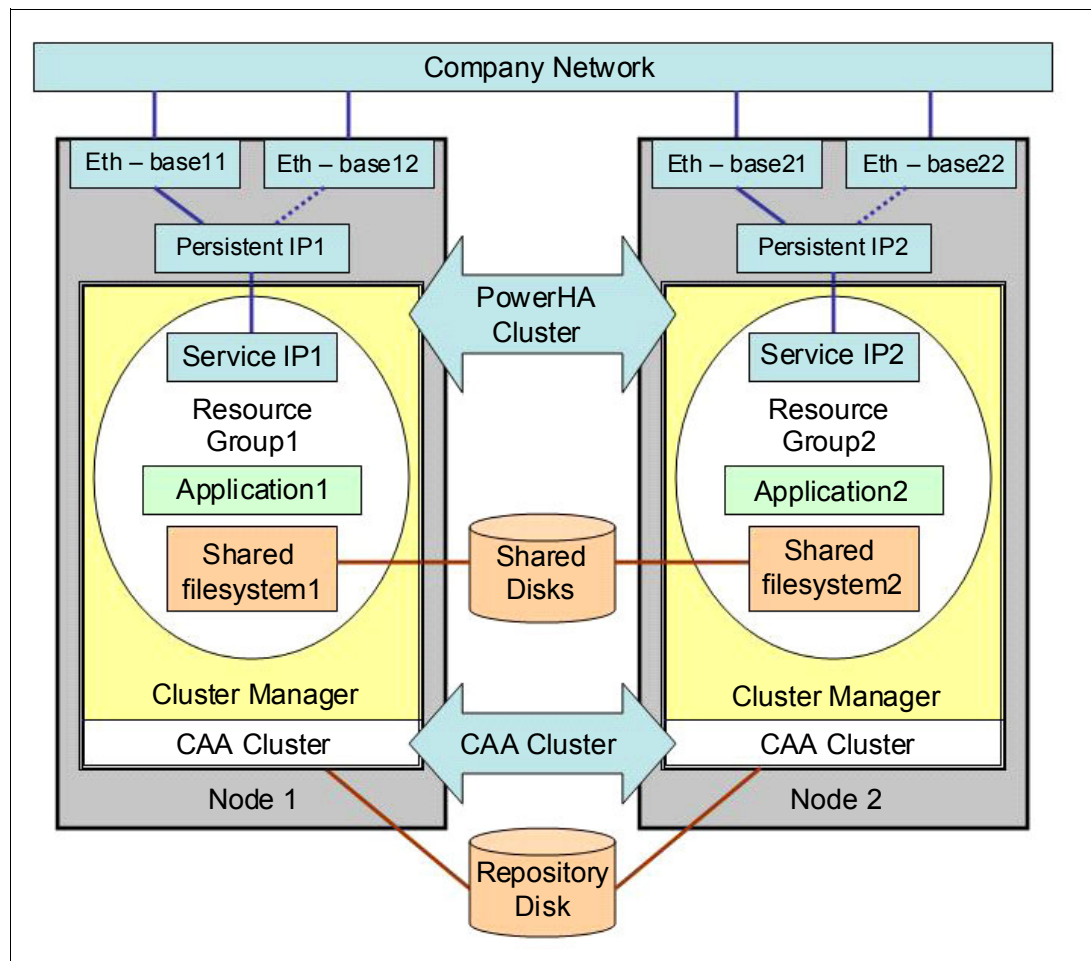
Figure 3-1 Typical PowerHA SystemMirror 7.1.1 cluster
