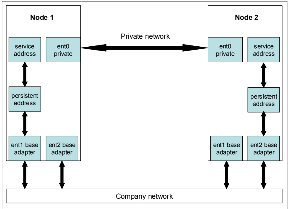
Figure 1-9 Common network configuration in a 2-node cluster environment
