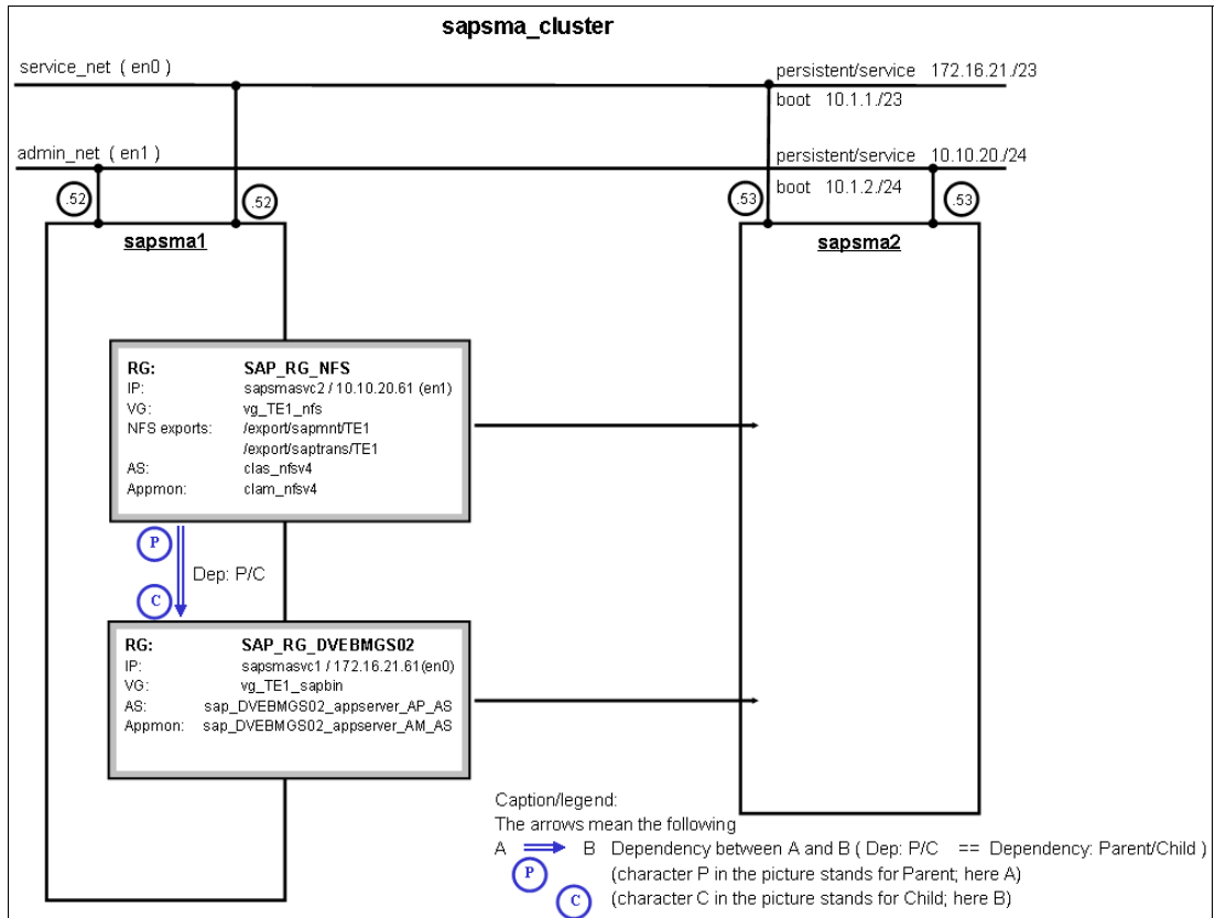
Figure 7-1 Schema overview alternative A for sapsma_cluster
