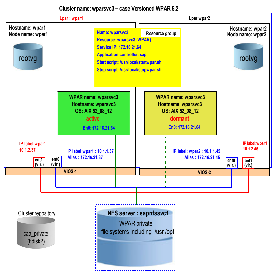
Figure 8-12 Configuration with NFS versioned 5.2 WPAR
