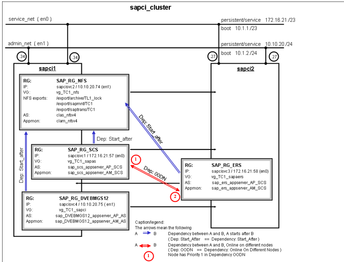
Figure 7-36 Schema overview for sapci_cluster
