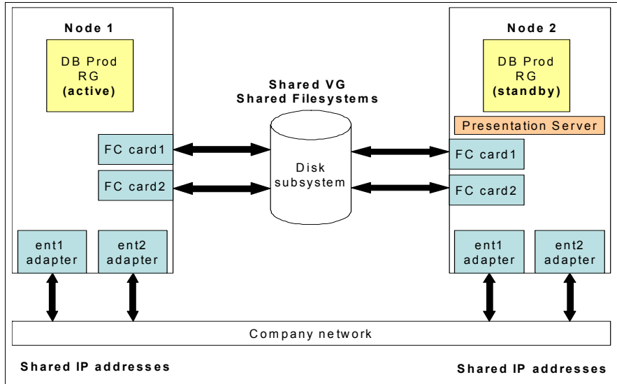
Figure 1-16 Sample one-sided takeover cluster configuration
