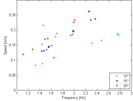
10: Speed of CUTTLEFIN. The asterisks represent the calculated values for the amplitudes \Theta = 10^\circ, 15^\circ and 20^\circ . Calculations using data where gear slippage occurred are displayed as crosses.
