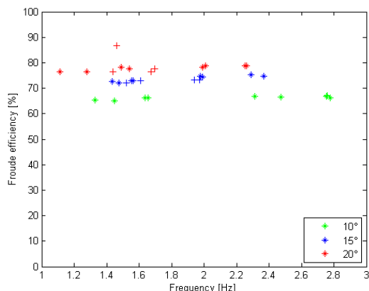
11: Froude efficiency of CUTTLEFIN. The asterisks represent the calculated values for the amplitudes \Theta = 10^\circ, 15^\circ and 20^\circ . Calculations using data where gear slipping occurred are displayed as crosses.
