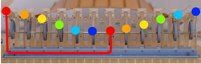
5: Pulley and wire system. The rear ends of each linked pair of rays which are 180^\circ out of phase are marked by circles of the same colour. One wire is highlighted as an example.
