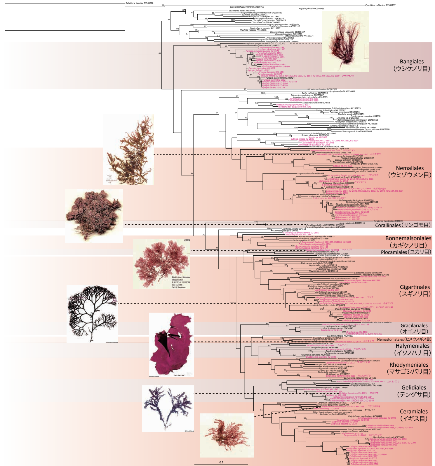
rbcL 遺伝子に基づく分子系統樹 / Molecular phylogenetic tree based on rbcL gene sequence
