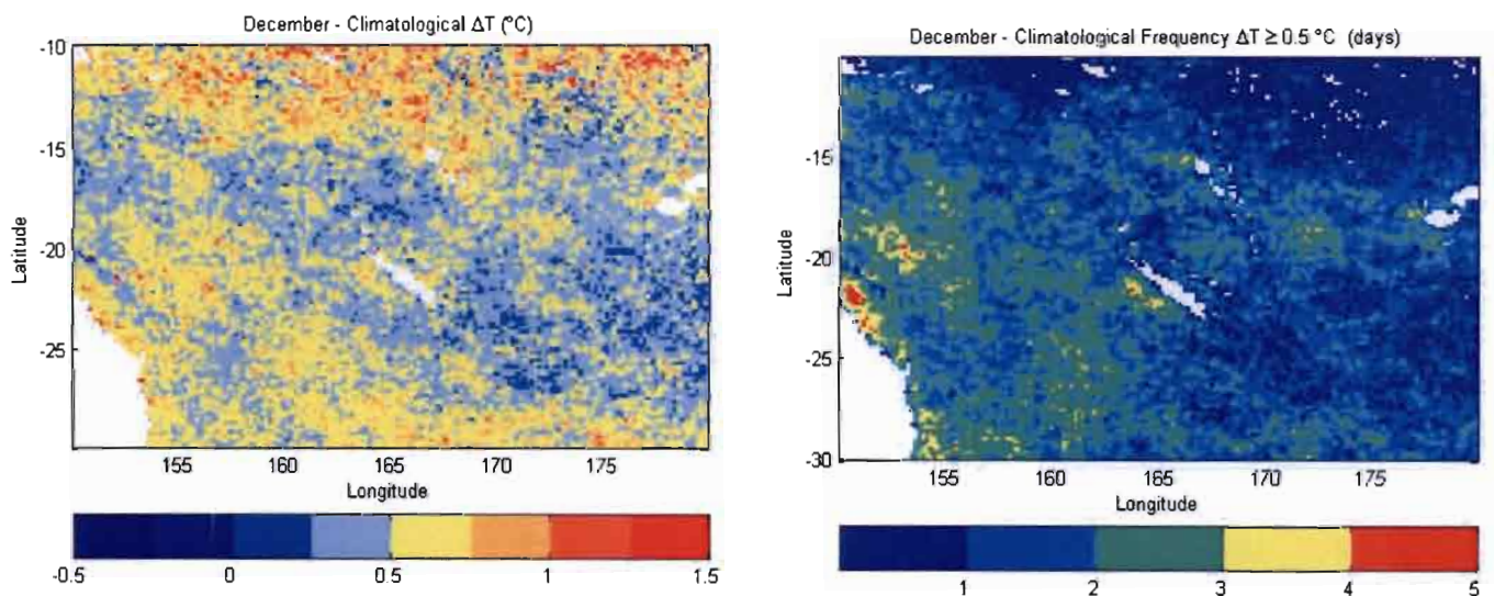
Figure 6. Monthly mean distribution in December of diurnal warming (left) and number of occurrences in days when \Delta T > 0.5^{\circ}\text{C} (right) based on satellite-derived SST (courtesy of Alice Stuart-Menteth).
