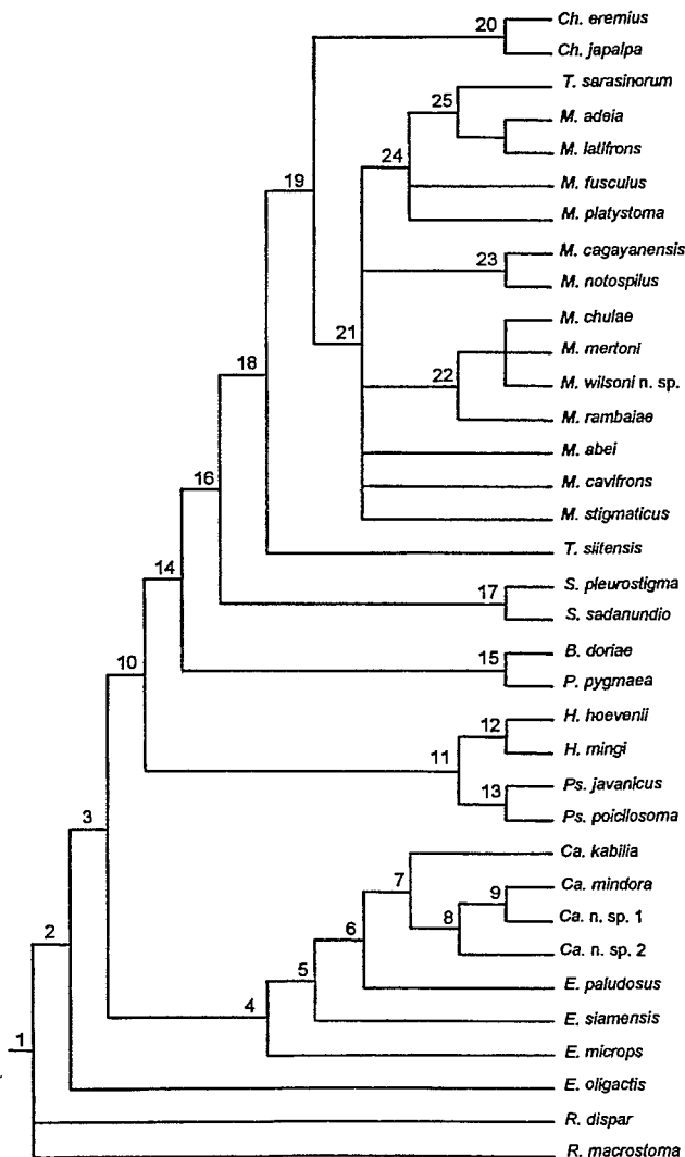
Figure 28 One of 12 equally parsimonious trees comprising the consensus shown in Figure 27; preferred tree on which to base the classification used in this paper.
