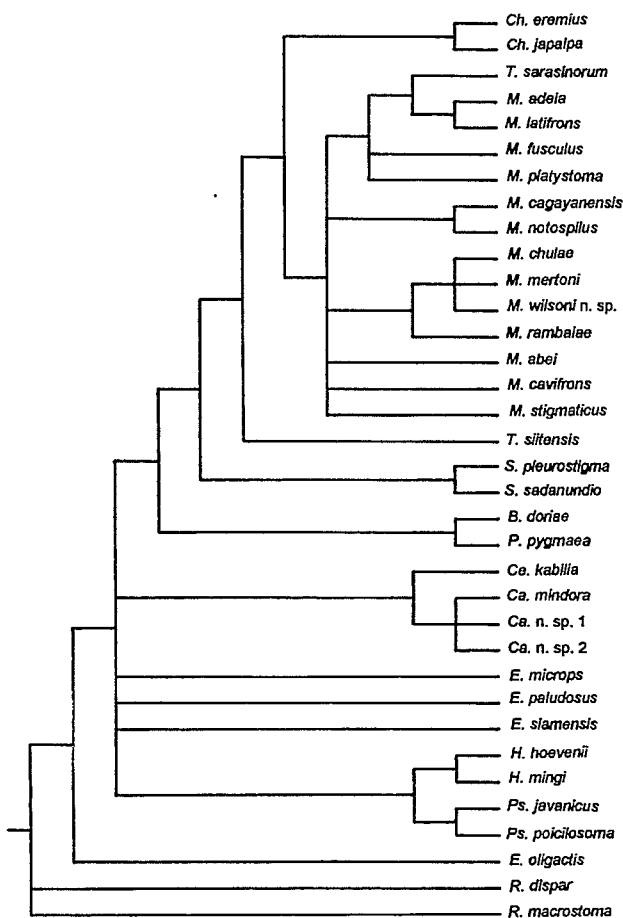
Figure 27 Result of PAUP analysis of reduced set of taxa, with Calamiana n. sp. 2 and Eugnathogobius paludosus added; strict consensus of 12 equally parsimonious trees.
