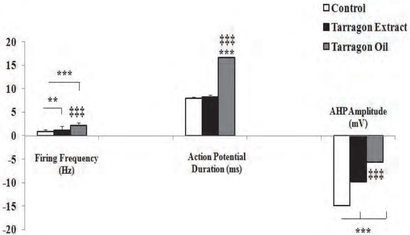
Fig. 3. Electrophysiological consequences of Tarragon application on action potential parameters in F1 neurons. Tarragon essential oil and its extract altered the AP configuration, as the essential oil profoundly increased the firing frequency and AP duration, but decreased the AHP amplitude. Tarragon extract also increased the firing rate and decreased the AHP, but to a lesser extent than did its essential oil. **, ***, significantly differences ( P < 0.01 , P < 0.001 ) from controls and ‡‡‡, significant difference ( p < 0.001 ) from Tarragon extract treated group.
