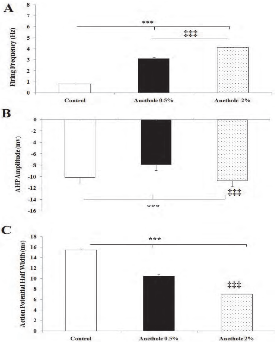
Fig. 7. Effects of anethole treatment on action potential characteristics. Effects of anethole treatment on (A) firing frequency, AHP amplitude (B) and on the AP duration (C). ***, significantly different ( P < 0.001 ) from control; §§§, significant different ( P < 0.001 ) from the 0.5% anethole-treated group.
