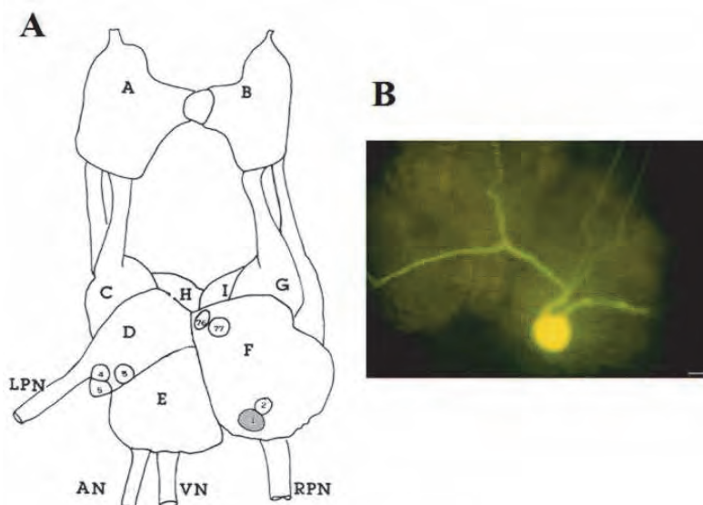
Fig. 1. (A) Scheme redrawn from Kerkut et al. (1975) showing the nine ganglia of the H. aspersa circum-oesophageal ganglia and the four main peripheral nerves. The cell body of F1 (in grey colour) is located in the RPG (A left cerebral ganglion, B right cerebral ganglion, C LPIG, D LPG, E VG, F RPG, G RPIG, H left pedal ganglion, I right pedal ganglion, LPN left pallial nerve, RP right pallial nerve, VN visceral nerve, AN anal nerve). (B) F1 neuron was stained intracellularly by the injection of Lucifer Yellow (5nA hyperpolarizing current pulses of 500ms duration).
