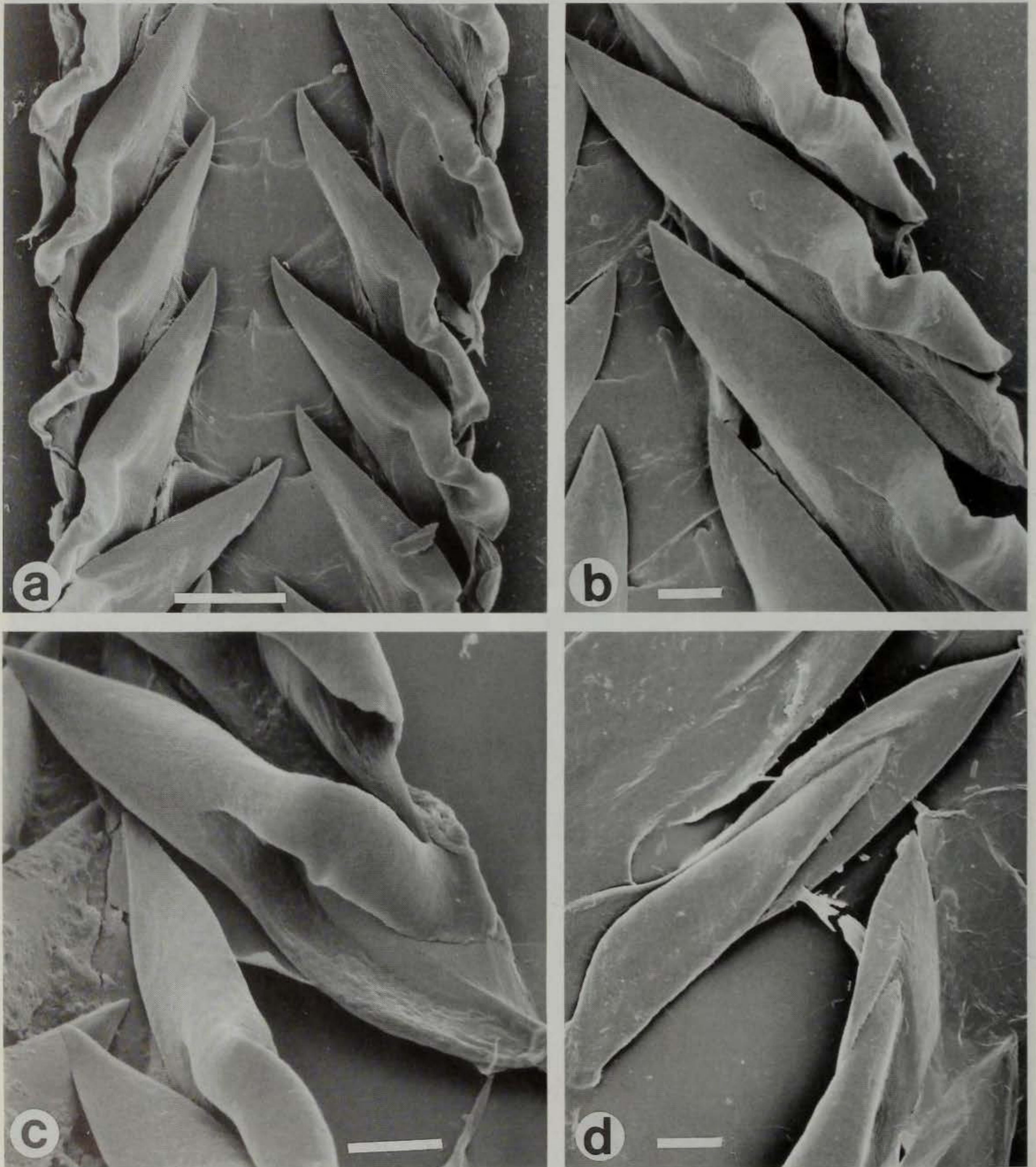
Fig. 19 Wishbone teeth of Turritinae and Cochlespirinae. a. radula of Gemmula deshayesi . Scale bar = 50 \mu\text{m} . b. marginal tooth of Gemmula deshayesi Scale bar = 20 \mu\text{m} . c. marginal tooth of Lophiotoma acuta Scale bar = 10 \mu\text{m} . d. marginal tooth of Antiplanes sanctioannis . Scale bar = 20 \mu\text{m} .
