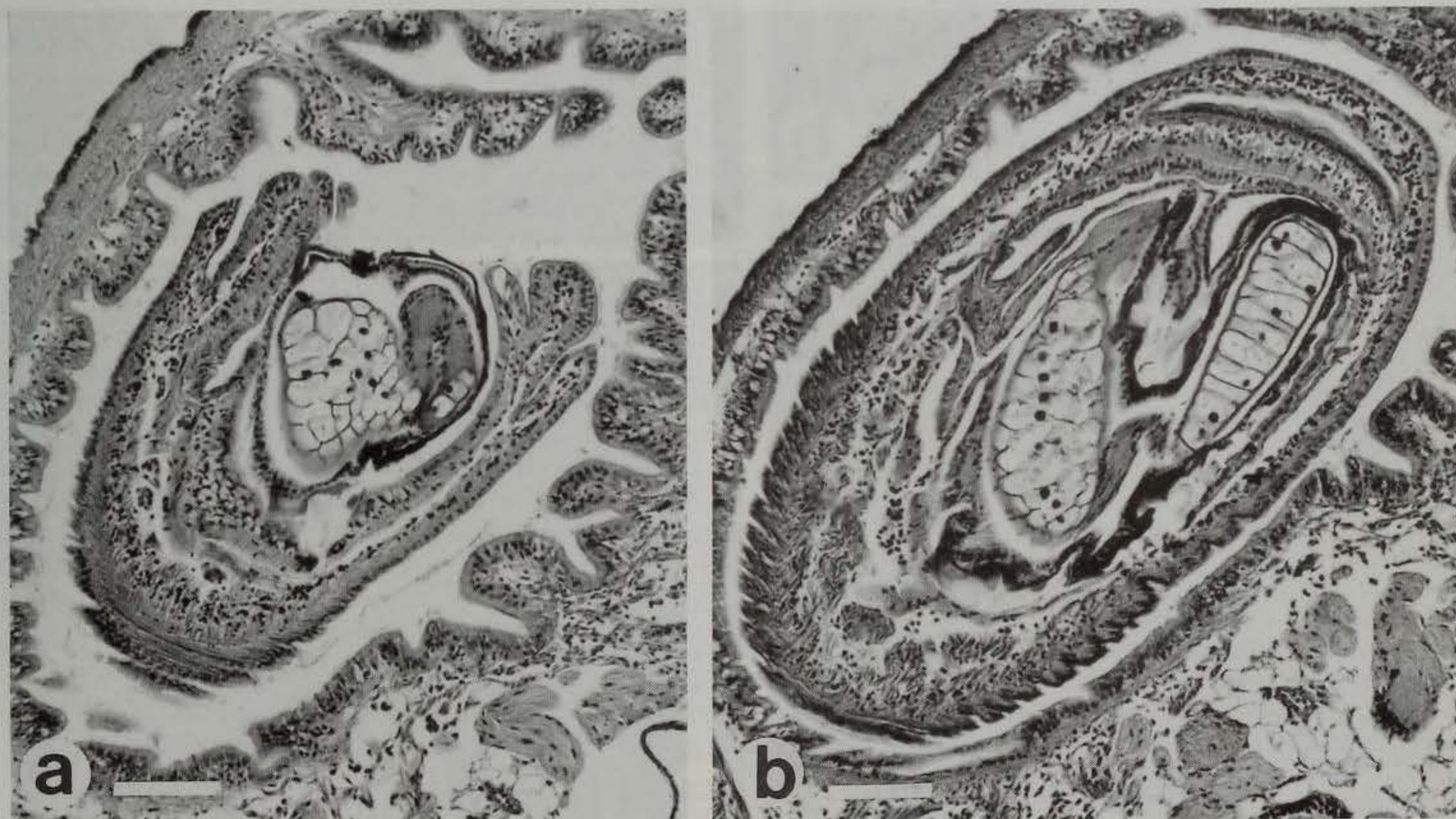
Fig. 13 Strictispira paxillus ; transverse section of the rhynchoel and the proboscis tip. a, mouth with distally-situated radula and virtually no bucal tube. Scale bar = 100 \mu m. b, section of the proboscis slightly to the posterior of (a) showing the two large odontophoral cartilages. Scale bar = 100 \mu m.
