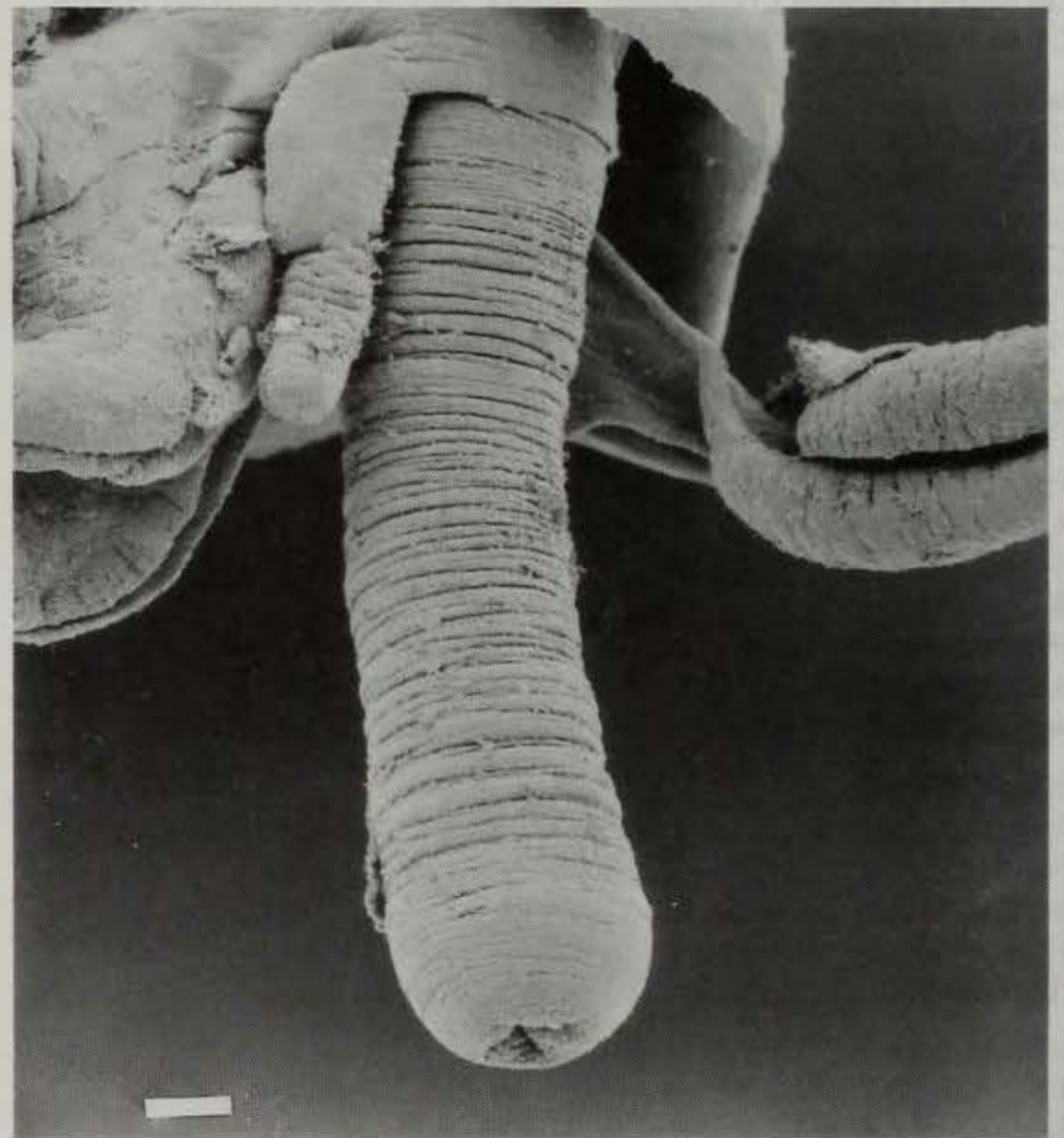
Fig. 3 Hemilienardia malleti ; extended rhynchodeal introvert, forming a pseudoproboscis in a relaxed, critical-point dried specimen. Scale bar = 100 \mu m.
