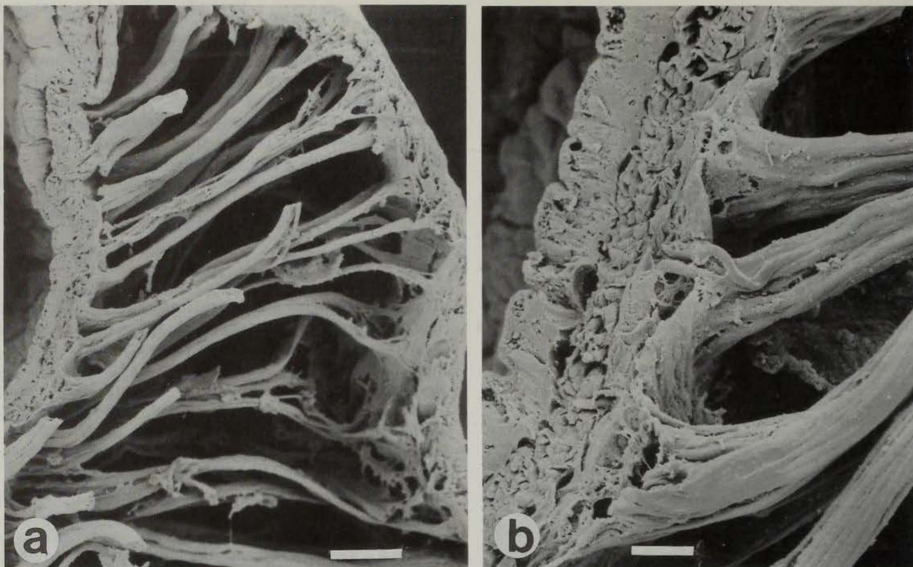
Fig. 5 Duplicaria spectabilis ; relaxed, critical-point dried specimen. A, Section of the rhynchodeal wall showing the transverse muscles joining the inner and outer walls. Scale bar = 100 \mu\text{m} . B, Detail of junction of transverse muscles joining the inner wall of the rhynchodaeum. Scale bar = 20 \mu\text{m} .
