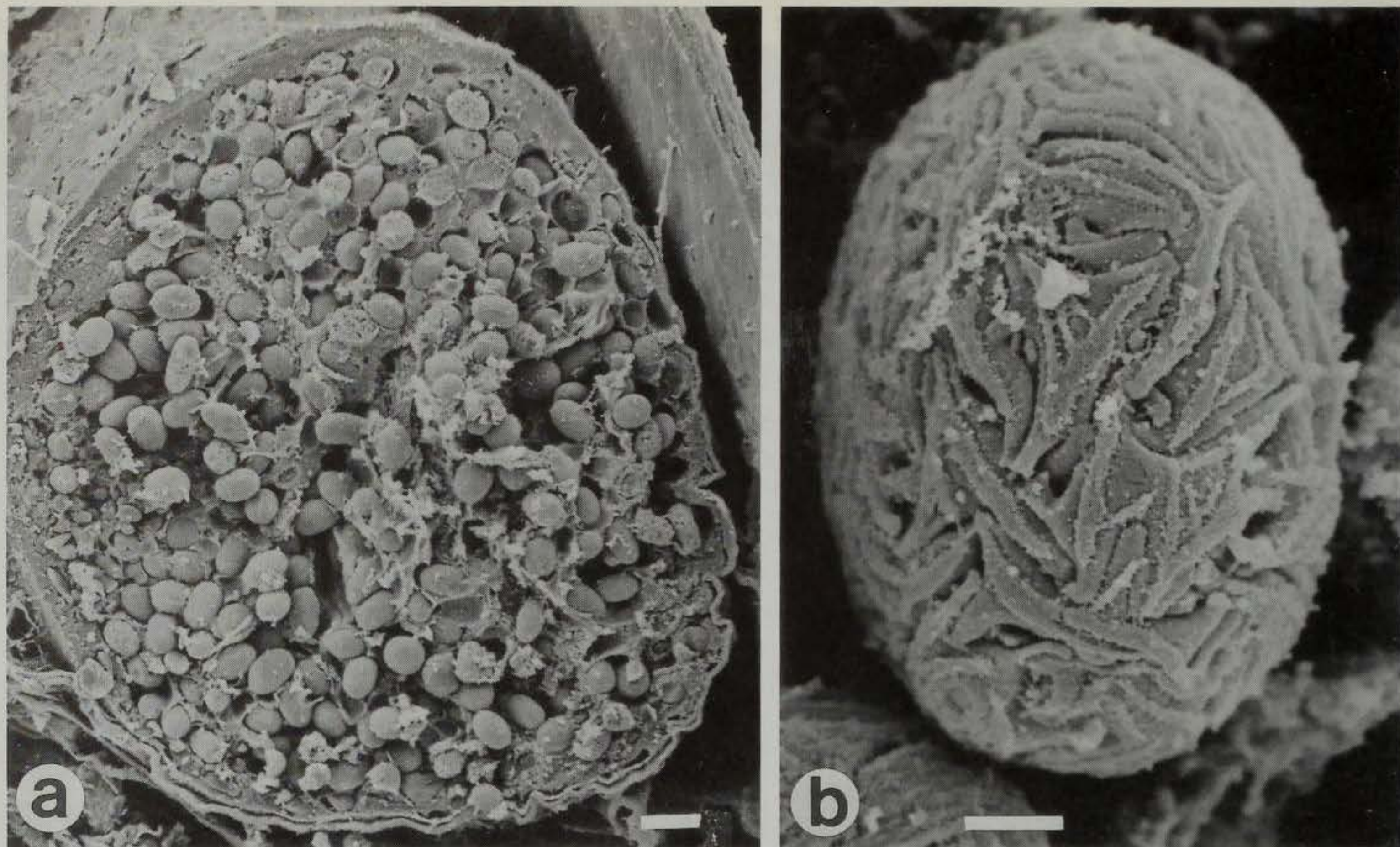
Fig. 24 Venom gland of Clavus sp. Guam. a. section through critical-point dried venom gland showing venom granules. Scale bar = 10 \mu\text{m} . b. enlargement of single venom granule. Scale bar = 1 \mu\text{m} .
