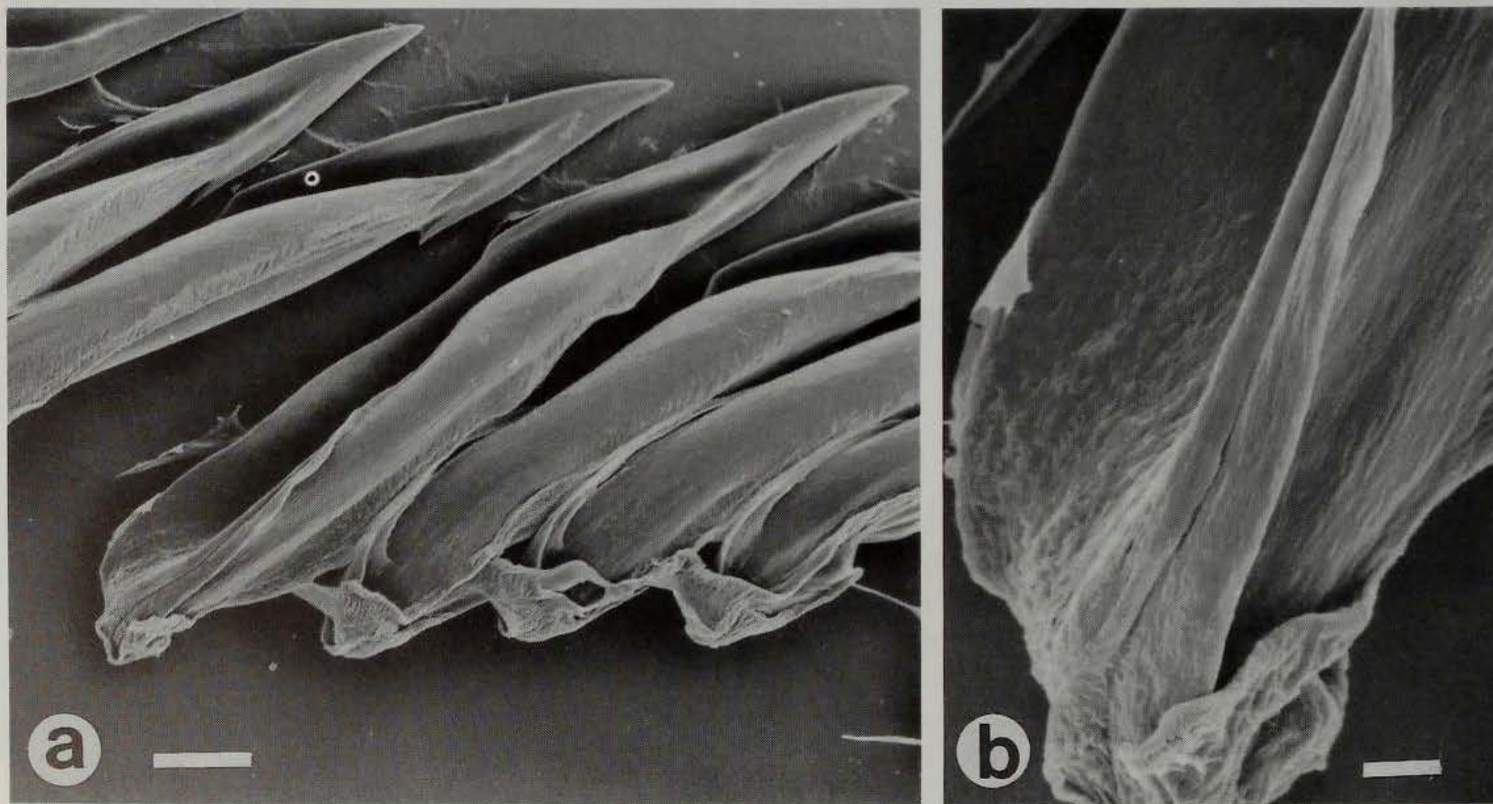
Fig. 21. Enrolled teeth of Pilsbryspira nympha . a. several adjacent marginal teeth. Scale bar = 25 \mu\text{m} . b. detail of base of tooth showing double structure (arrow) suggesting that tooth may be formed by the enrolling of wishbone teeth. Scale bar = 5 \mu\text{m} .
