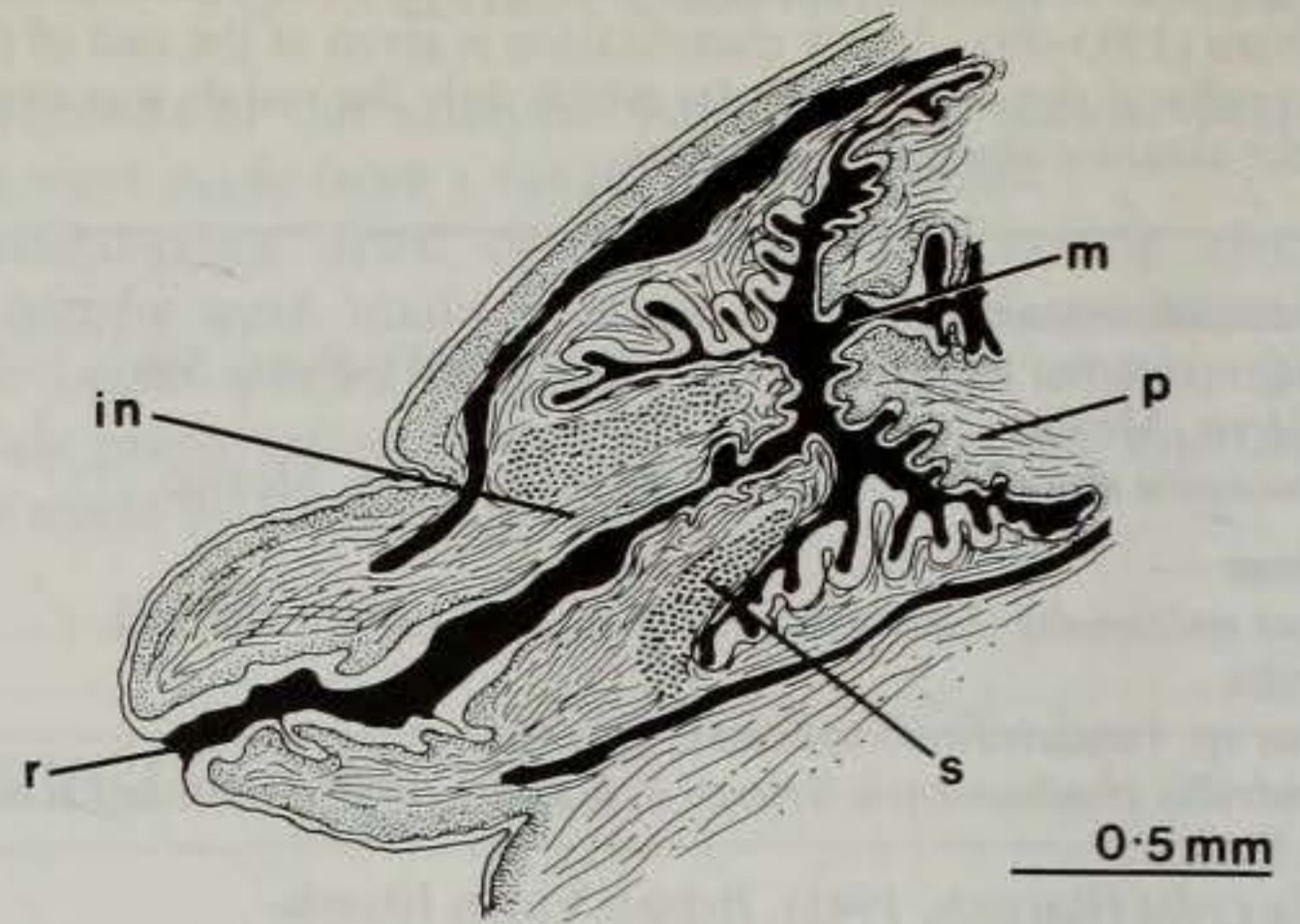
Fig. 2 Ophiidermella inermis ; longitudinal section of the anterior rhynchodeum showing the posteriorly-situated, rhynchostomal sphincter located on an introvert-like structure. Abbreviations: in, introvert; m, mouth; p, proboscis; r, rhynchostome; s, sphincter.
