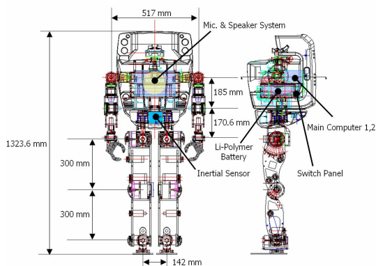
Fig. 3 The design of Albert HUBO
