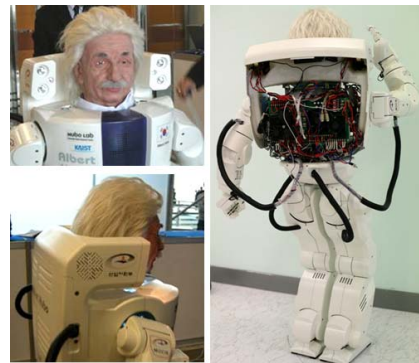
Fig. 8 The backpack of Albert HUBO
