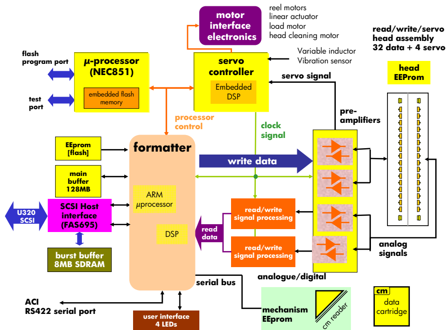
Figure 7. HP StorageWorks Ultrium 960 block diagram
