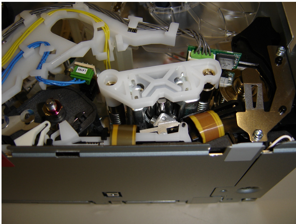
Figure 5. HP StorageWorks Ultrium 960 actuator assembly
