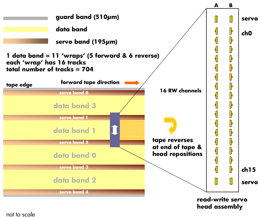
Figure 4. Ultrium 3 format format details
