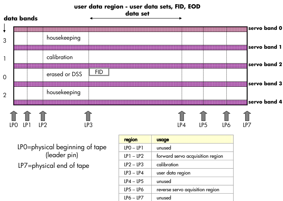
Figure 3. Ultrium format tape layout
