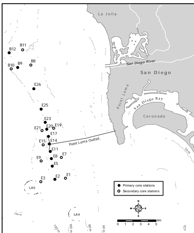
Figure 5.1 Benthic station locations sampled for the Point Loma Ocean Outfall Monitoring Program.
